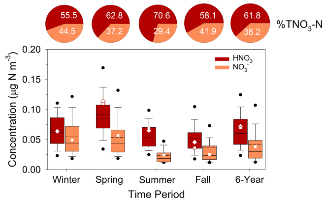
Figure 6. Summary of CASTNET HNO 3 and NO 3 - concentrations (as N) from 2015–2020 during winter, spring, summer, and fall. Solid and dashed lines inside the box represent the median and mean, respectively. The top and bottom of the box represent 75th and 25th percentiles. Whiskers represent 10th and 90th percentiles, and dots represent 5th and 95th percentiles. “6-year” represents the statistics for the entire 6-year period. Squares and diamonds represent the seasonal and annual mean CASTNET (HNO 3 and NO 3 - ) and continuous DD-CL HNO 3 for the August 2015–August 2016 modeling period, respectively. Pie charts represent the average percent contribution of HNO 3 and NO 3 - to total NO 3 - (HNO 3 + NO 3 - ) expressed as nitrogen.
