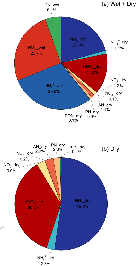
Figure 11. Speciated annual total (wet and dry) (a) and dry (b) deposition showing the percent contribution of individual components. TS11
