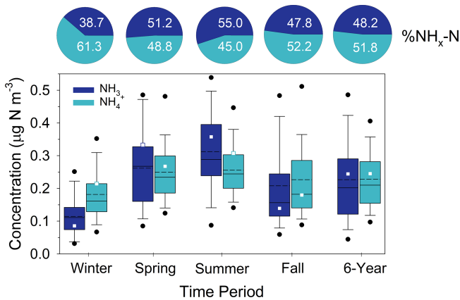
Figure 7. Summary of AMoN \text{NH}_3 and CASTNET \text{NH}_4^+ concentrations (as N) from 2015–2020 during winter, spring, summer, and fall. Solid and dashed lines inside the box represent the median and mean, respectively. The top and bottom of the box represent 75th and 25th percentiles. Whiskers represent 10th and 90th percentiles, and dots represent 5th and 95th percentiles. “6-year” represents the statistics for the entire 6-year period. Squares represent the seasonal and annual mean concentration for the August 2015–August 2016 modeling period. Pie charts represent the average percent contribution of \text{NH}_3 and \text{NH}_4^+ to total \text{NH}_x ( \text{NH}_3 + \text{NH}_4^+ ) expressed as nitrogen. AMoN concentrations were adjusted by subtracting the mean travel blank for the 6-year period.
