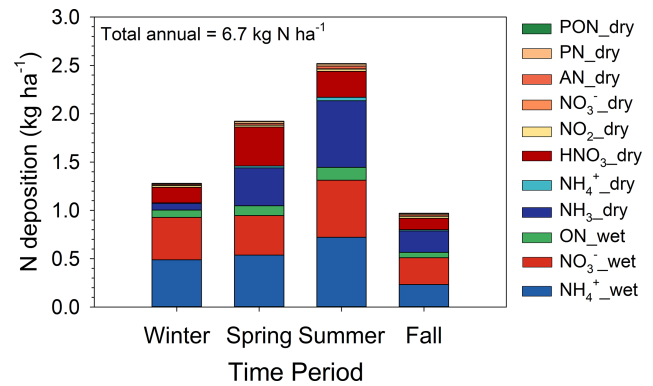
Figure 12. Seasonal speciated deposition budget. \text{N}_r species are listed in the legend as defined in the text, along with indication of the deposition pathway (dry or wet).
