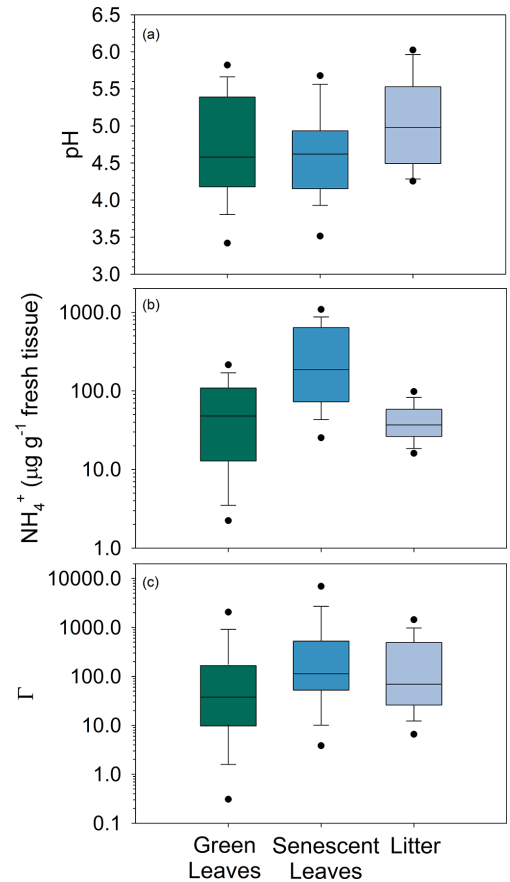
Figure 9. Box plots of pH (a), \text{NH}_4^+ (b) concentration ( \mu\text{g g}^{-1} fresh tissue), and equivalent emission potential ( \Gamma ) (c) in tissue of green leaves, senescent leaves, and litter on the forest floor. The solid line inside the box represents the median. The top and bottom of the box represent 75th and 25th percentiles. Whiskers represent 10th and 90th percentiles, and dots represent 5th and 95th percentiles.
