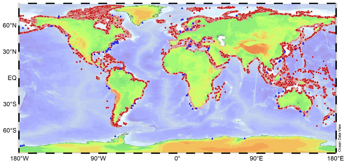
1090 Figure 2. Global distribution of reported FSGD (red circles) and OFG (blue triangles) sites. Location data from FSGD and OFG from Luijendijk et al. (2020) and Micallef et al. (2021), respectively.
