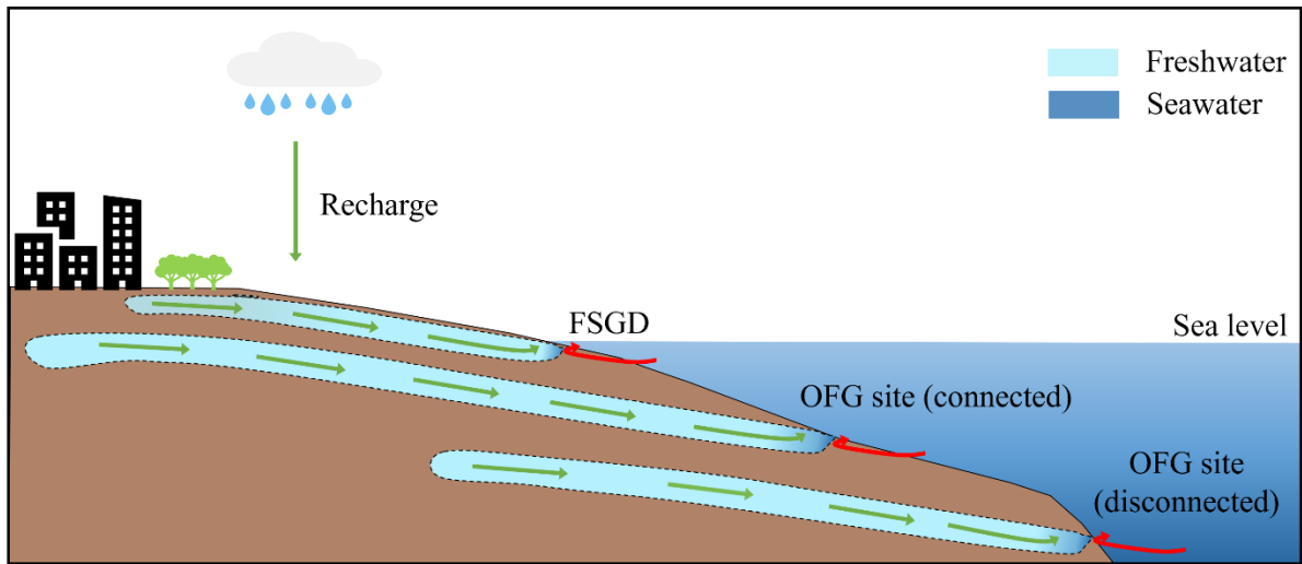
1080 Figure 1. Schematic representation of known pathways for the transport of and storage of fresh and freshened groundwater between terrestrial and marine realms. Areas surrounded by dashed lines indicate groundwater reservoirs, whereas arrows represent freshwater (green) and seawater (red) fluxes. Based on Bratton et al. (2010) and Weymer et al. (2020).
