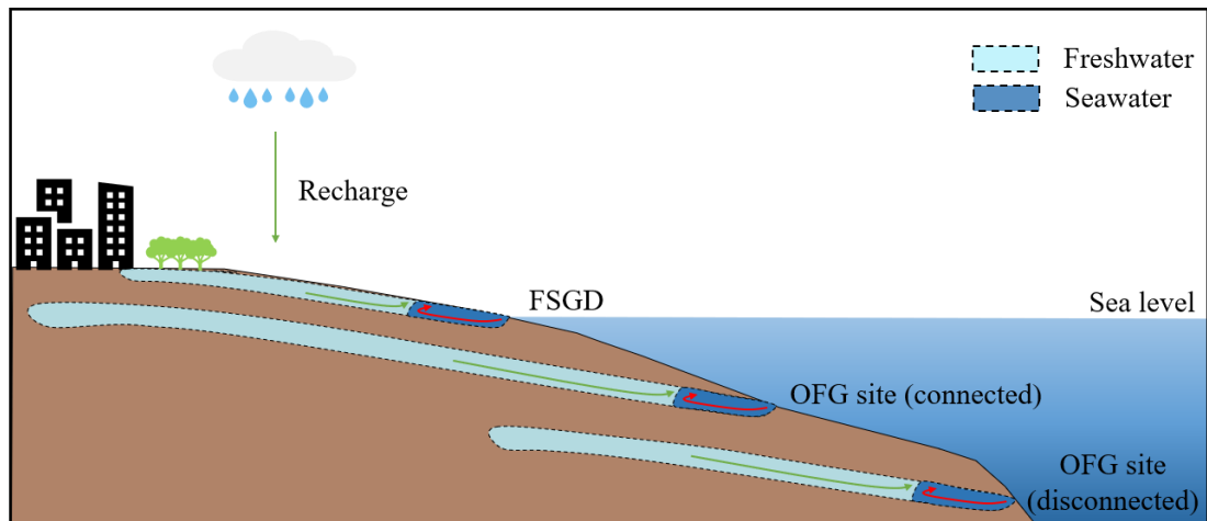
Figure 1. Schematic representation of known pathways for the transport of and storage of fresh and freshened groundwater between terrestrial and marine realms. Areas surrounded by dashed lines indicate groundwater reservoirs, whereas arrows represent freshwater (green) and seawater (red) fluxes. Based on Bratton et al. (2010) and Weymer et al. (2020).
