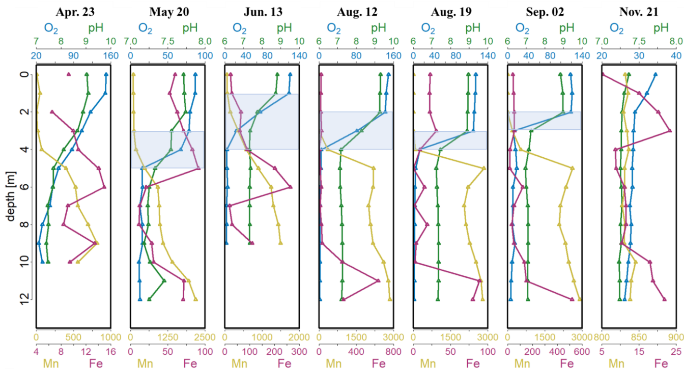
595 Fig. 1. Depth profiles of O 2 saturation (%), pH and concentrations of dissolved Mn [ \mu\text{g L}^{-1} ] and Fe [ \mu\text{g L}^{-1} ] in the Lake Ölper water column from April to November 2019. The depth of the sharp decrease in O 2 concentration and start of Mn reduction (RTZ) are shown in each panel (shaded light blue). Note that each column has an individual scale to better illustrate changes with depth. Depth profiles with the same scale in all columns are shown in the supplements (Fig. S1).
