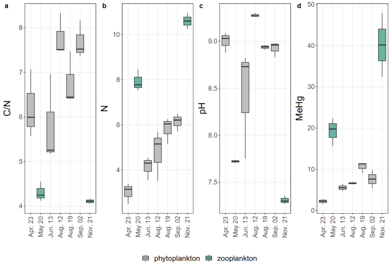
Fig. 4. C/N ratio (a), N concentration [%] (b), pH (c) and MeHg concentration [ng g -1 ] (d) of the individual sampling days from the upper two oxic metres (0; 1; 2 m). Colours indicate differences in plankton dominance; green symbolizes higher amounts of zooplankton; grey symbolizes higher amounts of phytoplankton. The relative dominance of zooplankton was estimated from visible inspection and from pH only.
