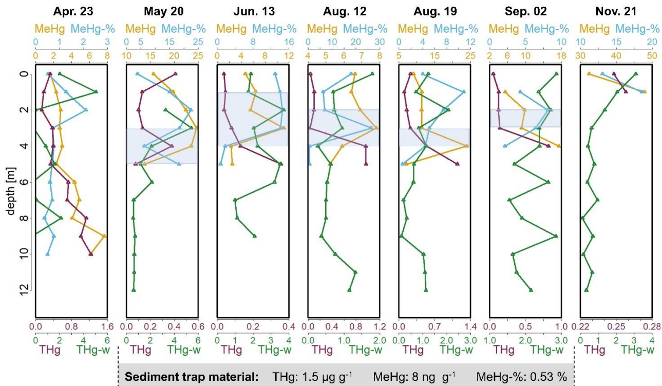
Fig. 3. Depth profiles of MeHg [ \text{ng g}^{-1} ] concentrations, percentage of MeHg [%] of THg (MeHg-%), THg concentrations in 610 seston [ \mu\text{g g}^{-1} ] and dissolved THg [ \text{ng L}^{-1} ] in the water column (THg-w) of lake Ölper from April to November 2019. The depth of the sharp decrease in \text{O}_2 concentration and start of Mn reduction (RTZ) are shown in each panel (shaded light blue). Concentrations of THg [ \mu\text{g g}^{-1} ], MeHg [ \text{ng g}^{-1} ], MeHg-% [%] of the sediment trap material collected over the 141 days between May 6 th and September 24 th are given in the grey box below. Note that each column has an individual scale to better illustrate changes with depth. Depth profiles with the same scale in all columns are shown in the supplements (Fig. S5).
