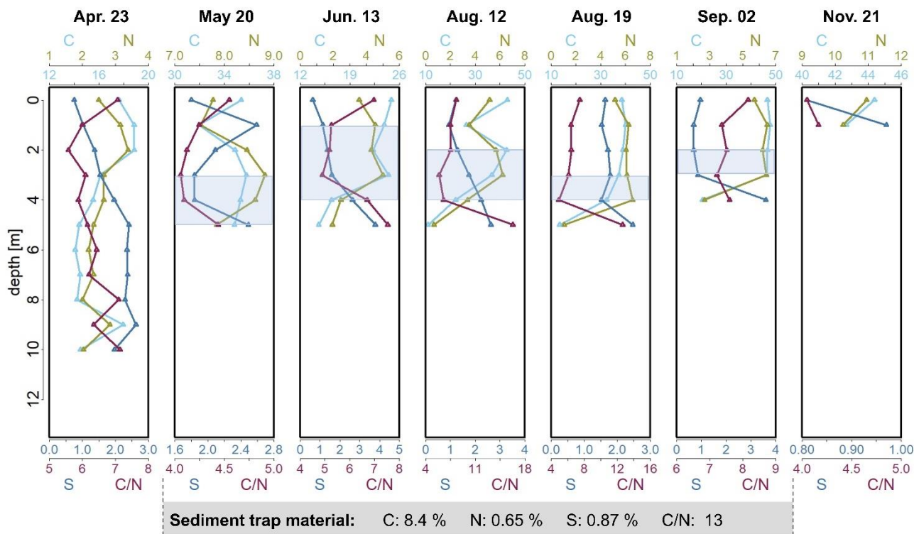
600 Fig. 2. Depth profiles of C [%], N [%], S [%] concentrations and calculated C/N ratio in the seston in Lake Ölper from April 605 to November 2019. The depth of the sharp decrease in O 2 concentration and start of Mn reduction (RTZ) are shown in each panel (shaded light blue). Concentrations of C [%], N [%], S [%] and the C/N ratio of the sediment trap material collected during the 141 days between May 6 th and September 24 th are given in the grey box below. Note that each column has an individual scale to better illustrate changes with depth. Depth profiles with the same scale in all columns are shown in the supplements (Fig. S4).
