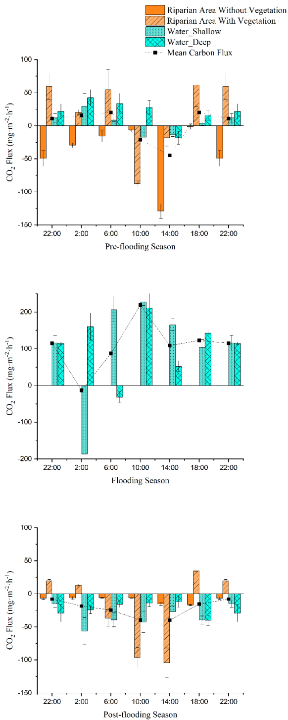
Figure 1. CO 2 fluxes in riparian area (with vegetation and without vegetation) and fluvial area (shallow area with vegetation and deep area without vegetation ) during pre-flooding season (measured in April), flooding season (August), and post-flooding season (October).
