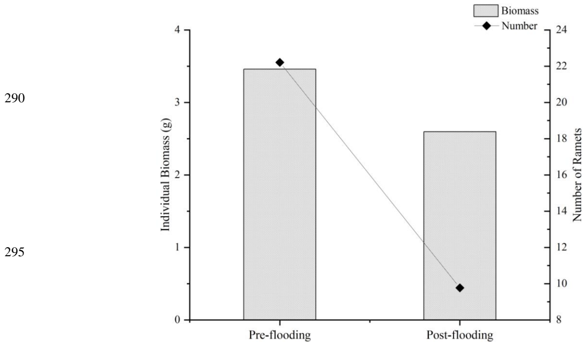
Figure 3. The comparison of the individual biomass and number of Chrysopogon aciculatus before and after flooding in the controlled experiment.
