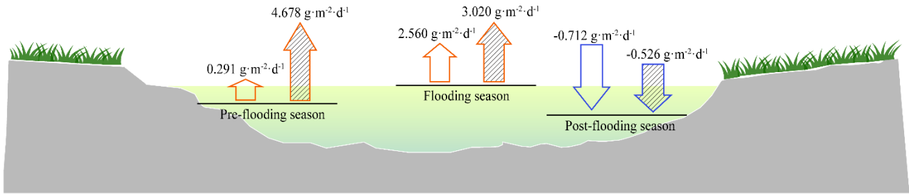
270 Figure 2. All-day CO 2 flux with low water-level in pre-flooding season, high water-level during flooding season, and resumed 275 low water-level in post-flooding season in 2014 (Blank) and 2016 (Dashed). The upward arrow refers to carbon emission, and the downward arrow refers to carbon uptake.
