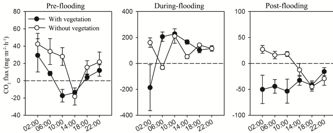
Appendix Figure A2: Effects of time (measuring times in one day) on CO 2 flux in the water-air surface of the water sections fluvial area with vegetation (shallow-water, filled) and without vegetation (deep-water, blank) in the three sampling stages. Mean ± 1 SE is given.
