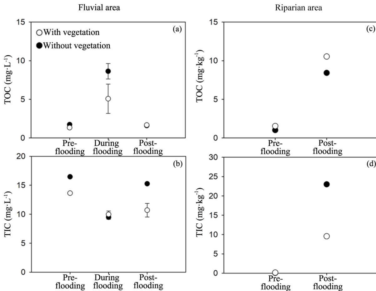
Figure 4. Total organic carbon (TOC) and total inorganic carbon (TIC) in the study area. The aquatic (fluvial area) and riparian habitats (riparian area) include study areas with vegetation and without vegetation. TOC and TIC were also measured in different sampling stages. The ANOVA results for habitats, season, and interaction effects are given, including the degree of freedom ( df ), F , and P values in Appendix Table A4.
