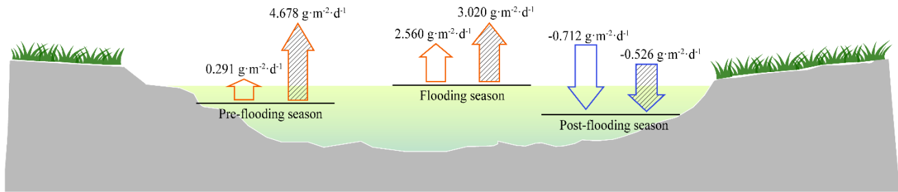
270 Figure 2. All-day CO 2 flux with low water-level in pre-flooding season, high water-level during flooding season, and resumed low water-level in post-flooding season in 2014 (Blank) and 2016 (Dashed). The upward arrow refers to carbon emission, and the downward arrow refers to carbon uptake.
