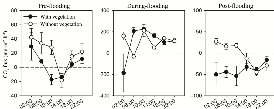
Appendix Figure A2: Effects of time (measuring times in one day) on CO 2 flux in the water-air surface of the fluvial area with vegetation (shallow-water, filled) and without vegetation (deep-water, blank) in the three sampling stages. Mean ± 1 SE is given.
