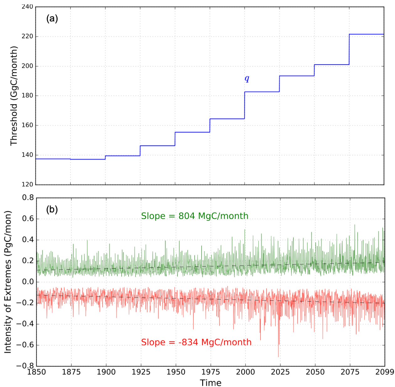
Figure 1. (a) The 5 th percentile threshold, q , of NBP anomalies. The negative extremes in NBP are those NBP anomalies that are < -q and positive extremes are > q . (b) The intensity of positive and negative extremes in NBP in CESM2 are represent by green and red color, respectively. The rate of increase of positive and negative extremes in NBP are 804 and -834 MgC per month, respectively.
