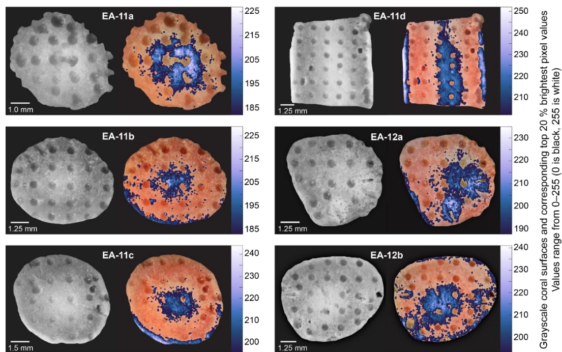
505 Figure 10: Compilation of grayscale images and corresponding brightest pixels (highest 20%) over each coral slice. The colors correspond to the grayscale pixel value (higher on the scale bar denotes a whiter pixel). The sample holes surrounded by at least ~75% of bright pixels were used to calculate representative \delta^{18}\text{O} values for each slice for temperature calibration (Table S3 in the Supplement ).
