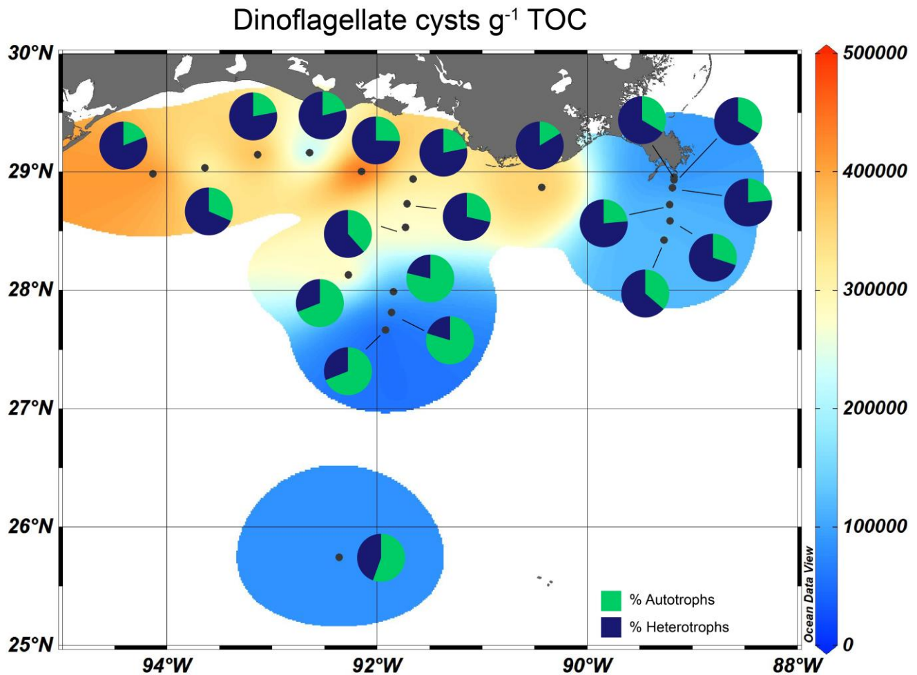
375 Figure 8: Isosurface plots of the TOC-normalized dinocyst concentration in GoM surface sediments overlain by pie-charts showing the relative contribution of autotroph and heterotroph species.
