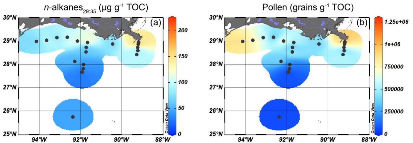
Figure 7: Isosurface plots for the input of higher plant-derived OM in surface sediments of the GoM, based on OC-normalized concentrations of a) long-chain ( C_{29} - C_{35} ) n -alkanes and b) pollen grains (excluding Pinus pollen).
