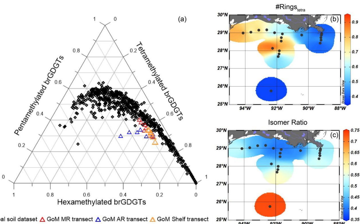
450 Figure 10: Assessment of the sources of brGDGTs in GoM surface sediments. A) Ternary diagram showing the tetra-, penta-, and hexamethylated brGDGTs in GoM surface sediments plotted together with the global soil and peat dataset (Dearing Crampton-Flood et al., 2019), b) the \#rings_{tetra} , an indicator for marine produced brGDGTs and c) the Isomer Ratio (IR), indicative for fluvially produced brGDGTs.
