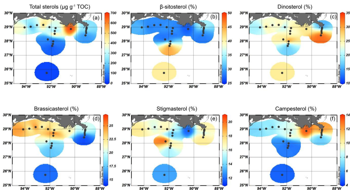
360 Fig. 6: Isosurface plots showing a) the total sterol concentration and b-f) relative abundances of the individual sterols; b) \beta -sitosterol, c) dinosterol, d) brassicasterol, e) stigmasterol, f) campesterol.
