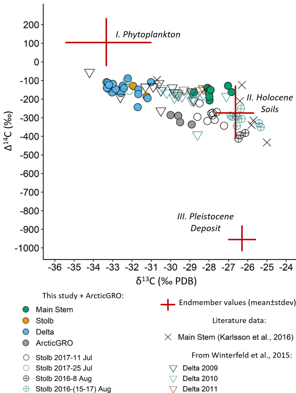
480 Figure 4. The origin of the POC in the Lena River and the Lena Delta. Endmember values (red crosses) were combined after Galimov et al., 2006, Wild et al., 2019, and Winterfeld et al., 2015; additional previously published data were added from Winterfeld et al., 2015 and Karlsson et al., 2016.
