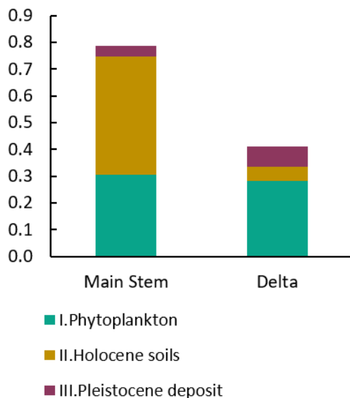
565 Figure 5. Contributions of different OM sources to the POC measured in the Lena River main stem and the Lena Delta along the transect in 2019.
