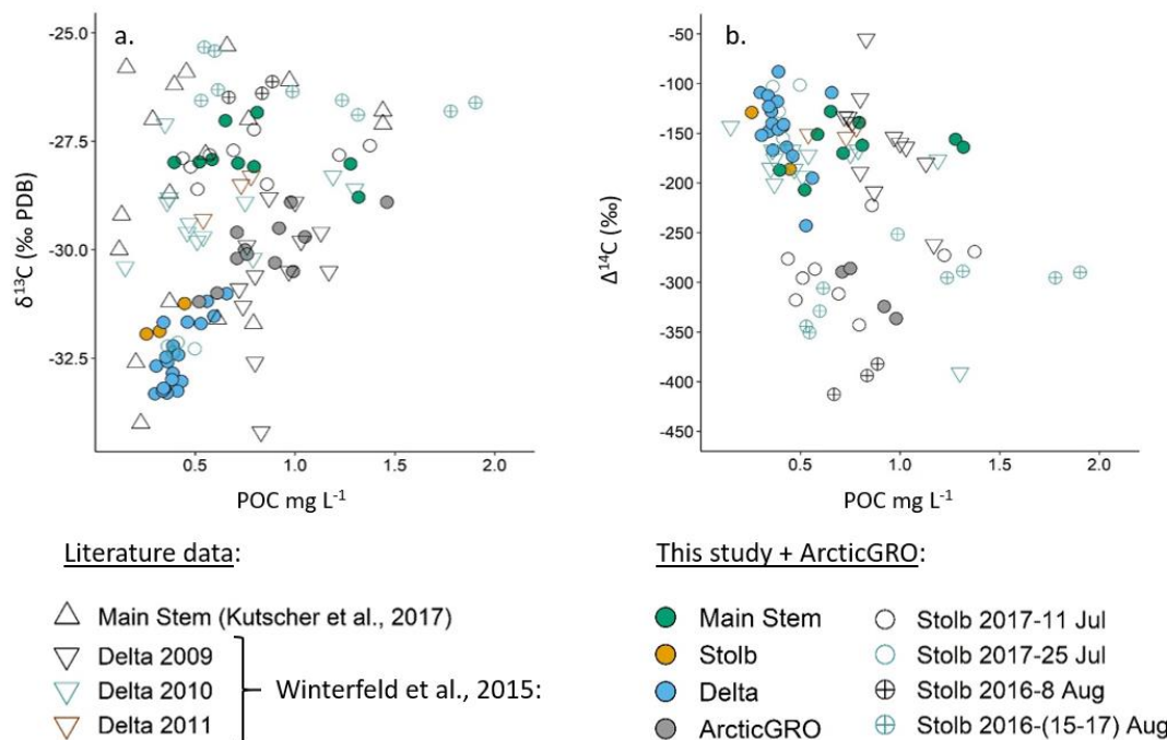
370 Figure 3. Stable and radiocarbon isotopic values and POC concentration for the Lena Delta and the Lena River main stem. Values were taken from this study and from the literature (Kutscher et al., 2017 and Winterfeld et al., 2015).
