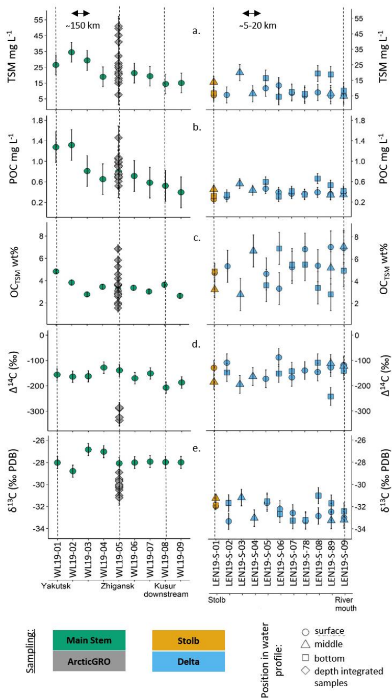
225 Figure 2. Distribution of studied parameters along the transect in the Lena main stem, the Lena Delta, and for the ArcticGRO dataset (mean ±stdev): a. TSM mg L -1 ; b. POC, mg L -1 ; c) OC TSM , wt%; d) Δ 14 C of POC, ‰; e) δ 13 C of POC, ‰.
