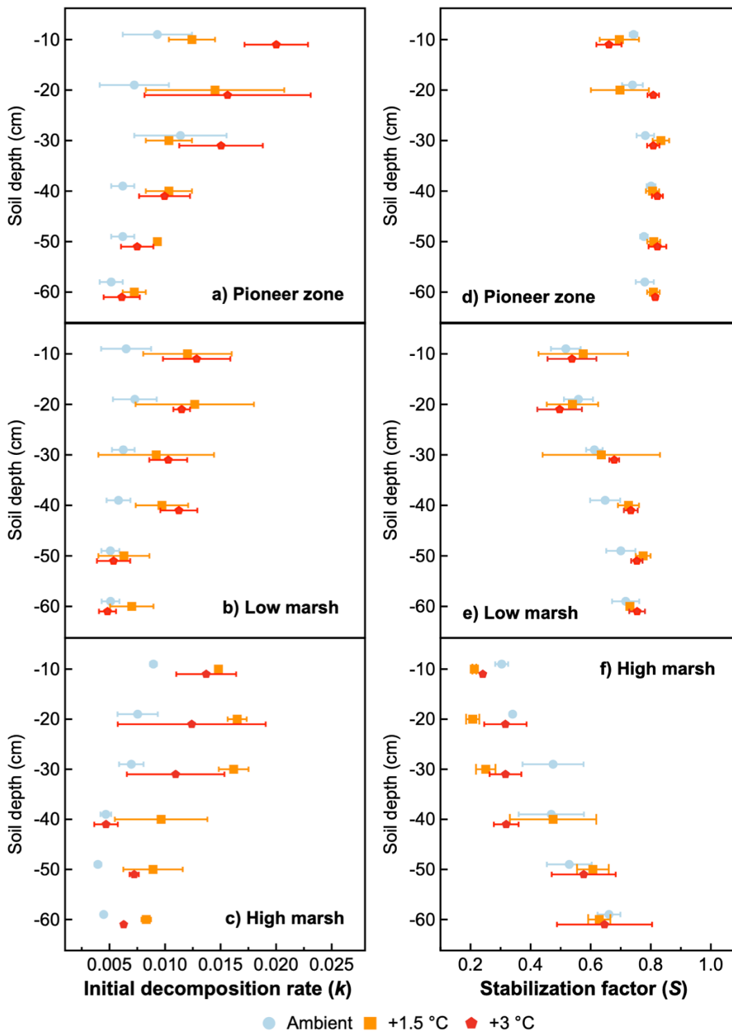
Figure 3 The initial decomposition rate ( k ) (a, b, c) and stabilization factor ( S ) (d, e, f) at different soil depths of the pioneer zone, low marsh, and high marsh zones under three temperature treatments (ambient, +1.5 °C and +3 °C) in year 1 (2018). Values are means \pm SE ( n=3 ). k describes the labile fraction which is decomposed in the deployed material, and S presents the part of the labile fraction that did not decompose which stabilized in the soil.
