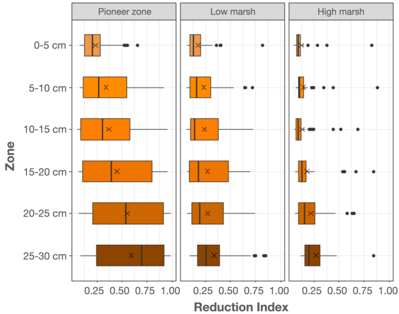
215 Figure 6. Soil reduction in relation to marsh zone and soil depth at the Hamburger Hallig salt marsh site. Shown are median- (black bar) and mean values (black x). The box is giving the interquartile range, and potential outliers are depicted as black points. Data are based on n = 6 observations per zone, deployed over four consecutive deployment campaigns (July-October). The reduction index (0-1) describes the fraction of FeCl 3 paint that is removed from the PVC stick after four weeks of deployment in the field.
