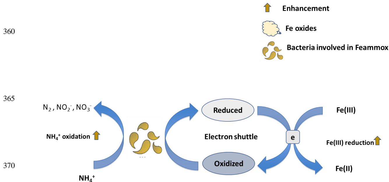
Figure 4. Electron shuttles enhance Fe reduction and NH_4^+ oxidation (Feammox) rates.
