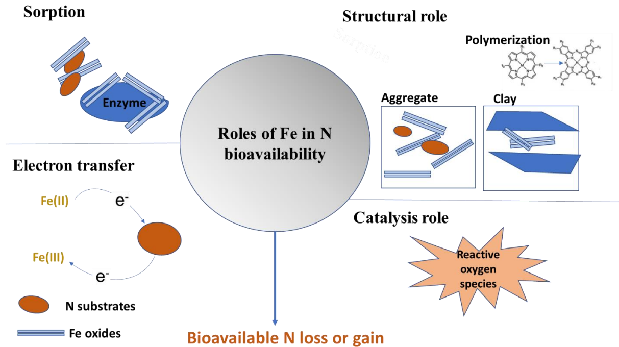
Figure 2: Roles of Fe in N bioavailability.
