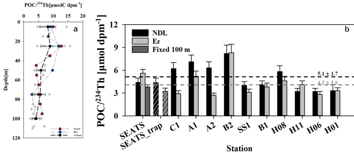
330 Figure 7: Water-column POC/ ^{234}Th ratios from bottle filtration, with the averages (black dots with dashed line) at each sampling depth plotted against depth (a). Also shown are the bottle- and trap-derived POC/ ^{234}Th ratios (bar with white stripes) at the bottom of the NDL (black), base of the euphotic zone (light grey), and fixed 100 m depth (dark grey) (b). Generally, the variability of POC/ ^{234}Th decreased as depth increased and converged around 4.2 \pm 1.6 \mu mol dpm^{-1} at the Ez base. No significant variability (within 2-fold) was found between POC/ ^{234}Th ratios derived from bottle and trap samples accessed at the same sampling depths at station SEATS.
