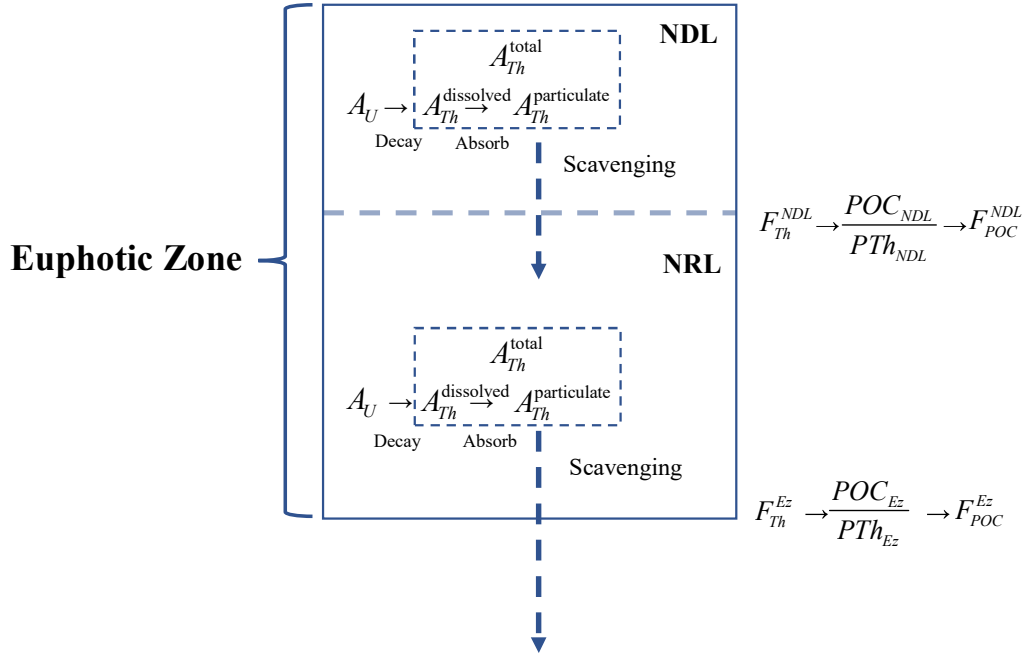
180 Figure 2: Schematic of the ^{234}\text{Th} model under the two-layer nutrient structure. The terms are defined in Eq. (2)-(4) and Eq. (7)-(9).
