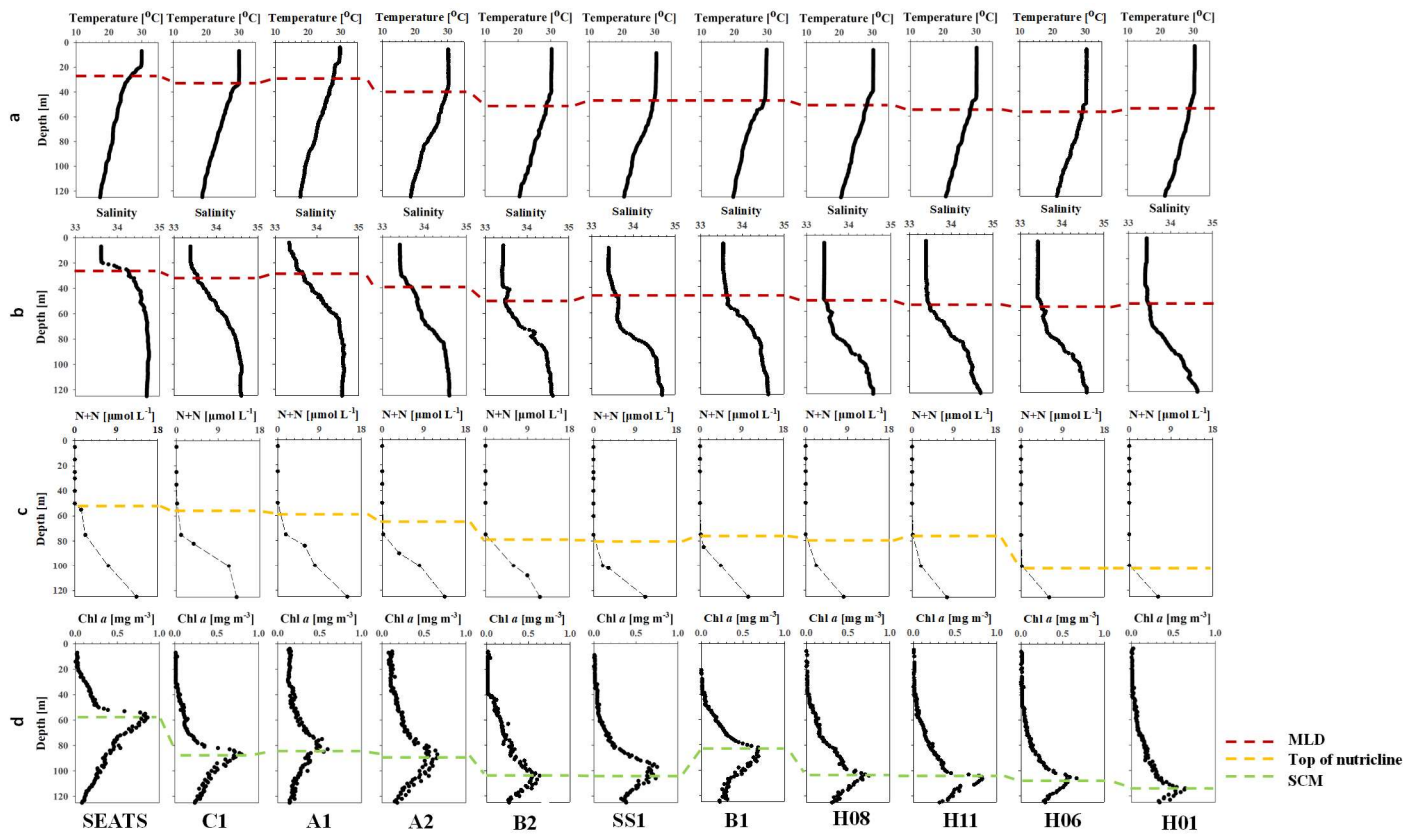
235 Figure 3: Vertical profiles of temperature (a), salinity (b), dissolved inorganic nitrogen (nitrate + nitrite, DIN, c) and Chl a (d). The MLD (red dash), interpolated depth of DIN=0.1 \mu\text{mol L}^{-1} (top of nutricline, yellow dash) and subsurface Chl a Maximum (SCM, green dash) are also shown.
