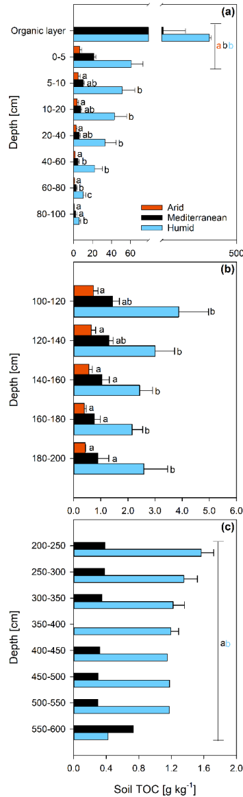
Figure 5: Total organic carbon (TOC) content (mean ± standard error) of soil depth increments down to (a) 100 cm, (b) 200 cm, and (c) 600 cm depth at three sites (arid, mediterranean, humid) located along a precipitation gradient in the Coastal Cordillera of Chile (0-200 cm: n = 3, except for humid site with n = 4; > 200 cm: n = 1, except for humid site 200-400 cm with n = 2). Different letters in both panel a and b indicate significant differences (p ≤ 0.05) among the sites tested by Tukey's posthoc test after Two-Way ANOVA Lines in panels a and c indicate which soil depth increments were combined (separately per site) for statistical analysis.
