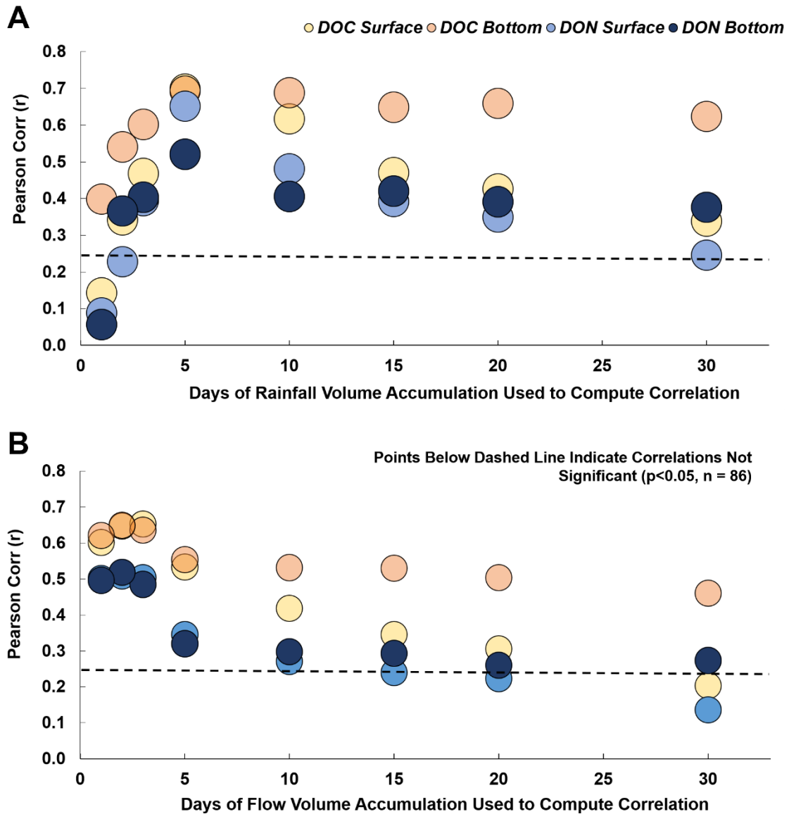
280 Figure 3: Pearson Correlation Coefficients ( r ) ( n = 86 ) between dissolved organic C and dissolved organic N concentrations measured at the Gordon River mouth and (A) accumulated rainfall (B) accumulated flow at the Gordon River mouth. Note that all correlations are statistically significant ( p < 0.05 ) except those circles whose centres are below the dashed line. The x-axis represents the number of days over which the volume of rain or estimated flow is summed and used to compute the correlations between DOC and DON. For instance, 5 days rainfall volume is equal to the rainfall volume measured at Strathgordon Gauge over the 5 days prior to water sampling at station GR1.
