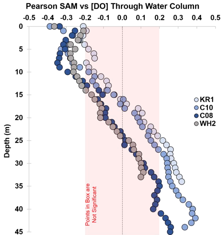
370 Figure 9: Pearson correlation coefficients ( r ) between Southern Annular Mode (SAM) Index and dissolved oxygen concentrations at KR1, C10, C08, and WH2 through the water column at 1m vertical resolution. Red box denotes statistical insignificant correlations while all points outside of the box indicate statistically significant correlations ( p < 0.05 ). Note points reference water depth not height off seabed.
