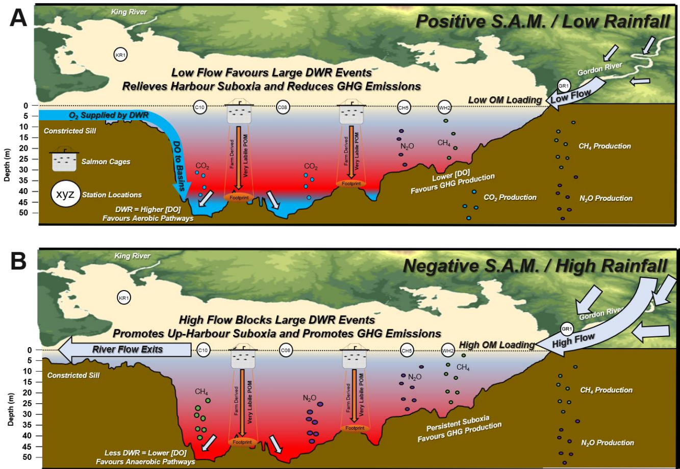
450 Figure 10: Conceptualisation of the role of freshwater inputs on the distribution of DO and potential for GHG production in the Harbour. (A) Harbour DO and GHG during periods of low rainfall (or positive SAM index) promoting DWR. (B) High rainfall (negative SAM index) blocks DWR and promotes the spread of suboxia and thus GHG production.
