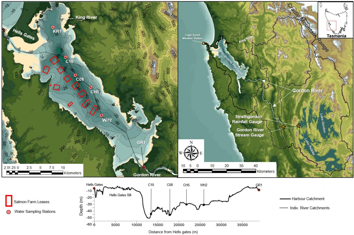
Figure 1: Macquarie Harbour, Tasmania. Monthly sampling sites shown with red circles, Gordon River Stream Gauge and Strathgordon Rainfall Gauge shown as orange stars. Aquaculture lease boundaries are shown as hollow red rectangles. Lease locations are sourced from Land Information Systems Tasmania (LISTmap - https://maps.thelist.tas.gov.au/ ). Station names reflect general harbour locations where KR1 indicates King River 1; C10, C08, CH5 indicate Central Harbour 10, 08, 5; WH2 indicates World Heritage Area 2; and GR1 indicates Gordon River station 1.
