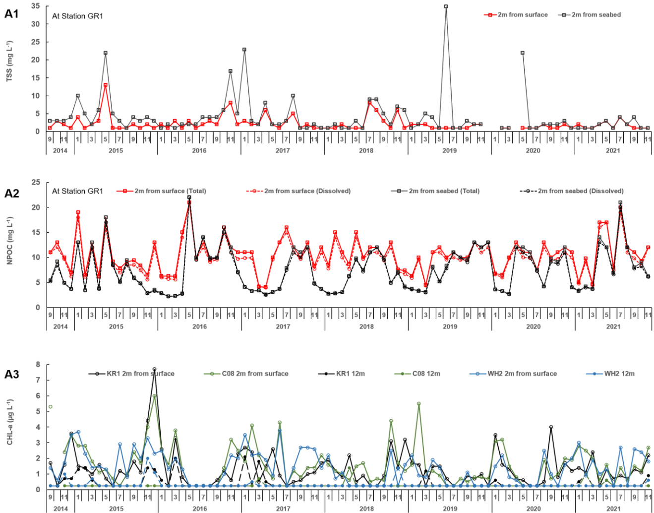
560 Figure for Appendix: (A1) Total Suspended Solids concentrations observed at station GR1. Samples collected 2m from surface (red) and 2m from seabed (black). (A2) Total organic carbon (solid lines) and dissolved organic carbon (dashed lines) concentrations observed at station GR1. Samples collected 2m from surface (red) and 2m from seabed (black). (A3) Chlorophyll-a collected from stations KR1 (black), C08 (green), and WH2 (blue). Samples collected 2m from surface (solid lines open symbols) and 12m from surface (dashed lines closed symbols). All data displayed reflect dates from September 2014 to November 2021 and are used here as an example of Macquarie Harbour water column properties.
