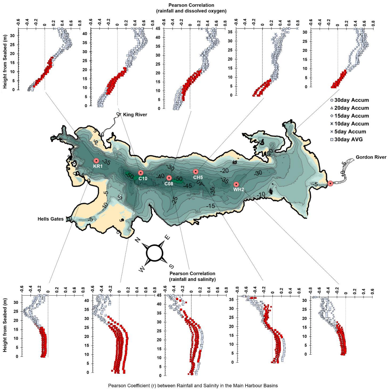
Figure 8: Pearson correlation coefficients (r) between rainfall and dissolved oxygen (top) and rainfall and salinity (bottom) through the water column at 1m vertical resolution. Selected rainfall metrics include accumulation 30 days prior to sampling (circles), 20 days (triangles), 15 days (diamonds), 10 days (asterisk), and 5 day (x) accumulation, and 30 day average daily rainfall prior to sampling (squares). Red symbols denote statistical insignificant correlations ( p < 0.05 ). Vertical dashed lines represent r = 0 .
