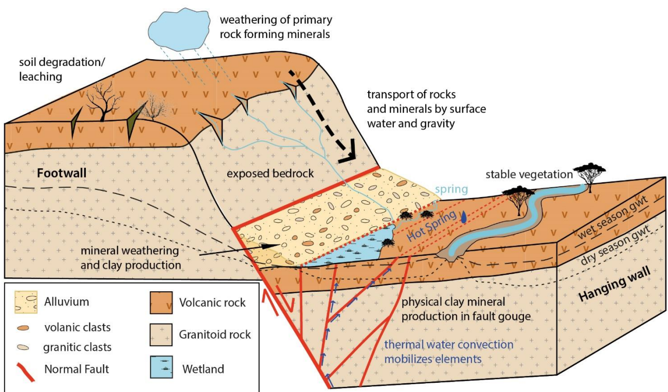
Figure 7 Conceptual model of tectonic activity influencing hydrological and clay forming and/or accumulating processes in a normal fault zone and schematic distribution of different rock types in the study area.
