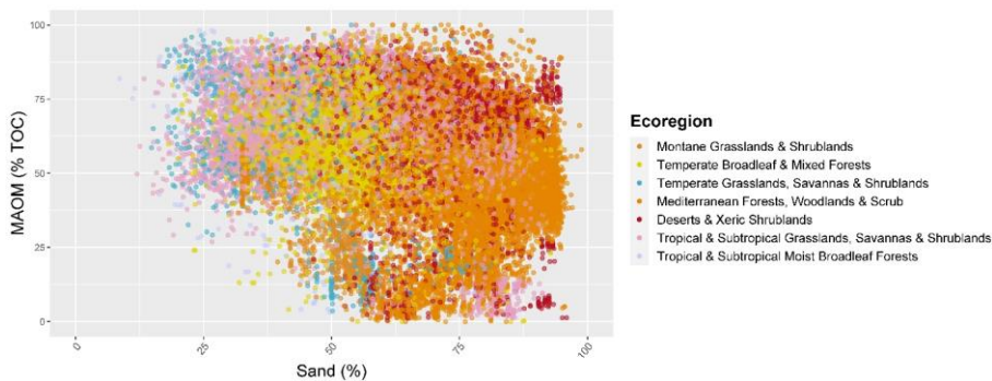
Figure 1149: Allocation of SOC into the mineral-associated organic carbon fraction (MAOC) plotted vs. sand content (%) by biome, from calibration data.
