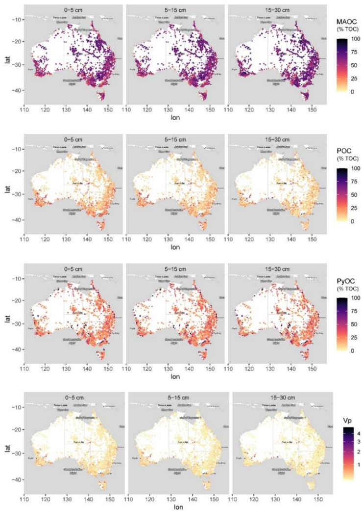
305 Figure 2: Location of the spectral predictions standardized for the depths 0-5 cm, 5-15 cm, and 15-30 cm used as input calibration data for digital soil mapping, standardized for the depths 0-5 cm, 5-15 cm, and 15-30 cm. Contribution of SOC fractions to total
