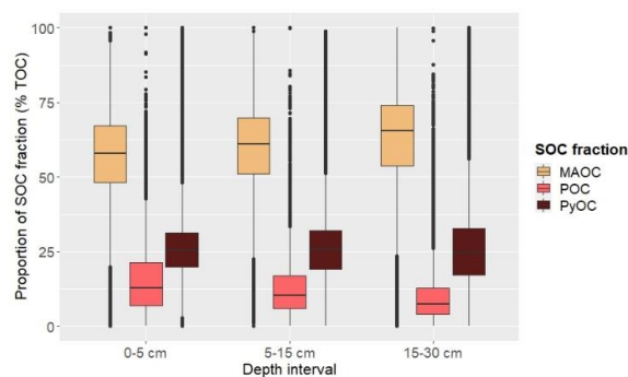
Figure 4: Distribution of total organic carbon (TOC) among three soil organic carbon (SOC) fractions in the spectral dataset calibration dataset . Mineral-associated SOC (MAOC), particulate organic carbon (POC), and pyrogenic organic carbon (PyOC).
