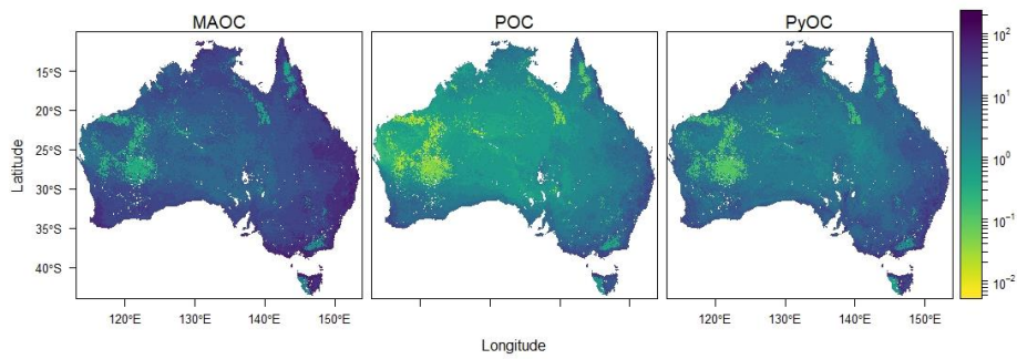
605 Figure 8: SOC fraction stocks (0-30 cm) (Mg C ha -1 ). The values are represented in the log 10 scale.
