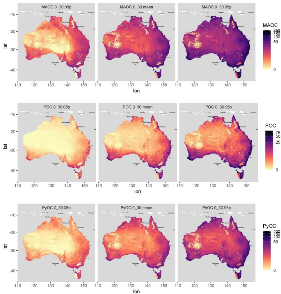
Figure 9: Uncertainty of SOC fraction stocks (Mg C ha -1 ) for the 0-30 cm calculated with 500 simulations in a subset of 98,400 pixels.
