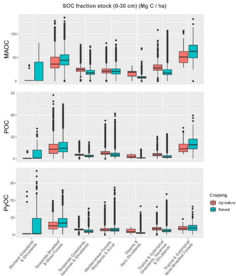
620 Figure 109: SOC fraction stock (Mg C ha -1 ) by biome and land use. Mineral-associated SOC (MAOC), particulate organic carbon (POC), pyrogenic organic carbon (PyOC).
