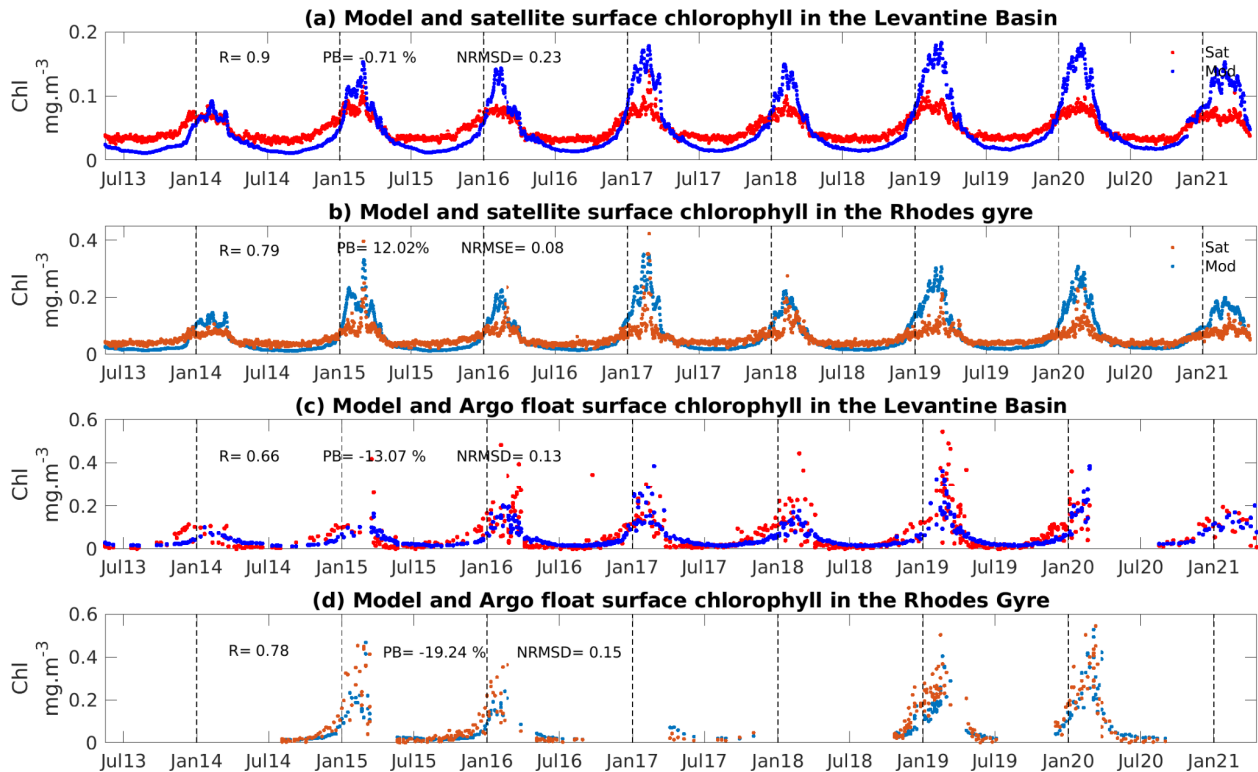
Figure 1.2 (Figure 2 of the manuscript): Time series of (a) modeled (in blue) and satellite (in red) surface chlorophyll-a concentration ( \text{mg m}^{-3} ) averaged over (a) the Levantine Basin and (b) the Rhodes Gyre. Time series of (c)-modeled (in blue) and BGC-Argo float (in red) surface chlorophyll-a concentration ( \text{mg m}^{-3} ) (c) in the Levantine Basin and (d) in the Rhodes Gyre. Coefficient correlation (R), percent bias (PB) and Normalized Root Mean Square Deviation (NRMSD) between model outputs and observations are indicated in (a), (b), (c) and (d).
