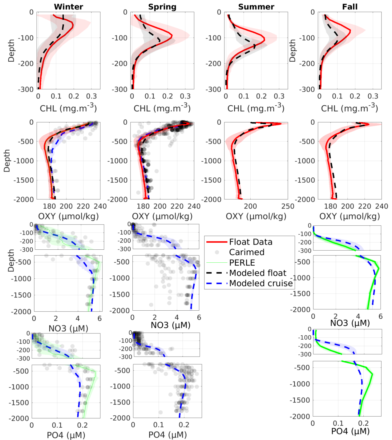
Figure 1.3 (Figure 3 of the manuscript): Comparison over the Levantine Sea between observed (gray points for CARIMED, green lines for PERLE1 and PERLE2, red line for BGC-Argo float data) and modeled (blue and black lines) profiles of chlorophyll ( \text{mg Chl m}^{-3} ), dissolved oxygen ( \mu\text{mol kg}^{-1} ), nitrate ( \mu\text{M} ) and phosphate ( \mu\text{M} ) concentrations, averaged by season (winter: 21 December to 20 March, spring: 21 March to 20 June, summer: 21 June to 20 September, fall: 21 September to 20 December). Shaded areas represent standard deviation.
