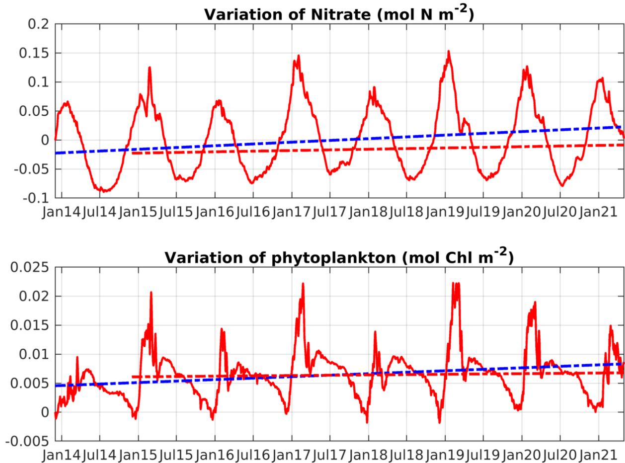
Figure 2.1: Time evolution of the variation of the nitrate and phytoplankton ( \text{mol m}^{-2} ) inventory averaged over the Rhodes Gyre surface layer (0-150 m). The blue line represents the trend from December 2013-May 2021, the red line, the trend excluding the first year (December 2014-May 2021).
