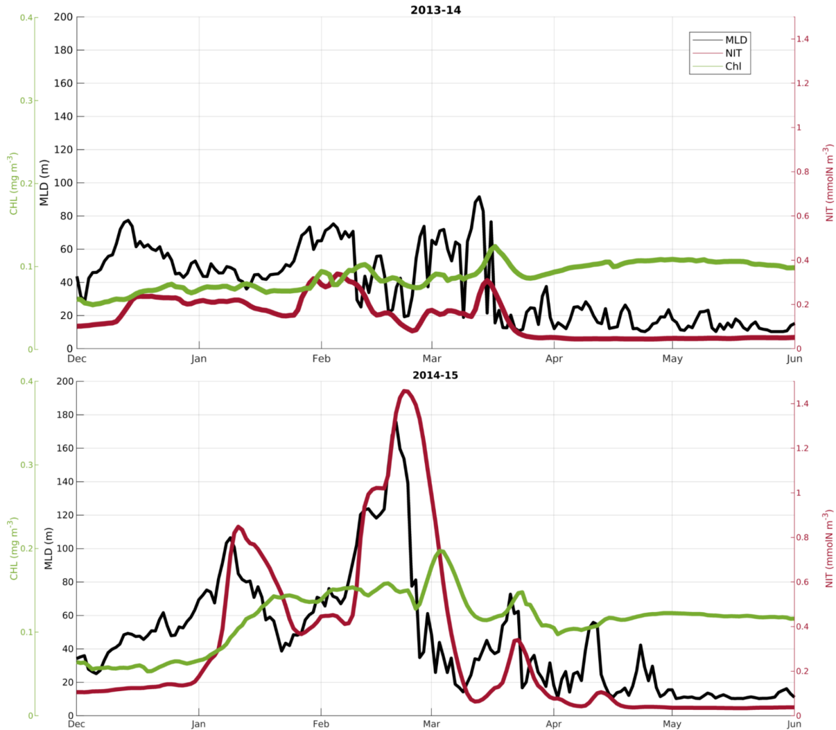
Figure 2.2 (modified Figure 11 in the submitted manuscript): Annual cycle of the Mixed Layer Depth (MLD, m) (black), surface chlorophyll (CHL, \text{mg m}^{-3} ) (green) and nitrate (NIT, \text{mmol N m}^{-3} ) (red) concentration-concentration, net primary production (NPP, \text{mmol C m}^{-2} \text{day}^{-1} ) (blue) in the upper layer (0-150 m), and the organic carbon export ( \text{mmol C m}^{-2} \text{day}^{-1} ) at 150 m depth (purple), for years 2013-14, and 2014-15, 2016-17.
