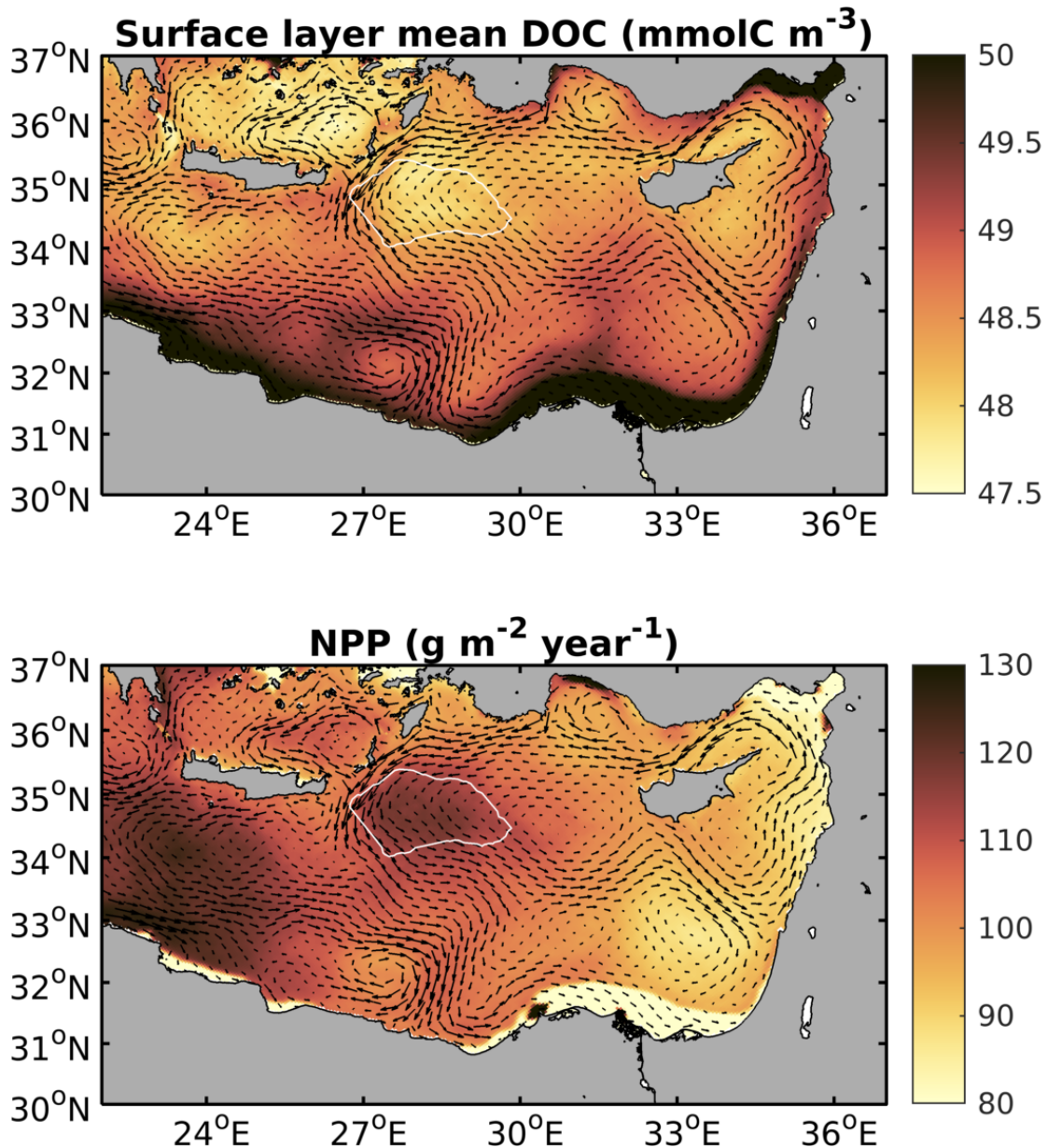
Figure 1.5: Modeled (a) surface layer mean dissolved organic carbon concentration (mmolC/m 3 ) and (b) net primary production (g/m 2 /year), averaged over the period from December 2013 to December 2020. The arrows represent the surface currents averaged over the period of study, the white contour delimits the Rhodes Gyre.
