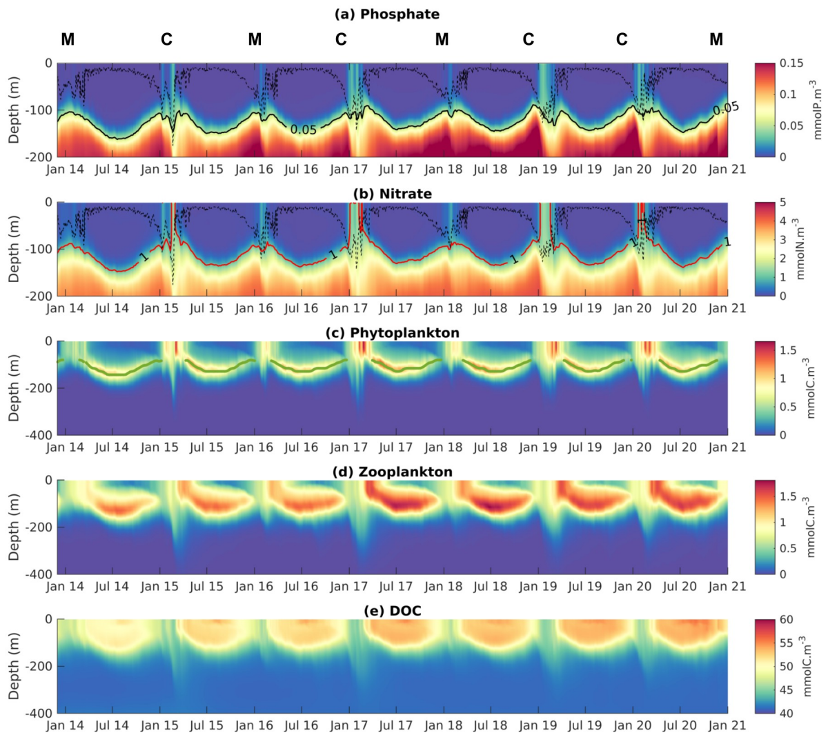
1265 Figure 6: Hovmöller diagrams of modeled (a) phosphate ( \text{mmol P m}^{-3} ), (b) nitrate ( \text{mmol N m}^{-3} ), (c) phytoplankton ( \text{mmol C m}^{-3} ), (d) zooplankton ( \text{mmol C m}^{-3} ) and (e) dissolved organic carbon ( \text{mmol C m}^{-3} ) concentrations averaged over the Rhodes Gyre, from December 2013 to January 2021. The black dotted line in (a) and (b) indicates the mixed layer depth. The red line represents the depth of the nitracline in (b), and the black one of the phosphocline in (a). The green dotted line in (c) indicates the deep chlorophyll maximum. C refers to cold winter years and M to mild winter years.
