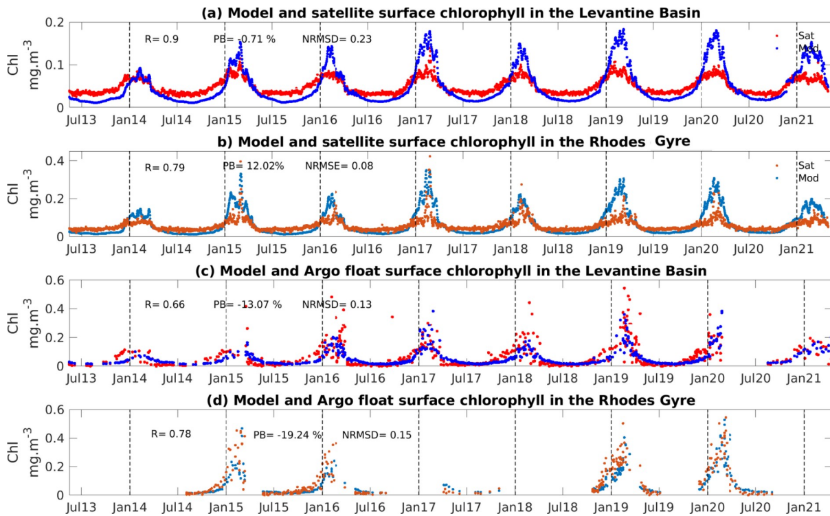
1220 Figure 2: Time series of modeled (in blue) and satellite (in red) surface chlorophyll-a concentration ( \text{mg m}^{-3} ) averaged over (a) the Levantine Basin and (b) the Rhodes Gyre. Time series of modeled (in blue) and BGC-Argo float (in red) surface chlorophyll-a concentration ( \text{mg m}^{-3} ) (c) in the Levantine Basin and (d) in the Rhodes Gyre. Coefficient correlation (R), percent bias (PB) and Normalized Root Mean Square Deviation (NRMSD) between model outputs and observations are indicated in (a), (b), (c) and (d).
