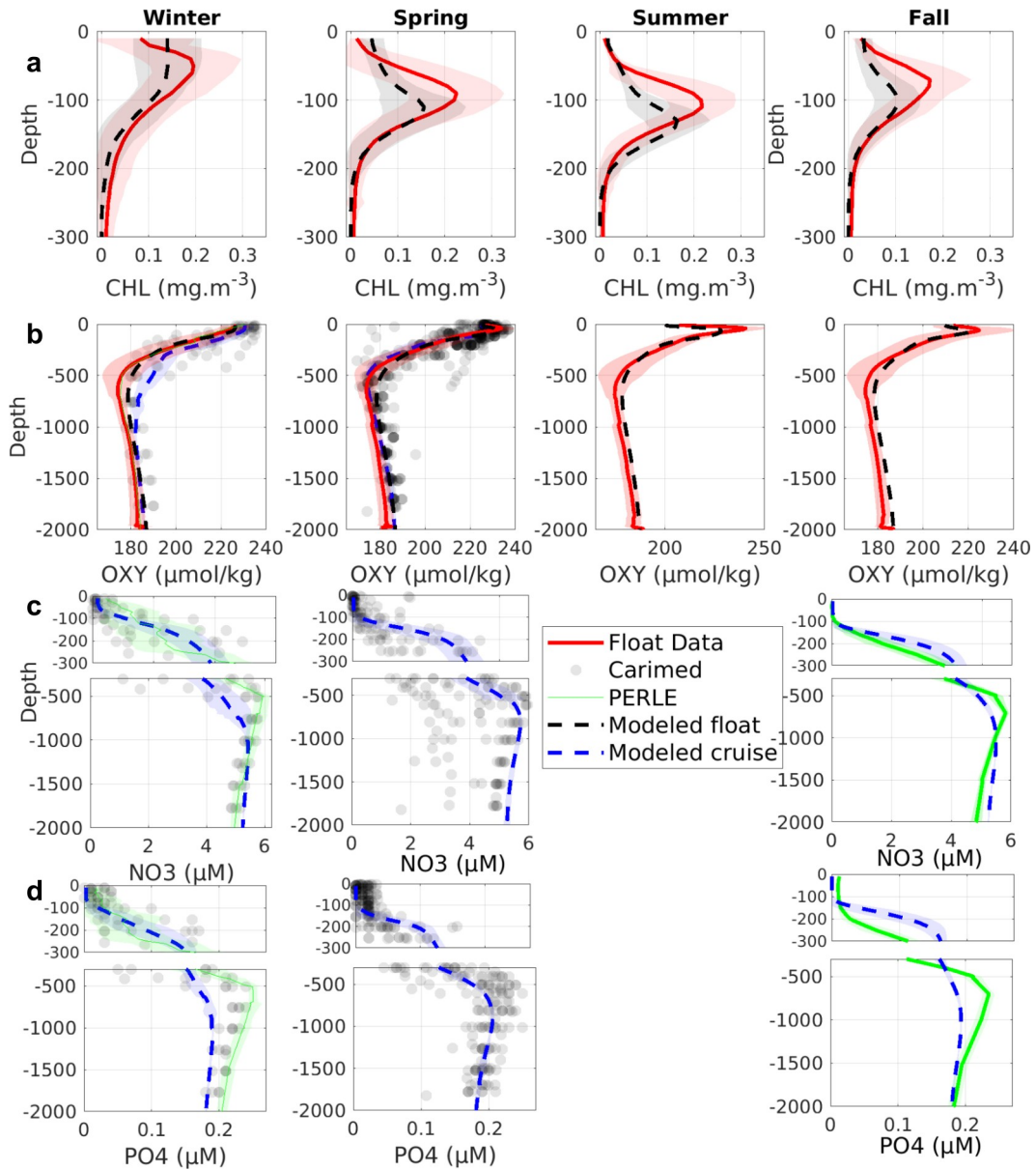
1225 Figure 3: Comparison over the Levantine Sea between observed (gray points for CARIMED, green lines for PERLE1 and PERLE2, red line for BGC-Argo float data) and modeled (blue and black lines) profiles of chlorophyll ( \text{mg Chl m}^{-3} ), dissolved oxygen ( \mu\text{mol kg}^{-1} ), nitrate ( \mu\text{M} ) and phosphate ( \mu\text{M} ) concentrations, averaged by season (winter: 21 December to 20 March, spring: 21 March to 20 June, summer: 21 June to 20 September, fall: 21 September to 20 December). Shaded areas represent standard deviation.
