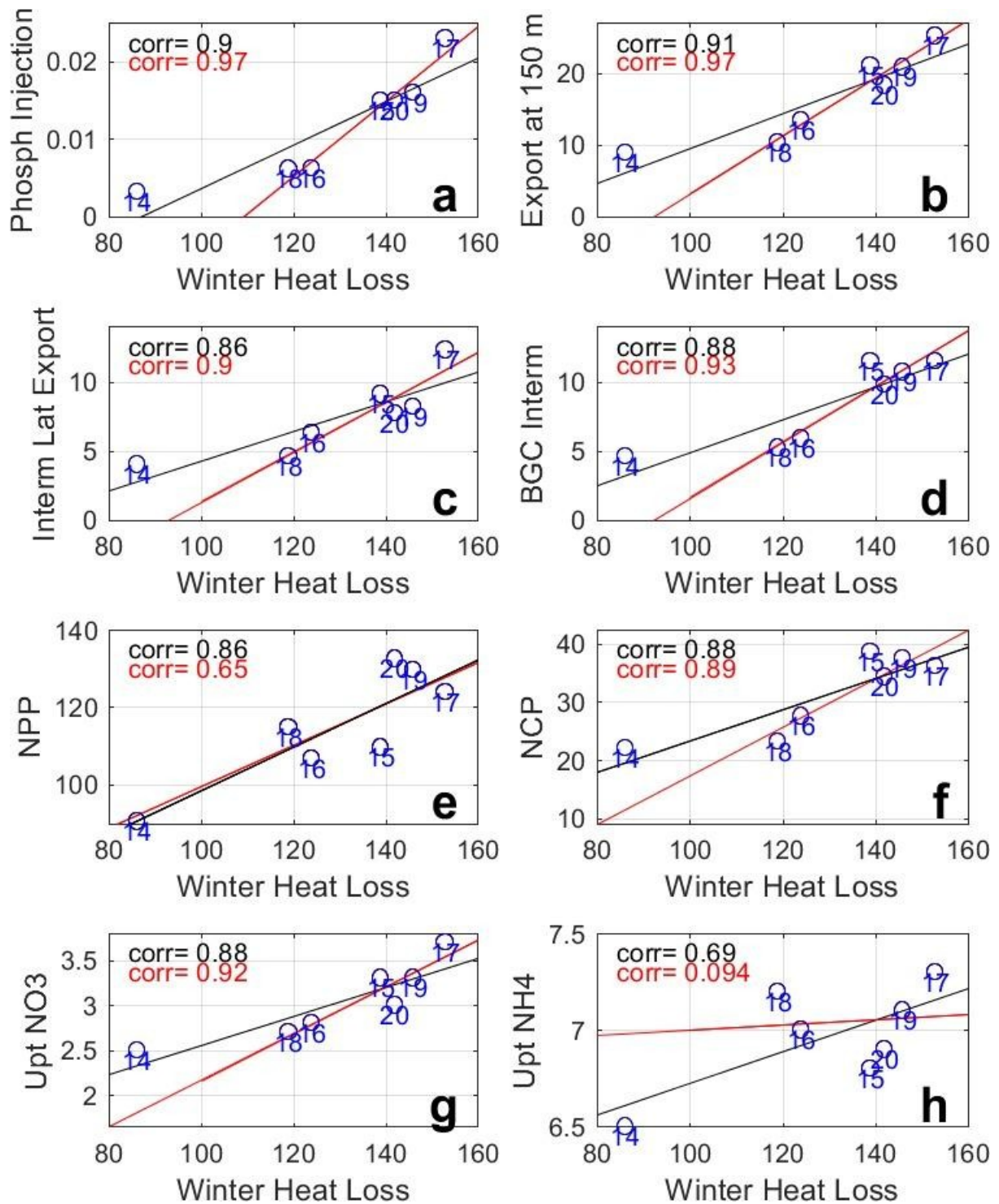
1255 Figure 10: Scatter-plot of winter surface heat loss ( W m^{-2} ) vs. (a) winter phosphate injection ( mol P m^{-2} ) into the 1260 surface layer and mean annual values of (b) downward export of OC (Organic Carbon) at 150 m ( gC m^{-2} year^{-1} ), (c) lateral export from the intermediate layer ( gC m^{-2} year^{-1} ), (d) biogeochemical consumption in the intermediate layer ( gC m^{-2} year^{-1} ), (e) NPP, (f) NCP ( gC m^{-2} year^{-1} ), (g,h) uptake of nitrate and ammonium ( mmol N m^{-2} year^{-1} ). The years are identified by the numbers in blue, e.g. 14 stands for 2013-14. The black line shows the seven years linear regression and the red line shows the linear regression when excluding 2013-14. The corresponding correlations are shown with the same color code.
