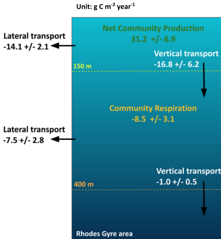
Figure 9: Annual organic carbon budget ( \text{g C m}^{-2} \text{year}^{-1} ) in the surface and intermediate layers of the Rhodes Gyre for the seven year period 2013-2020.
