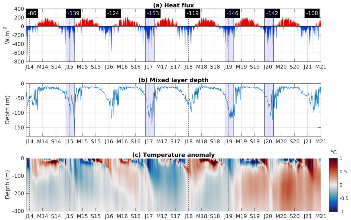
Figure 5: Time series of modeled (a) surface heat fluxes ( W m^{-2} ), (b) mixed layer depth (m) and (c) temperature anomaly ( ^{\circ}C ), averaged over the Rhodes Gyre area. The winter (December-January-February) mean heat flux is indicated in black rectangles in (a). J: January M: May S: September. Winters with strong heat loss and deeper mixed layers are emphasized in blue in (a) and (b).
