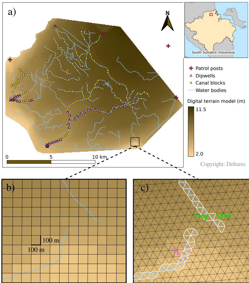
Figure 1. Study area and peat hydrological module (PHM) mesh. (a) Digital terrain model (brown gradient), water bodies (blue lines), dipwells (pink triangles), canal blocks (yellow dots) and patrol posts (red crosses). Each patrol post consist of a weather station and six daily measured dipwells along a 200 m transect. The rest of the dipwells were measured manually with monthly frequency. Native forest species are the main vegetation cover. The area extends from ( 2^{\circ}5'29'' S 104^{\circ}3'14'' E) to ( 1^{\circ}57'11'' S 104^{\circ}14'1'' E). (b) and (c) Zoomed in region near two canals in the southern part of the study area. (b) Original 100\text{ m} \times 100\text{ m} resolution of the digital terrain model, which was later interpolated to 50\text{ m} \times 50\text{ m} . (c) Triangular mesh for the peat hydrological module (PHM). The white segments show the mesh cell faces corresponding to the canals, which were treated differently. This difference is emphasized with the green and pink schematic annotations. Two cell faces are shown in green: one is the cell face between two canal mesh cells, and has a null hydraulic transmissivity, T = 0 , because flow along the canals occurs only in the canal network module (CNM); the other is the cell face between a canal and a peat mesh cell and therefore T \neq 0 in general. In pink we indicate the lateral inflow per unit length, q , between the peat and canal mesh cells.
