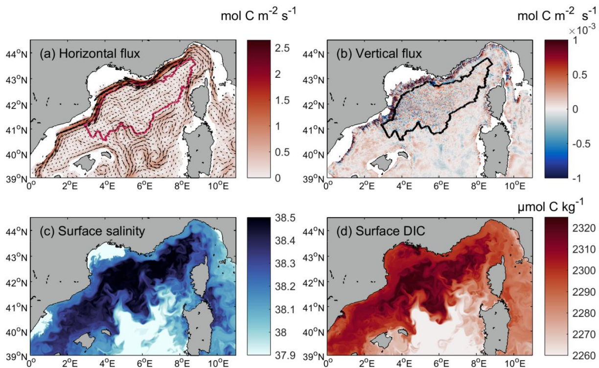
Figure 10: (a) Winter horizontal flux of dissolved inorganic carbon (DIC, \text{mol C m}^{-2} \text{s}^{-1} ), vertically integrated over the upper layer (0-150 m), (b) winter vertical DIC flux ( \text{mol C m}^{-2} \text{s}^{-1} ) at 150 m, (c) surface salinity and (d) DIC concentration ( \mu\text{mol C kg}^{-1} ) on 4 March 2013. The red and black lines in (a) and (b), respectively, indicate the limit of the deep convection area.
