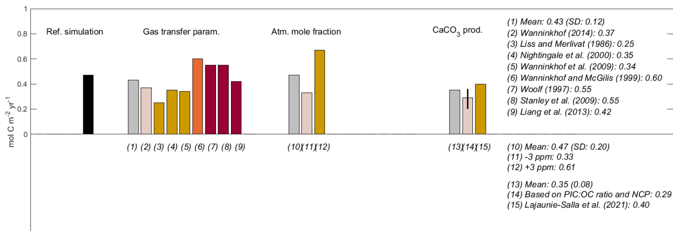
1260 Figure 13: Sensitivity tests to the parameterization of gas transfer velocity, the variability of the mole fraction of CO 2 in the 1265 atmosphere, and the calcification processes, on the annual air-to-sea CO 2 flux estimate. The black bar indicates the annual estimate in the reference simulation, grey bars the mean value for each of the three sets of sensitivity tests. For the sensitivity tests on the parameterization of gas transfer (from 2 to 9), relations with a quadratic (2), hybrid (3 to 5), cubic (6) wind speed dependency are respectively in light pink, yellow and orange, and relations that include explicit bubble parametrizations (7 to 9) are in red. For the test (14) on calcification processes, the bar indicates the result found for the mean PIC:POC ratio, while the black line indicates the range using the minimum and maximum PIC:POC ratios.
