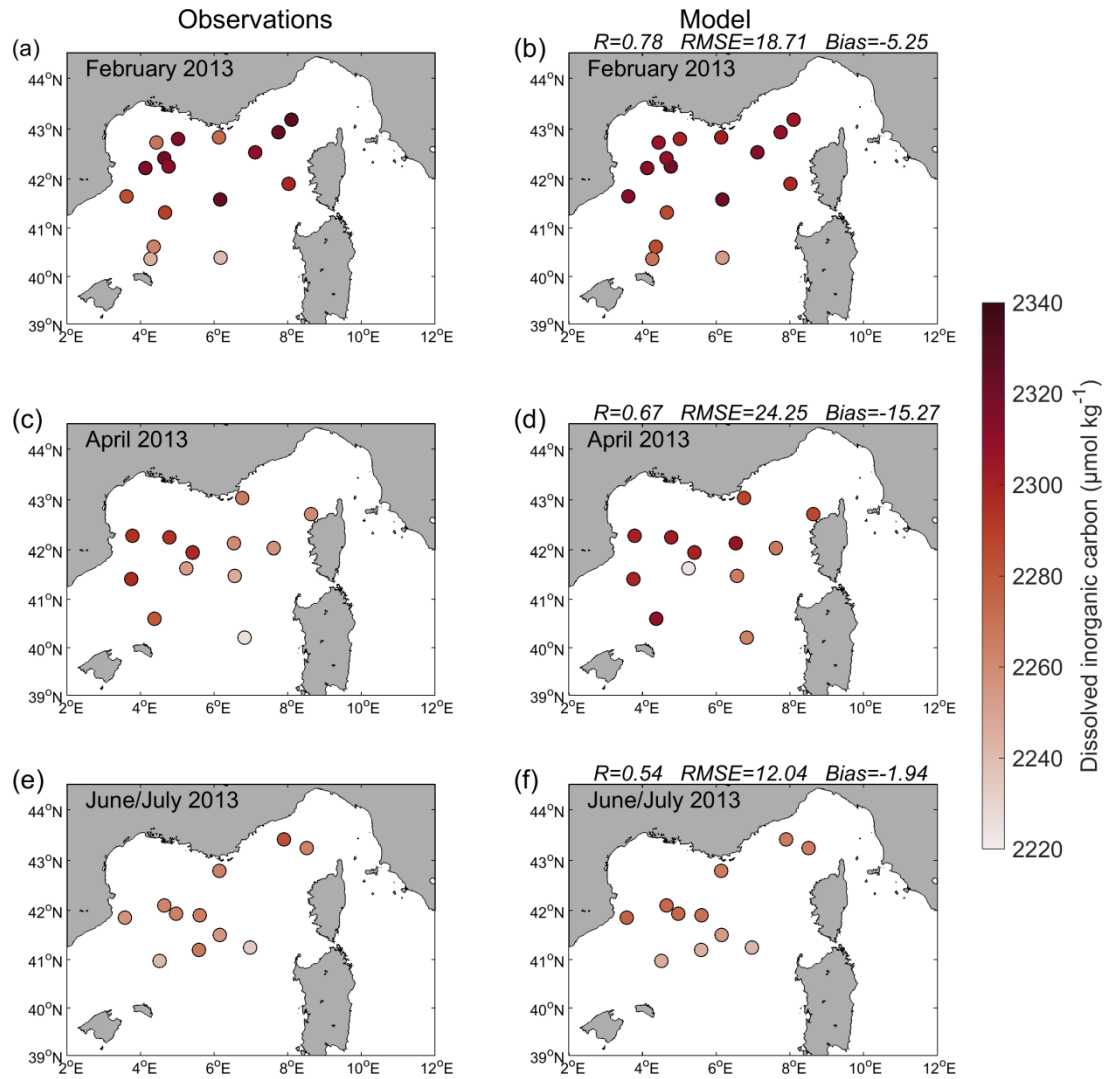
1180 Figure 4: Surface dissolved inorganic carbon (DIC) concentration ( \mu\text{mol kg}^{-1} ) observed (left) and modeled (right) over the (a,b) DEWEX Leg1 (1-21 February 2013), (c,d) DEWEX Leg2 (5-24 April 2013), and (e,f) MOOSE-GE (11 June-9 July 2013) cruise periods. The correlation coefficient ( R ), root mean square error ( RMSE ), and bias between surface observed and modeled DIC are indicated in (b,d,f).
