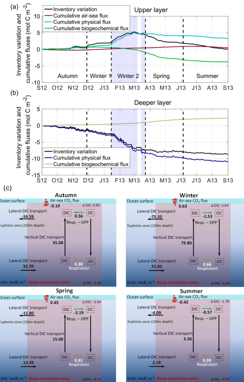
Figure 7: Time series of variation in dissolved inorganic carbon (DIC) inventory since the 1 st September 2012 (black) and cumulative air-sea (red), physical (light and dark blue), and biogeochemical (bright and brown green) flux of dissolved inorganic carbon in the (a) upper (surface to 150 m) and (b) deeper (150 m to bottom) layers, from September 2012 to September. The cumulative flux at a day d is the time-integrated flux over the period from the 1 st September 2012 to day d. Unit: mol C m -2 . Positive values of fluxes represent DIC inputs for the deep convection area. The blue shaded area corresponds to the deep convection period (period when spatially averaged mixed layer depth > 100 m). The DIC inventory on 1 st September 2012 was 353 and 5560 mol C m -2 in the upper and deeper layers, respectively. (c) Scheme of cumulative seasonal fluxes in mol C m -2 over the respective periods (fall: 88 days, winter: 116 days, spring: 74 days and summer: 87 days). Resp. stands for respiration and GPP for gross primary production. The direction of the arrows indicates the direction of the fluxes and positive values correspond to DIC inputs for the deep convection area.
