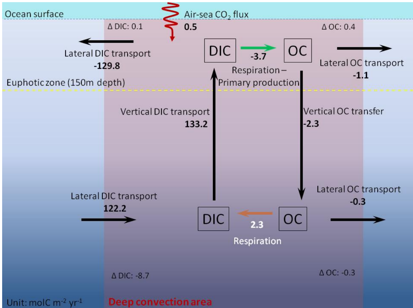
1245 Figure 11: Scheme of the annual carbon budget for the period September 2012 to September 2013 from the coupled model SYMPHONIE-Eco3M-S. Fluxes are indicated in \text{mol C m}^{-2} \text{ yr}^{-1} . The direction of the arrows indicates the direction of the fluxes and positive values of fluxes represent DIC inputs for the deep convection area (positive vertical fluxes represent inputs for the upper layer).
