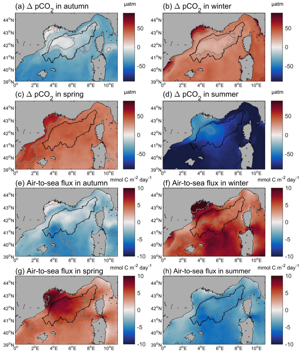
1220 Figure 8: Seasonal averages of modeled (a to d) p\text{CO}_2 difference ( p\text{CO}_{2,\text{atm}} - p\text{CO}_{2,\text{sea}} , in \mu\text{atm} ), and (e to h) air-to-sea \text{CO}_2 flux ( \text{mmol C m}^{-2} \text{day}^{-1} ). Note that the periods of seasons here are defined in Sect. 4.1 according to mixed layer depth and biogeochemical processes (Fall: 1 September-27 November, Winter: 28 November-23 March, Spring: 24 March-5 June, Summer: 6 June-31 August). Grey lines indicate in (a) to (d) p\text{CO}_2 difference isolines (-50, -25, -10, 0, 10, 25, 50 \mu\text{atm} ), in (e) to (h) \text{CO}_2 flux isolines (-10, -5, 0, 5, 10 \text{mmol C m}^{-2} \text{day}^{-1} ), and the black line the limit of the deep convection area.
