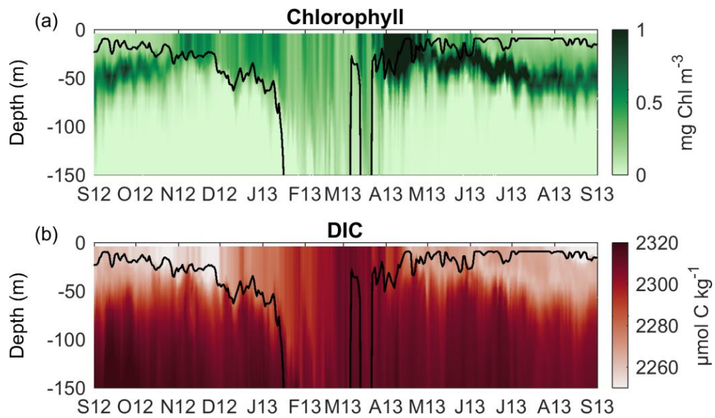
1230 Figure 9: Time evolution of (a) chlorophyll-a ( \text{mg Chl m}^{-3} ) and (b) dissolved inorganic carbon (DIC, \mu\text{mol C kg}^{-1} ) concentration profile, with mixed-layer depth (m) indicated by the black line, horizontally averaged over the deep convection area.
