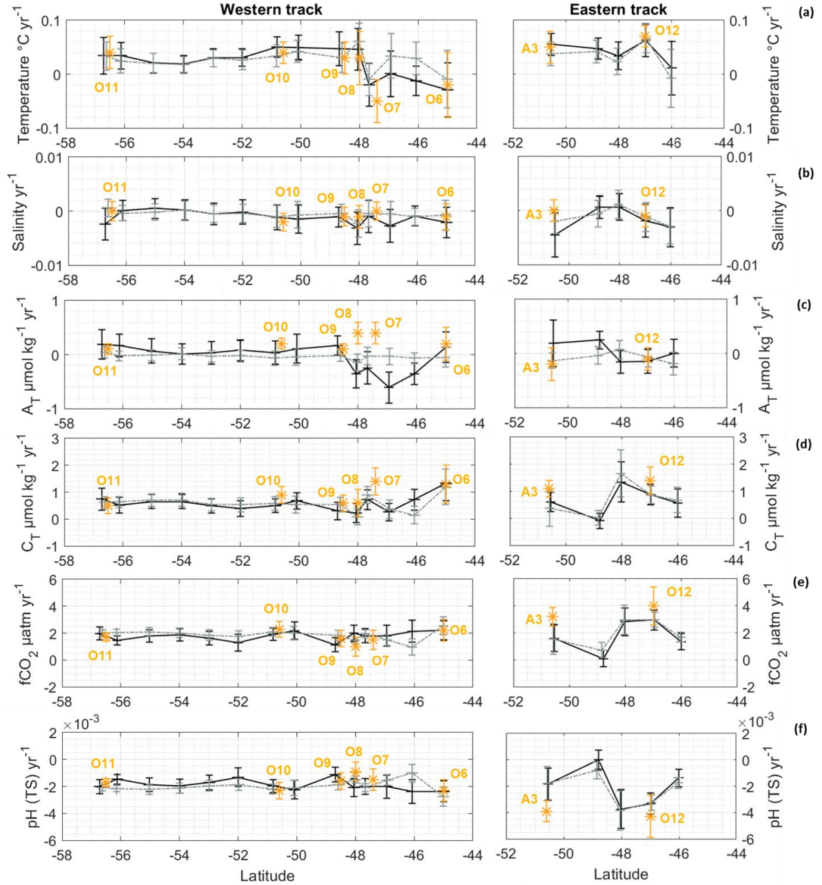
5 Figure 4. Trends (per year) of temperature (a), salinity (b), A_T (c), C_T (d), fCO_2 (e) and pH (f) evaluated from the fCO_2 surface dataset (in grey), the A_T C_T surface dataset (in black) and the A_T C_T data in the mixed layer at each station (in orange) along the western and eastern tracks (see Fig. S4). The computation method is explained in the section 2.3.
