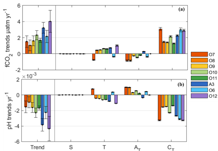
Figure 6. Trends and decomposition of fCO 2 (a) and pH (b) trends in the summer mixed layer, according to Equation 9. The effect of change in salinity (S), temperature (T), A T and C T are shown. The three phytoplanktonic bloom stations are reported in blue/purple (last ones) and are separated from the HNLC stations (first five).
