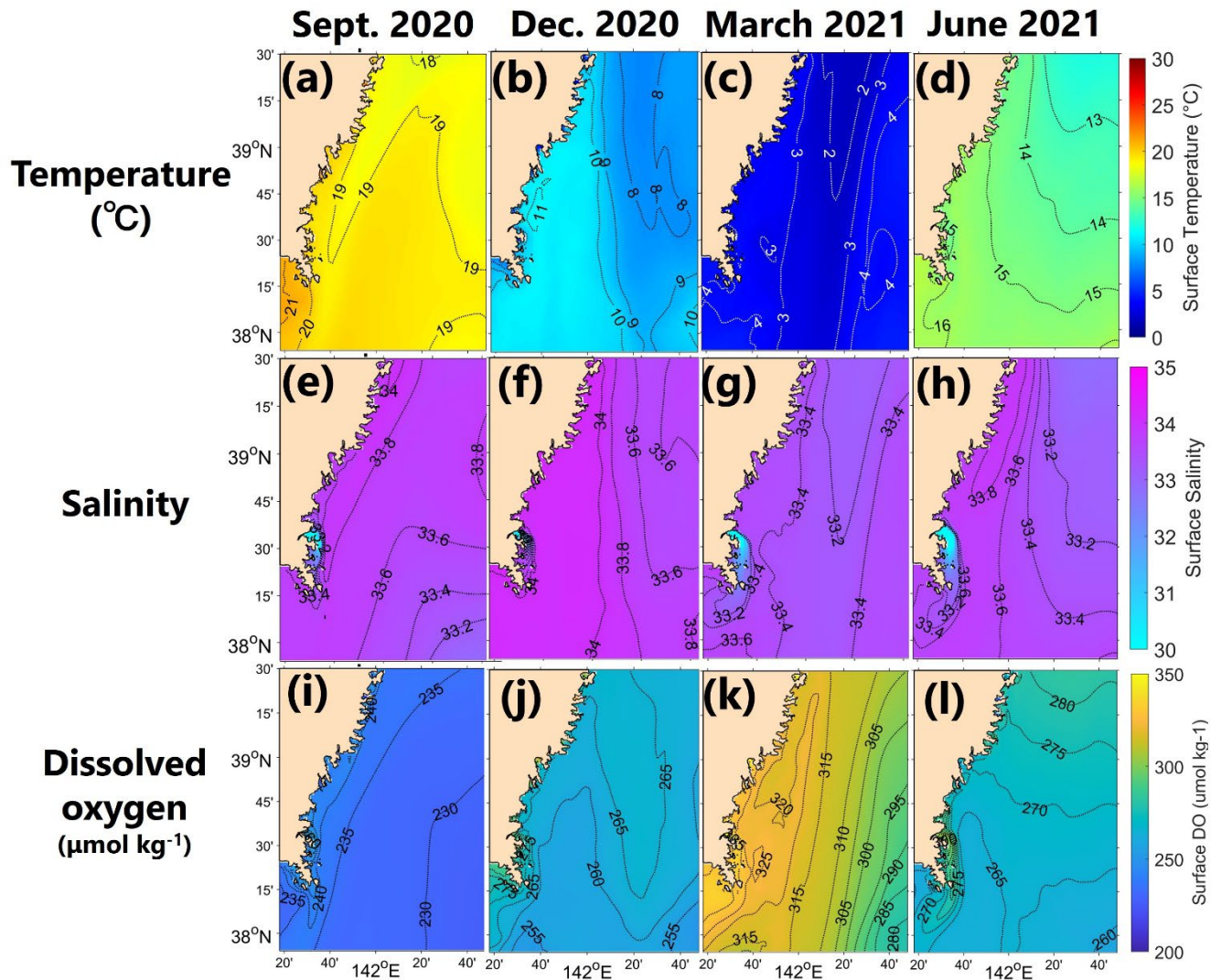
Figure 9: Horizontal distribution of modeled monthly-mean surface temperature ( ^{\circ}\text{C} ) ((a)-(d)), salinity ((e)-(h)) and DO ( \mu\text{mol kg}^{-1} ; (i)-(l)) in September, December, March and June in the model domain of Shizugawa Bay.
