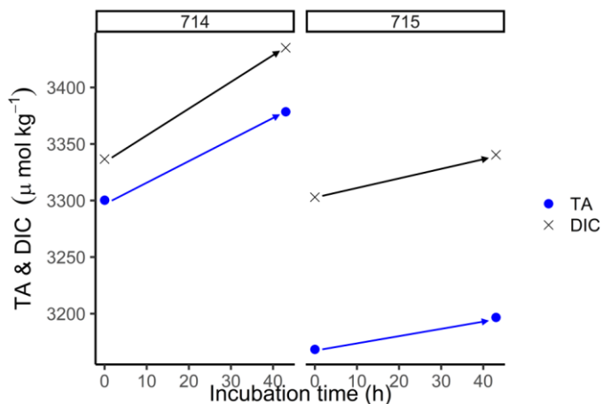
Figure 6. BOD incubations. The start (0h) and end (43h) concentrations of total alkalinity (TA) (blue/black dots) and dissolved inorganic carbon (DIC) (black crosses/white dots) of the BOD incubation samples from station 714 and 715, respectively.
