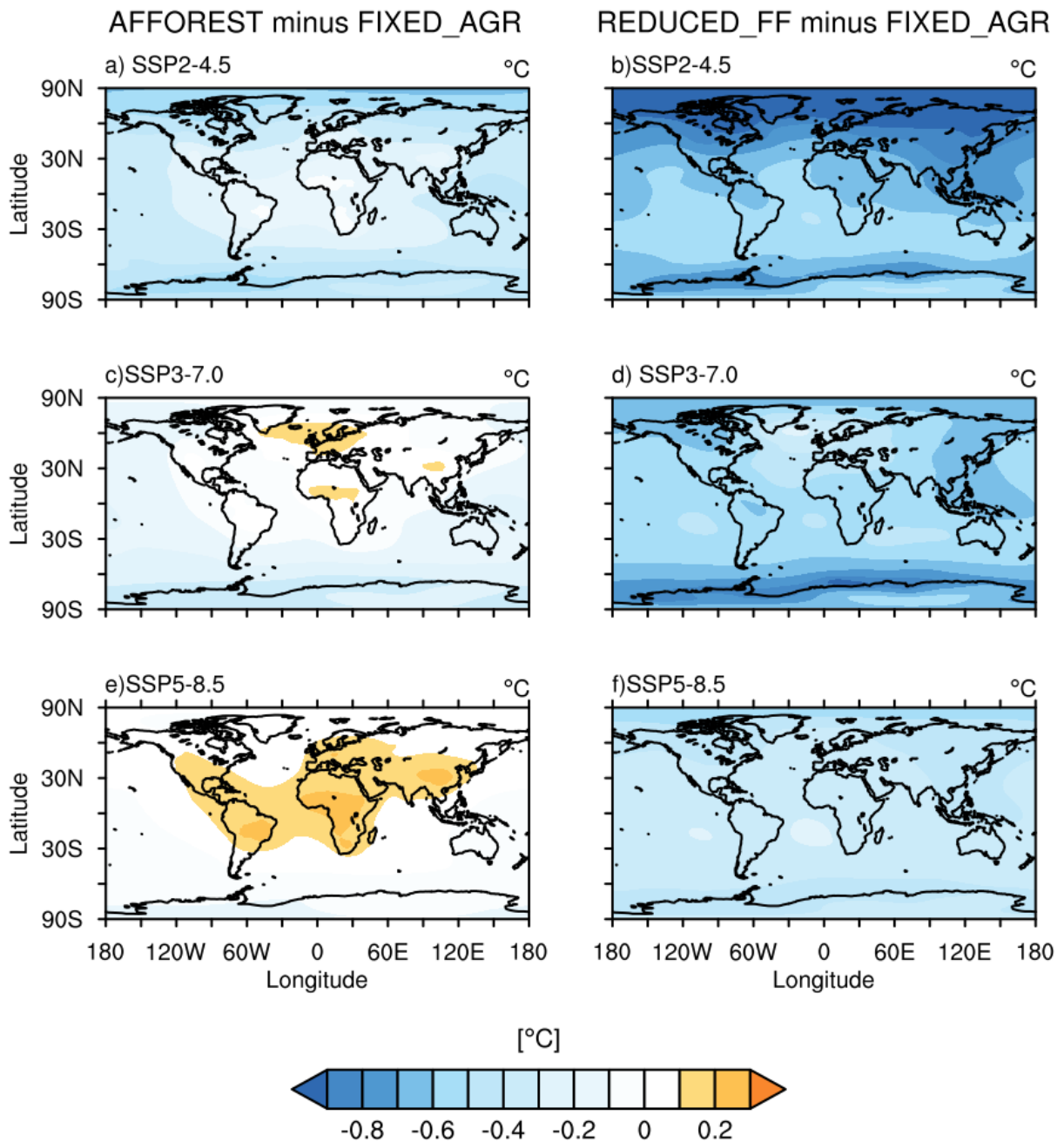
675 Figure 5. The left (right) panel shows the spatial pattern of the difference in global mean surface air temperature (SAT) averaged over the last 30 years between the AFFOREST (REDUCED_FF) and FIXED_AGR cases. The top, middle and bottom panels correspond to the SSP2-4.5, SSP3-7.0 and SSP5-8.5 scenarios, respectively. The REDUCED_FF case shows lower SAT everywhere relative to the FIXED_AGR case in the three SSP scenarios, while the AFFOREST case shows regional warming relative to the FIXED_AGR case in the SSP3-7.0 and SSP5-8.5 680 scenarios. Note that the regions of warming in the AFFOREST case is more prominent over land where the forest regrowth results in a lower land surface albedo (Figure S14).
