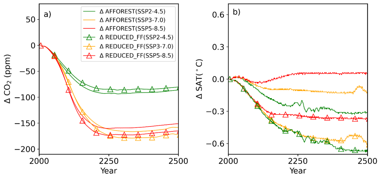
660 Figure 4. Changes in a) global mean atmospheric CO 2 concentration and b) global mean surface air temperature in the AFFOREST (solid lines; ΔAFFOREST) and REDUCED_FF (solid lines with triangle markers; Δ REDUCED_FF) cases relative to the FIXED_AGR case in the SSP2-4.5 (green), SSP3-7.0 (orange) and SSP5-8.5 (red) scenarios. The decrease in atmospheric CO 2 because of afforestation or reduced fossil fuel emissions is almost twice in SSP3-7.0 and SSP5-8.5 compared to SSP2-4.5 due to two reasons: i) amount of carbon removed by land is larger in the SSP3-7.0 and SSP5-8.5 scenarios because of larger CO 2 -fertilization effect as discussed in Sect 3.1 ii) larger ocean carbon uptake in the FIXED_AGR case relative to the AFFOREST and REDUCED_FF cases in the SSP2-4.5 compared to SSP3-7.0 and SSP5-8.5 scenarios (Table 2). The REDUCED_FF case has a lower SAT than the FIXED_AGR case in the three SSP scenarios because of reduced fossil fuel emissions in the REDUCED_FF case. In the AFFOREST case, the cooling effect of the removal of CO 2 is partially or completely offset by the biophysical warming effects from regrowth of forests. Hence, the AFFOREST case has similar SAT as that of the FIXED_AGR case in the SSP3-7.0 and SSP5-8.5 scenarios and a smaller SAT in the SSP2-4.5. 665 670
