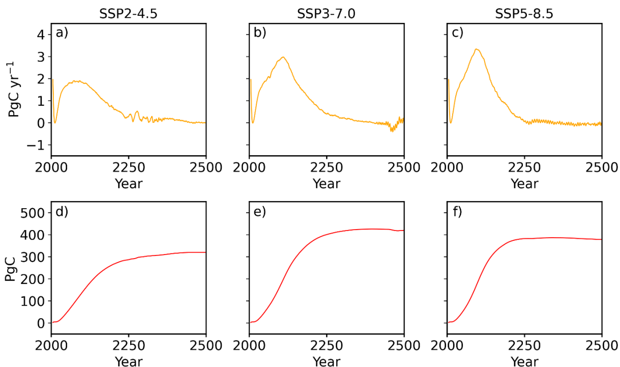
620 625 Figure 1. Top panels show the amount of carbon additionally stored in land in each year in the AFFOREST case compared to the FIXED_AGR case in a) SSP2-4.5, b) SSP3-7.0 and c) SSP 5-8.5 scenarios, respectively. The bottom panels show the cumulative amount of additional carbon storage in land in the AFFOREST case compared to the FIXED_AGR case each year in d) SSP2-4.5, e) SSP 3-7.0 and f) SSP5-8.5 scenarios, respectively. In the AFFOREST simulations, the amount of carbon additionally stored in the land (between 2006-2500) compared to the FIXED_AGR case are 319.84 PgC, 418.93 PgC, and 379.21PgC in the SSP2-4.5, SSP3-7.0, and SSP 5-8.5 scenarios, respectively. The initial peak in yearly additional carbon storage is due to the rapid growth of vegetation over abandoned agricultural land in the AFFOREST case. The second peak is due to the gradual increase in tree fraction in the AFFOREST case (Figure S5).
