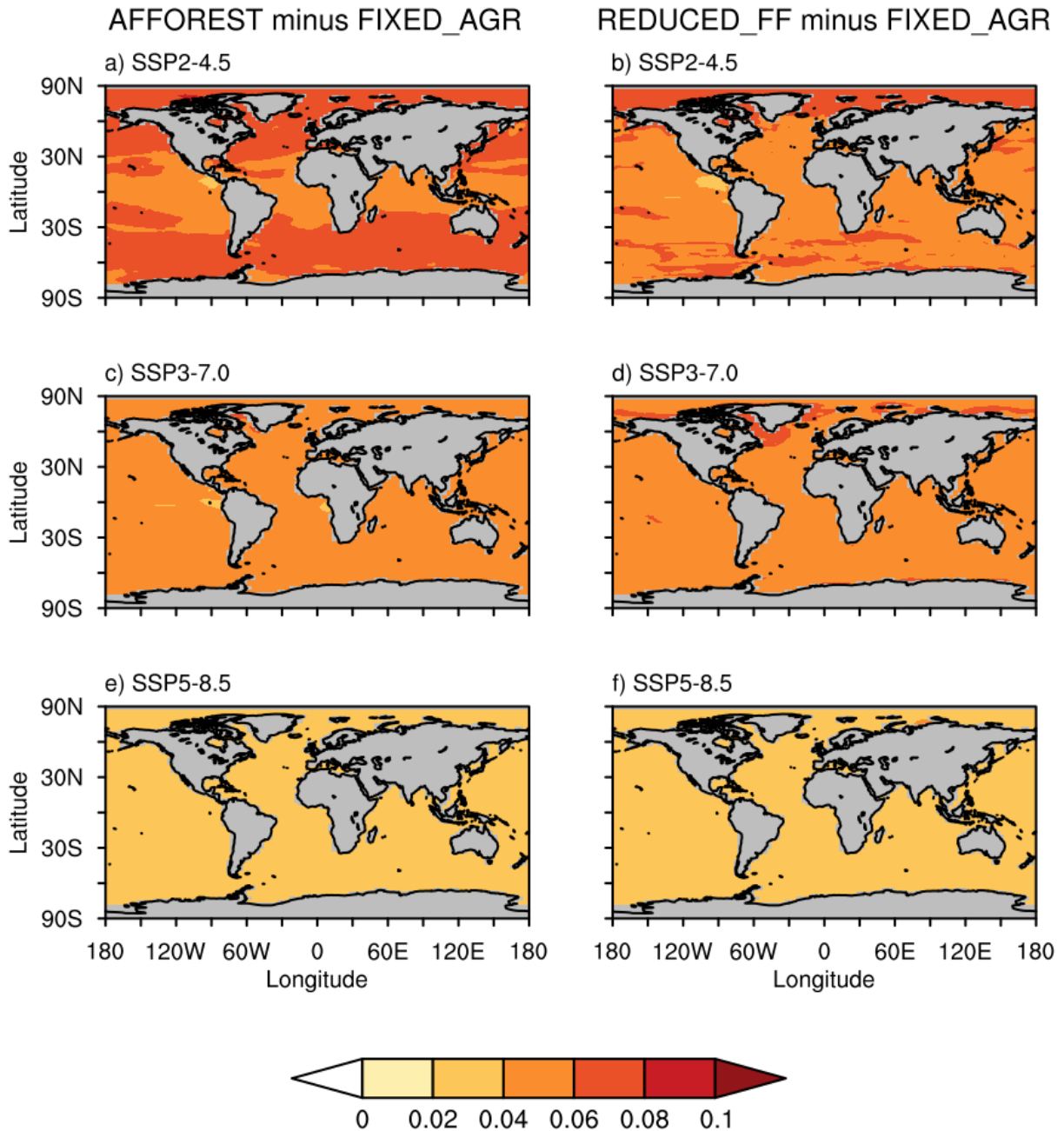
705 Figure 8. The left (right) panel shows the spatial pattern of the difference in global mean surface ocean pH (averaged over 2471-2500) between AFFOREST (REDUCED_FF) and FIXED_AGR cases. The top, middle, and bottom panels correspond to the SSP2-4.5, SSP3-7.0, and SSP5-8.5 scenarios, respectively. AFFOREST and REDUCED_FF cases have larger and similar surface ocean pH in all regions compared to the FIXED_AGR case in the three SSP scenarios.
