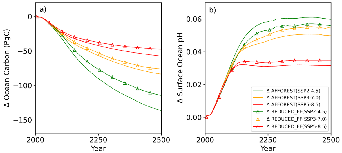
660 Figure 7. Changes in a) global total ocean carbon content and b) global mean surface ocean pH in the AFFOREST (solid lines; \Delta AFFOREST) and REDUCED_FF (solid lines with triangle markers; \Delta REDUCED_FF) cases relative to the FIXED_AGR case in the SSP-4.5 (green), SSP-7.0 (orange), and SSP-8.5 (red) scenarios. The AFFOREST and REDUCED_FF cases have smaller ocean carbon than the FIXED_AGR case in the three SSP scenarios because of the reduction of atmospheric CO 2 in the AFFOREST and REDUCED_FF cases by afforestation and reduced fossil 665 fuel emissions, respectively, and the consequent reduction in ocean carbon uptake. The AFFOREST and REDUCED_FF cases have larger surface ocean pH than the FIXED_AGR case because of the smaller ocean carbon content in the AFFOREST and REDUCED_FF cases.
