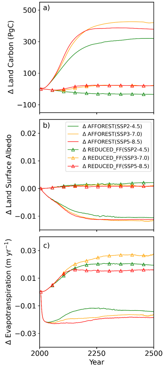
620 Figure 3. Changes in a) global total land carbon stock, b) land surface albedo and c) evapotranspiration in the AFFOREST (solid lines; \Delta AFFOREST) and REDUCED_FF (solid lines with triangle markers; \Delta REDUCED_FF) cases relative to the FIXED_AGR case in the SSP2-4.5 (green), SSP3-7.0 (orange) and SSP5-8.5 (red) scenarios. In the AFFOREST case, land carbon stock is larger than the FIXED_AGR case by 319.84 PgC, 418.93 PgC, and 379.21PgC in the SSP2-4.5, SSP3-7.0 and SSP5-8.5 scenarios by the year 2500, respectively, while the difference 625 between land carbon stock in REDUCED_FF and FIXED_AGR cases is nearly zero in the three SSP scenarios. The land surface albedo in the AFFOREST case is smaller by 0.011 (averaged over 2471-2500) in the three SSP scenarios compared to the FIXED_AGR case, while the REDUCED_FF case has a similar land surface albedo as in the FIXED_AGR case in the three SSP scenarios. The evapotranspiration is smaller (larger) in the AFFOREST (REDUCED_FF) case compared to the FIXED_AGR case due to changes in the water use efficiency of vegetation at 630 higher atmospheric CO 2 levels.
