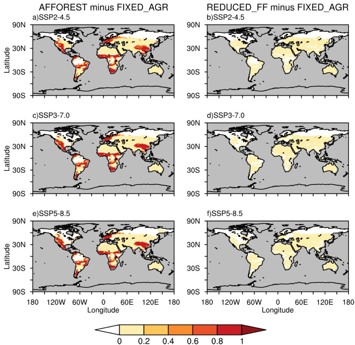
610 Figure 2. The left (right) panel shows the spatial pattern of the difference in tree fraction (averaged over 2471-2500) between the AFFOREST (REDUCED_FF) and FIXED_AGR cases. The top, middle, and bottom panels correspond to the SSP2-4.5, SSP3-7.0, and SSP5-8.5 scenarios, respectively. The tree fraction is higher in the AFFOREST case compared to the FIXED_AGR case regionally because of the regrowth of forests over the abandoned agricultural land after the year 2005, while the REDUCED_FF and FIXED_AGR cases have similar tree fraction in all regions.
