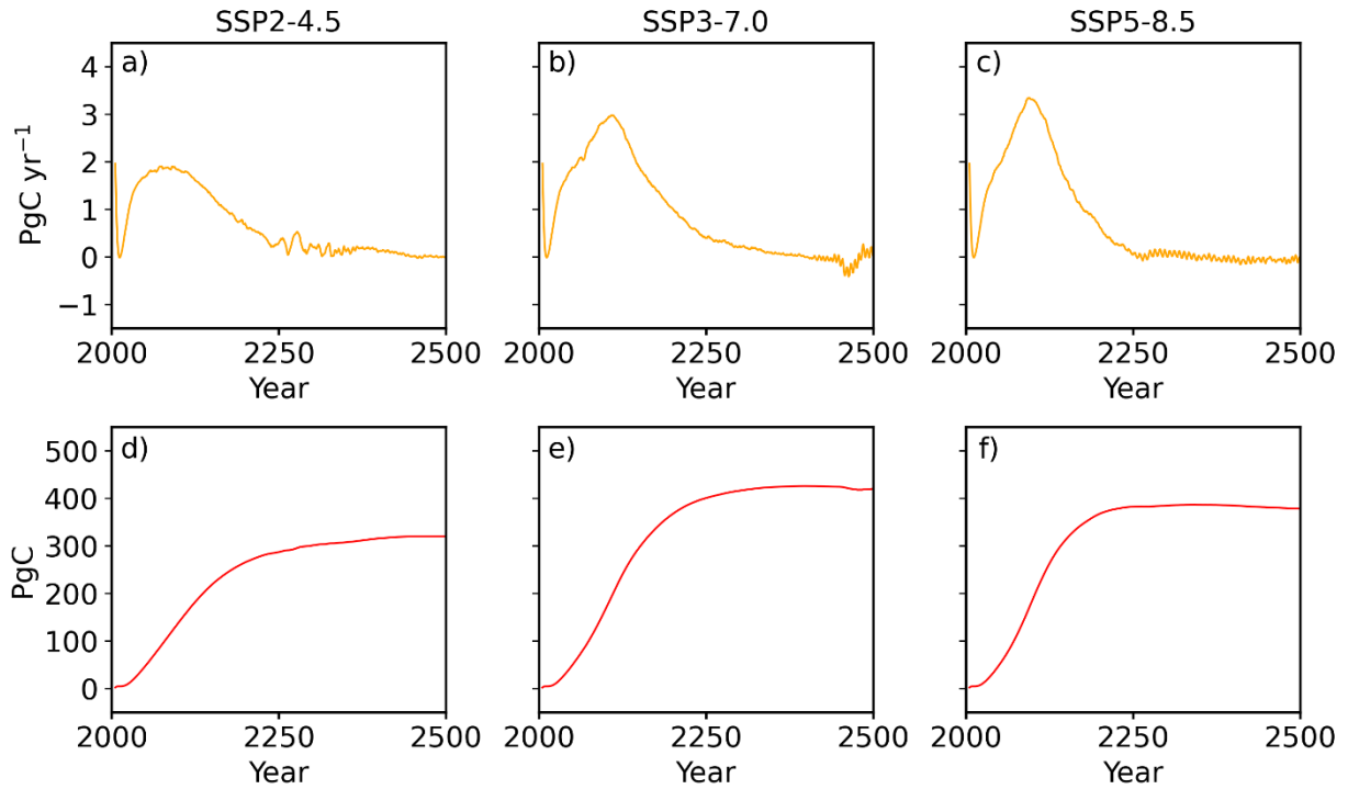
595 Figure 1. Top panels show the amount of carbon additionally stored in land each year in the AFFOREST case compared to the FIXED_AGR case in a) SSP2-4.5, b) SSP3-7.0 and c) SSP 5-8.5 scenarios, respectively. The bottom panels show the cumulative amount of additional carbon storage in land in the AFFOREST case compared to the FIXED_AGR case each year in d) SSP2-4.5, e) SSP 3-7.0 and f) SSP5-8.5 scenarios, respectively. In the AFFOREST simulations, the amount of carbon additionally stored in the land (between 2006-2500) compared to the FIXED_AGR case are 319.84 PgC, 418.93 PgC, and 379.21PgC in the SSP2-4.5, SSP3-7.0, and SSP 5-8.5 scenarios, respectively. 600 The initial peak in yearly additional carbon storage is due to the rapid growth of vegetation over abandoned agricultural land in the AFFOREST case. The second peak is due to the gradual increase in tree fraction in the AFFOREST case (Figure S5).
