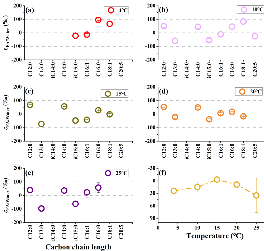
160 Figure 2. The hydrogen isotope composition of fatty acids in S. piezotolerans WP3 growing at different temperatures. (f) is the abundance-weighted mean \epsilon_{FA/Water} values at different temperatures. The error bars represent the 1 \sigma standard deviations of duplicate cultures. All cultures are not shaken.
