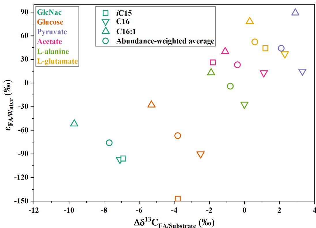
Figure 6. The values of carbon and hydrogen fractionation of fatty acids in S. piezotolerans WP3 growing on different organic substrates. The \Delta\delta^{13}\text{C}_{\text{FA/Substrate}} values are cited from Chen et al. (2022).
