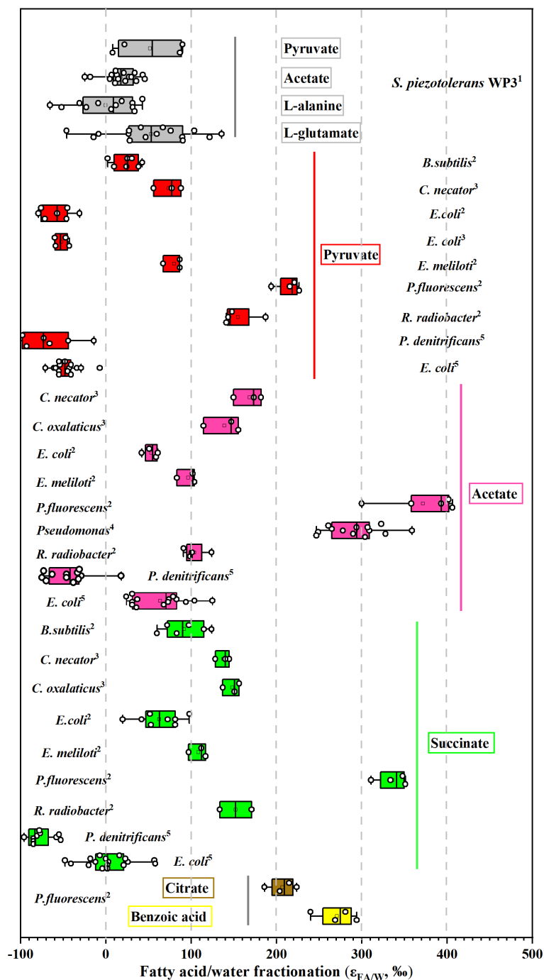
260 Figure 5. Compilation of measured hydrogen isotope fractionations growing on pyruvate and TCA cycle substrates. For each organism, bars represent the range of values for all individual fatty acids. The vertical line is the average value. Data sources: 1 This study; 2 Wijker et al. (2019); 3 Zhang et al. (2009a); 4,5 Heinzlmann et al. (2015 b).
