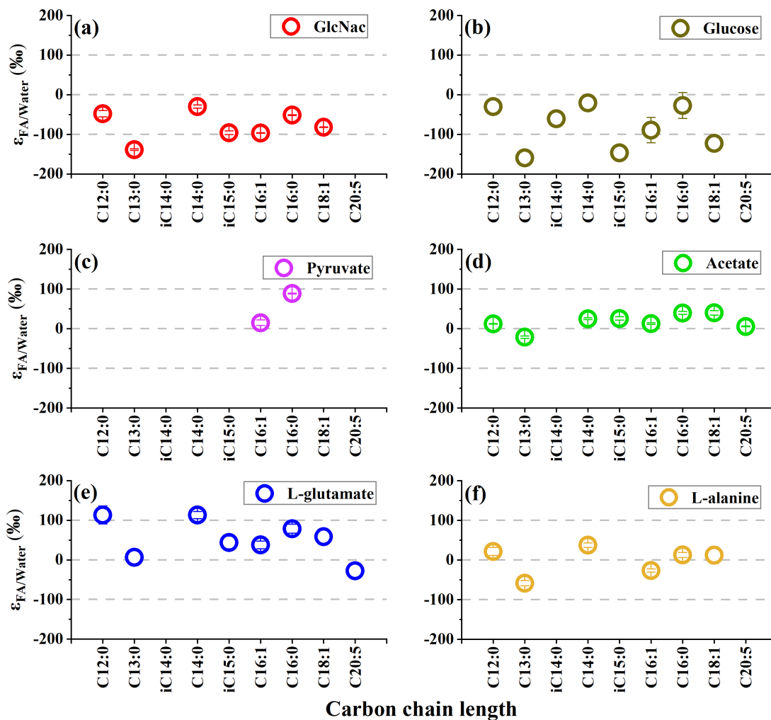
145 Figure 1. The hydrogen isotope fractionation between fatty acids and growth water in S. piezotolerans WP3 growing on different substrates including GlcNac, acetate, D-glucose, pyruvate and amino acids at 20 °C and shaking at 200 rpm. The error bars represent the 1σ standard deviations of duplicate cultures.
