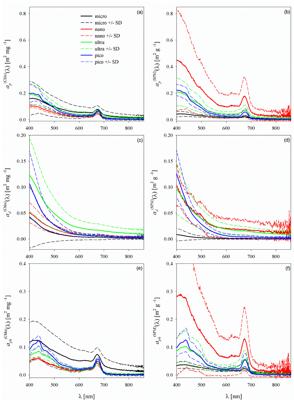
490 Figure 10: Mean chlorophyll-specific (left panel) and mass-specific (right panel) light absorption coefficients for all particles (a, b), detritus (c, d) and phytoplankton (e, f) for 4 size classes : micro-, nano-, ultra- and picoplankton. SD means standard deviation.
