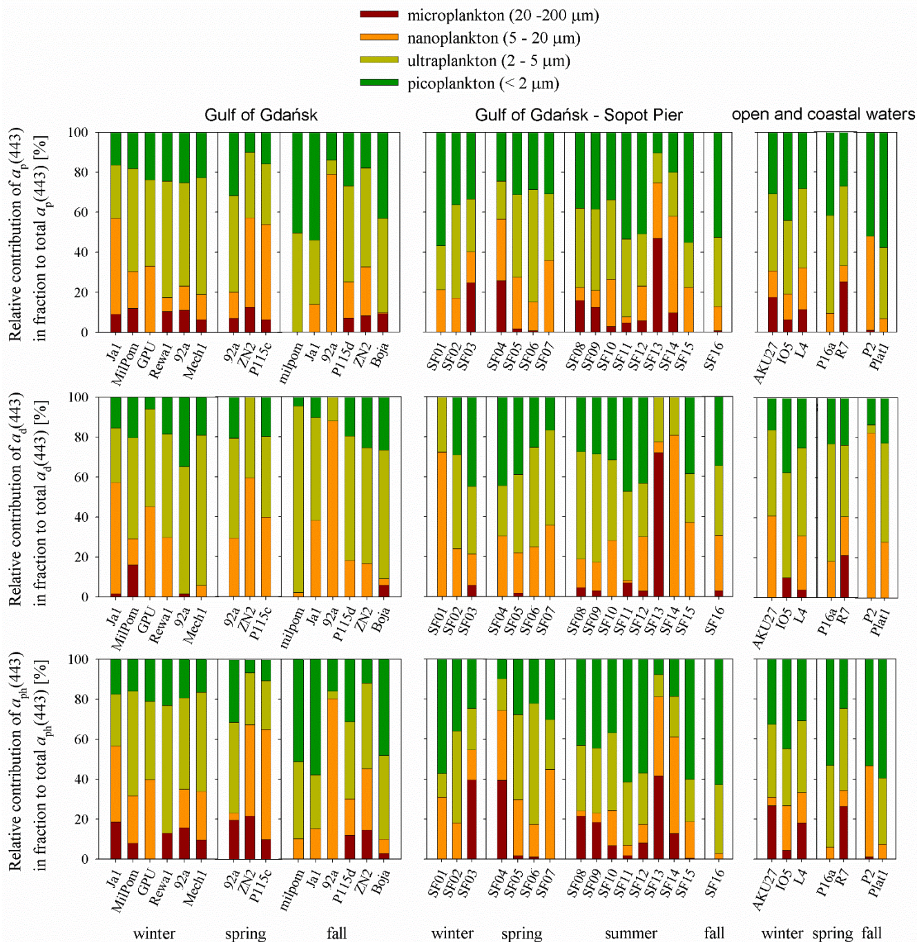
450 Figure 8: Contribution of particles from size classes in the total light absorption by all particles, detritus and phytoplankton according to the division into 4 size classes according to Ciotti et al. (2002) (micro-, nano-, ultra- and pico-particles) in GG, SF and OCW in for seasons
