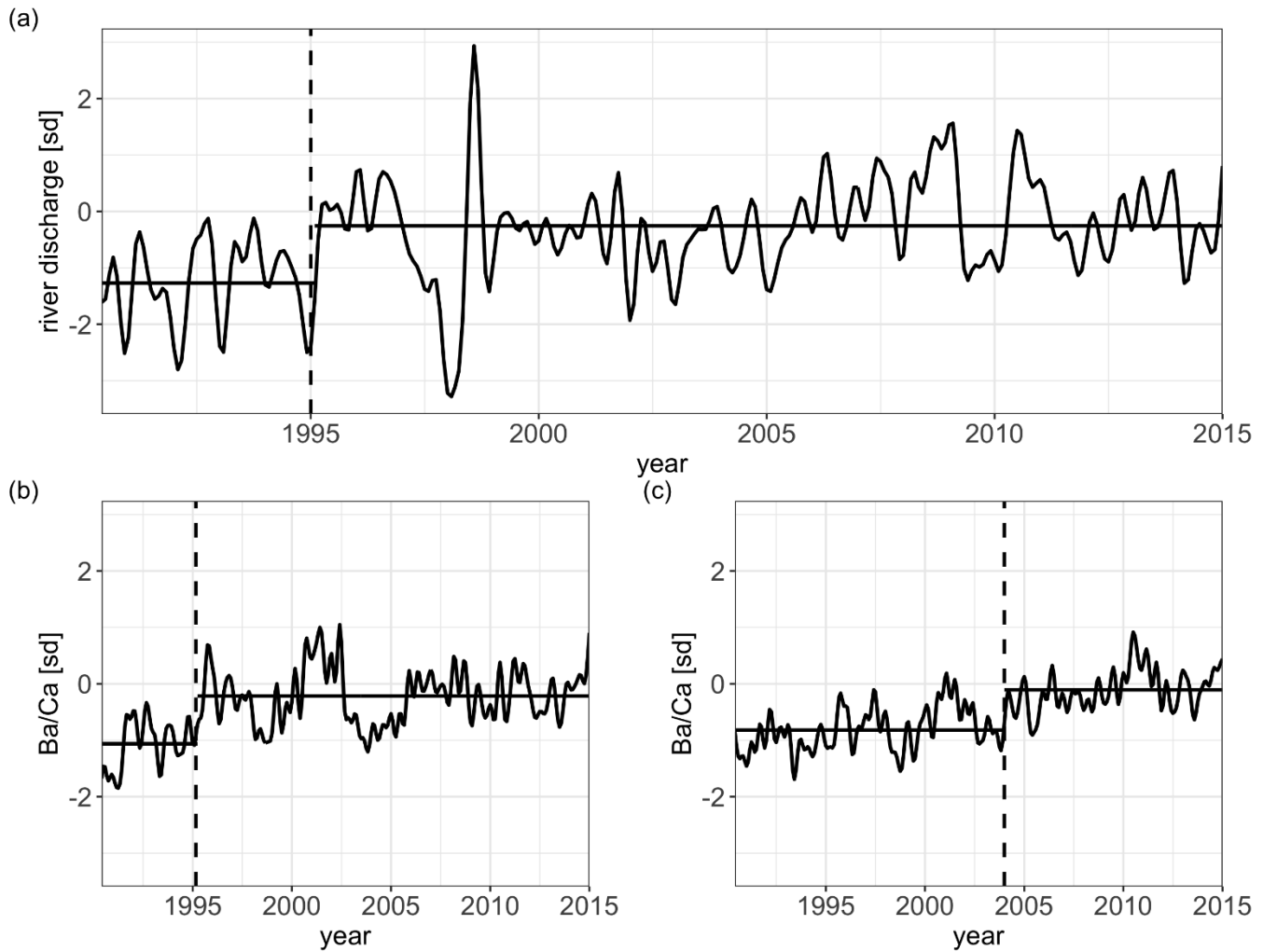
380 Figure 6: Change point analysis (MATLAB, Release 2022b) based on significant arithmetic mean change for (a) Marudi station's discharge as well as both composite records, (b) C1 and (c) C2.
