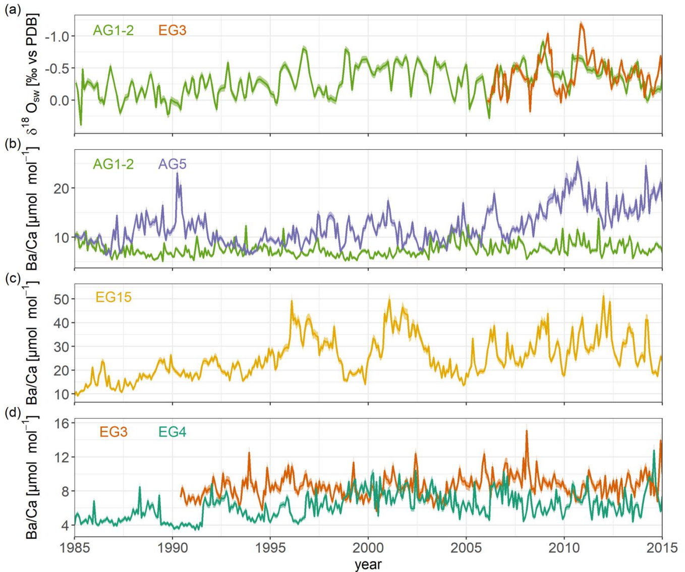
Figure 2: Monthly interpolated time series of (a) reconstructed \delta^{18}\text{O}_{\text{sw}} for Anemone's Garden 1 (AG1-2) in light green and Eve's Garden 3 (EG3) in orange (Krawczyk et al., 2020) and Ba/Ca ratios of (b) Anemone's Garden 1 and 5 (AG1-2 and AG5) in light green and blue, (c) Eve's Garden 15 (EG15) in yellow and (d) Eve's Garden 3 and 4 (EG3 and EG4) in orange and dark green, respectively, with shading indicating analytical error. Note that the y axis on the (a) panel is reversed.
