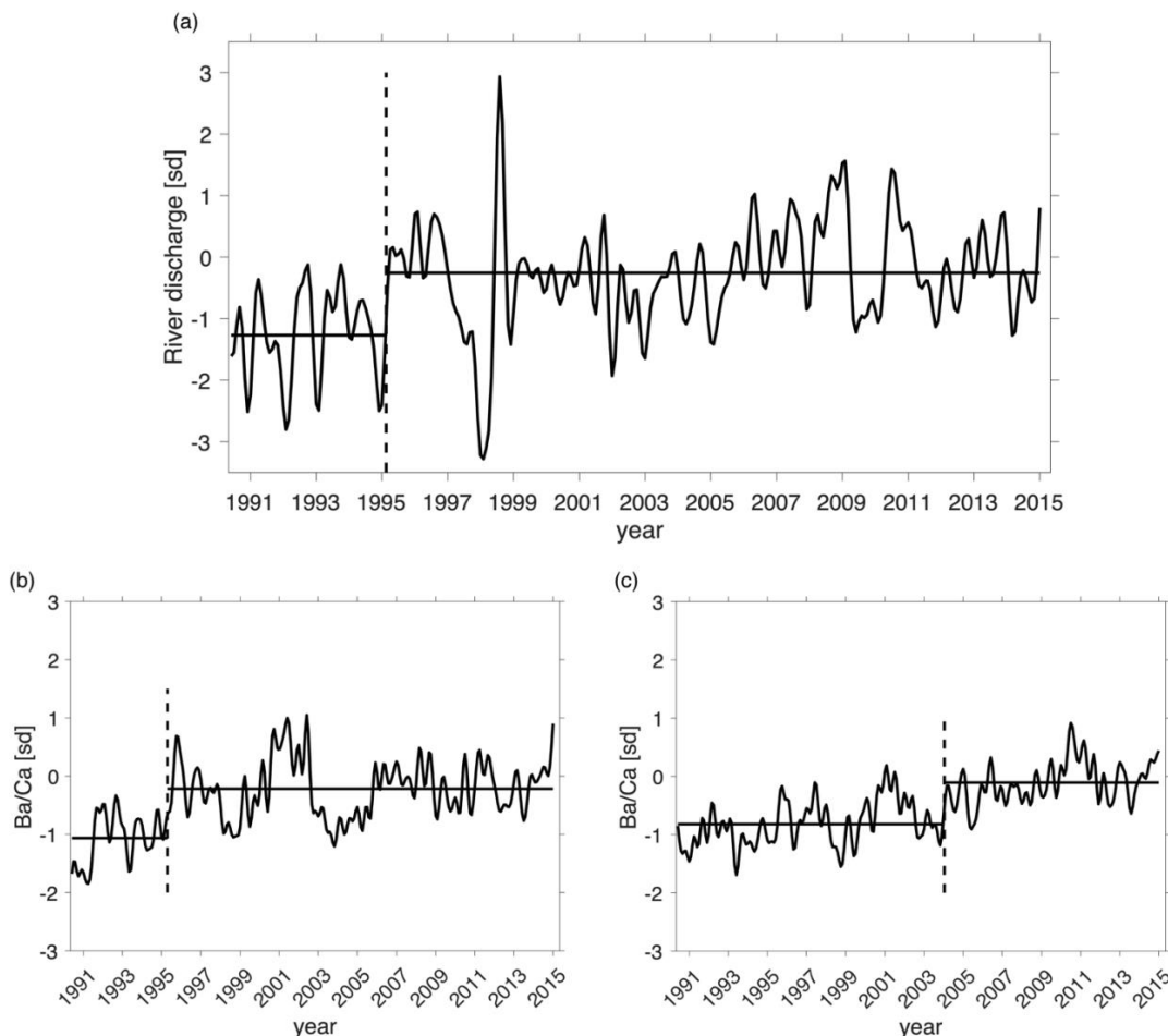
Figure 6: Change point analysis (MATLAB, Release 2022b) based on significant arithmetic mean change for (a) Marudi station's discharge as well as both composite records, (b) C1 and (c) C2.
