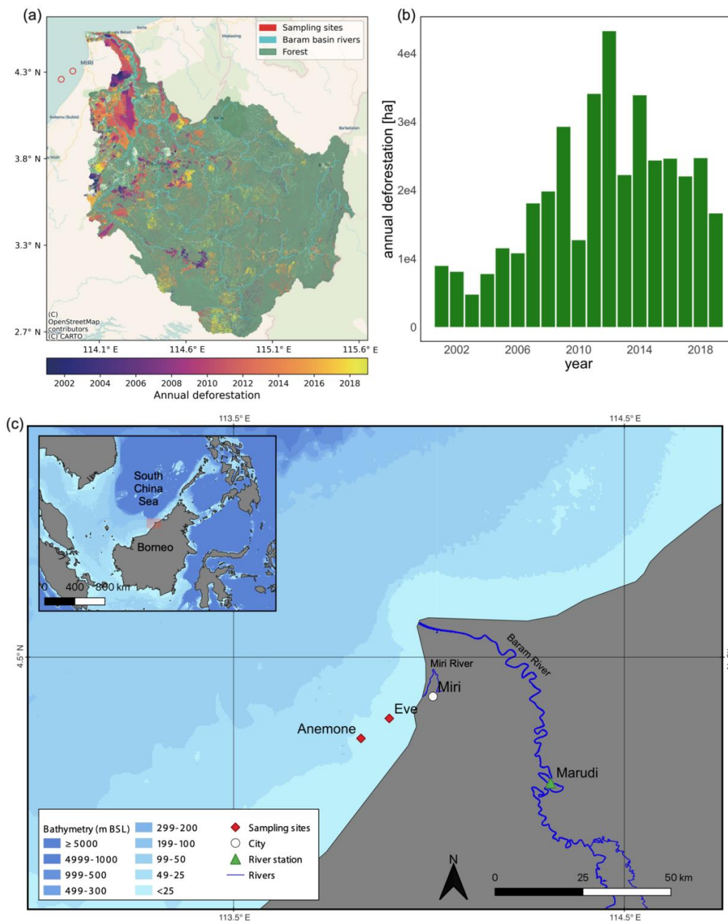
Figure 1: (a) Deforestation extent from 2001 to 2019 across the Baram River basin (map created on Python with annual deforestation data derived from the Global Forest Change dataset (Hansen et al., 2013)), © OpenStreetMap contributors 2022. Distributed under the Open Data Commons Open Database License (ODbL) v1.0”, (b) annual deforestation rate in the Baram River catchment in hectares between 2001 and 2019 and (c) map of the South China Sea and surrounding countries with an enlarged map of the study area both showing the bathymetry as well as the two sampling sites, Eve’s and Anemone’s Garden, the city of Miri, Miri River, and the Marudi station along the Baram River on the focused map. Map made on QGIS® (v. 3.22.0-Białowieża) using raster data from Natural Earth.
