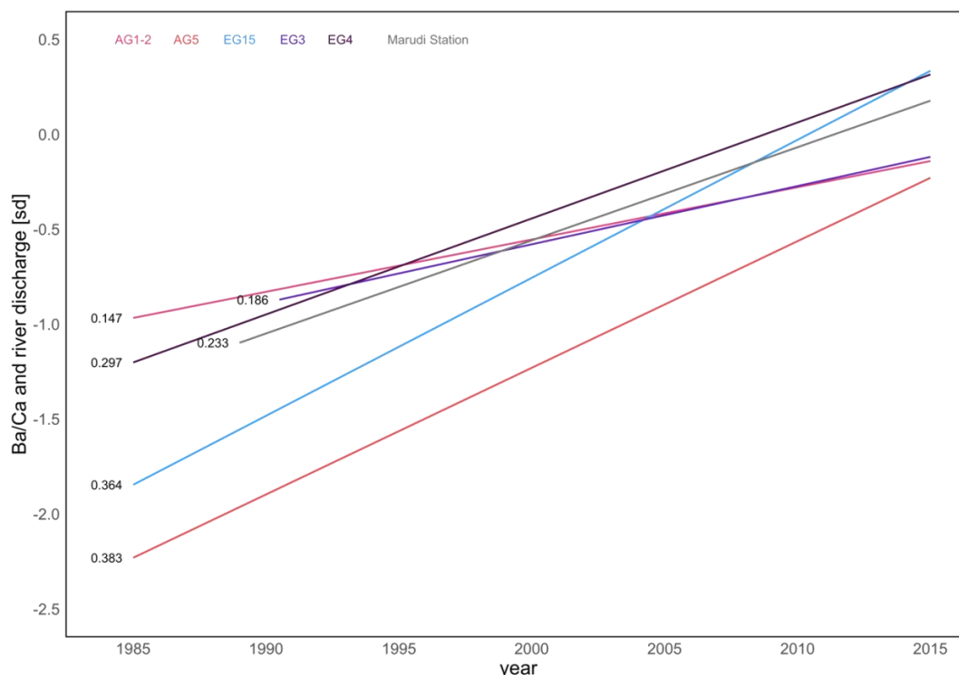
Figure 3: Trends in the Ba/Ca record of all five cores as well as river discharge using Sen's non-parametric method. The increasing trends are indicated by the Mann-Kendall tau-b statistic next to each record, all results are significant at the 0.05 level.
