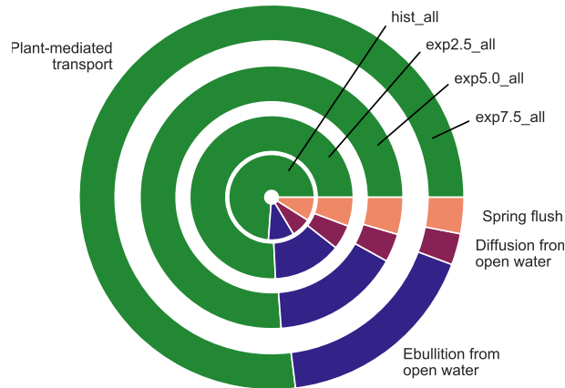
Figure 10. The contribution of each flux type to the overall emissions in the average year. The size of a segment represents the contribution of the respective flux type. The area of each circle is proportional to the absolute methane emissions of the average year in each simulation.
