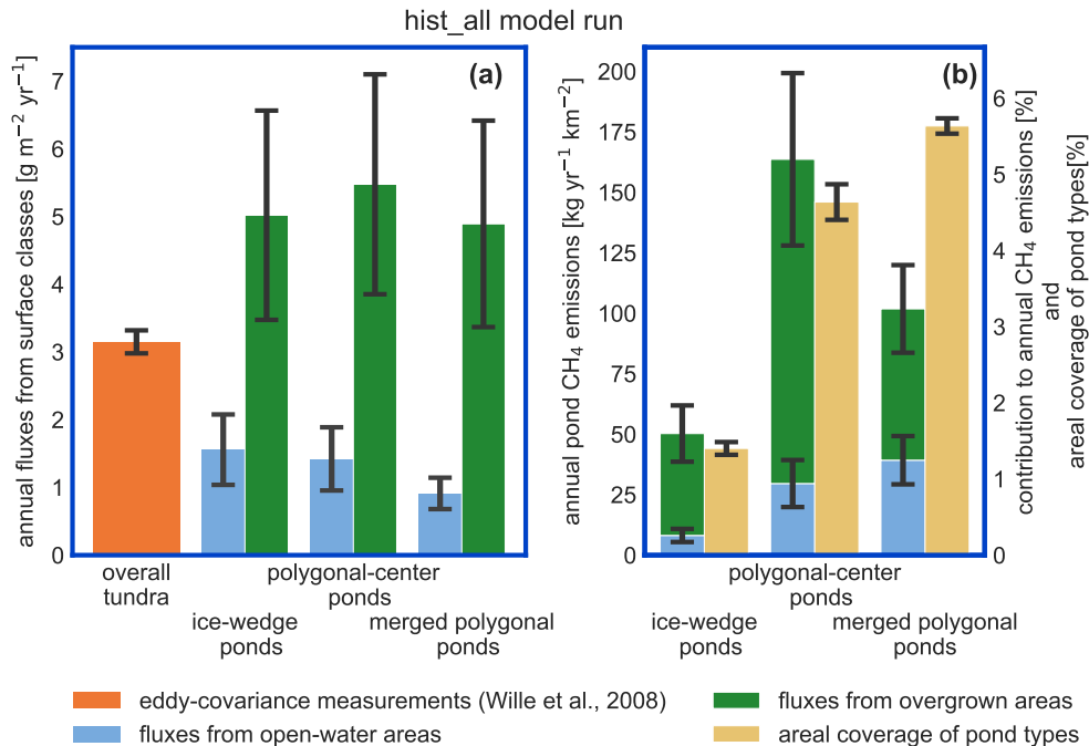
Figure 9. Impact of pond emissions on landscape methane emissions. (a) For the hist_all simulation, we compare fluxes from different landscape elements. The estimate for the overall tundra emissions (orange bar) were acquired with eddy-covariance measurements over the growing season of 2003 (Wille et al., 2008) and are shown for comparison. Note, that the influence of ponds on these measurements is low. The methane emissions per square meter of open and overgrown water are broken down per pond type. (b) Methane emissions per square kilometer of polygonal tundra of each pond type are displayed as stacked bars. We compare these emissions per pond type to the area this pond type covers in the polygonal tundra of Samoylov Island (sand-colored bar). This comparison relies on the assumption that the emissions measured by Wille et al. (2008) are representative for polygonal-tundra emissions.
