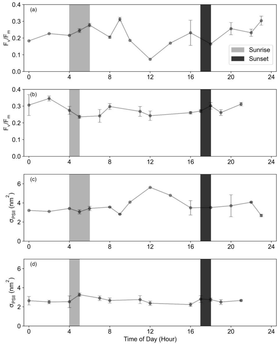
485 Figure A3. The diurnal cycle of (a,b) F_v/F_m for the (a) 6°E SIZ and (b) Astrid Ridge, and of (c,d) \sigma_{PSII} for the (c) 6°E SIZ and (d) Astrid Ridge, where the range of local sunrise and sunset times are indicated. Data were averaged together using the hour of the day, where error bars indicate standard deviation.
