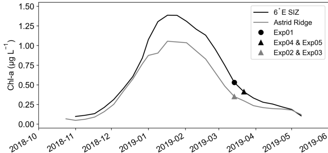
270 Figure 3. Satellite chlorophyll-a (Chl-a; \mu\text{g L}^{-1} ) data from OC-CCI from 01/10/2018 to 01/06/2019. The 6°E SIZ (62 – 72°S; 0 – 9°E) and Astrid Ridge (62 – 72°S; 9 – 16°E) were created from spatial means as indicated in the methods. The dates of the experimental set-ups are included for each region.
