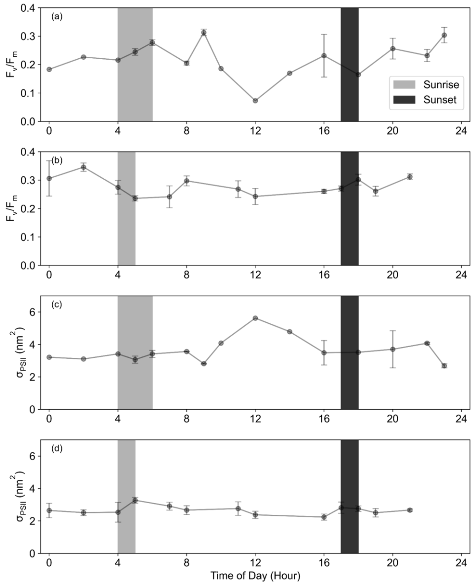
475 Figure A3. The diurnal cycle of (a,b) F_v/F_m for the (a) 6°E SIZ and (b) Astrid Ridge, and of (c,d) \sigma_{PSII} for the (c) 6°E SIZ and (d) Astrid Ridge, where the range of local sunrise and sunset times are indicated. Data were averaged together using the hour of the day, where error bars indicate standard deviation.
