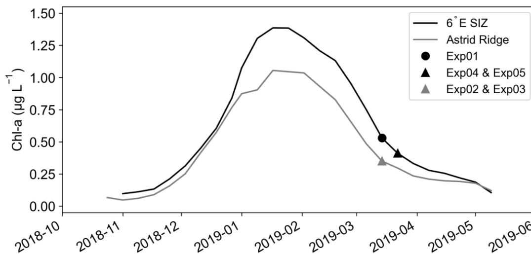
Figure 3. Satellite chlorophyll-a (Chl-a; \mu\text{g L}^{-1} ) data from OC-CCI from 01/10/2018 to 01/06/2019. The 6°E SIZ (62 – 72°S; 0 – 9°E) and Astrid Ridge (62 – 72°S; 9 – 16°E) were created from spatial means as indicated in the methods. The dates of the experimental set-ups are included for each region.
