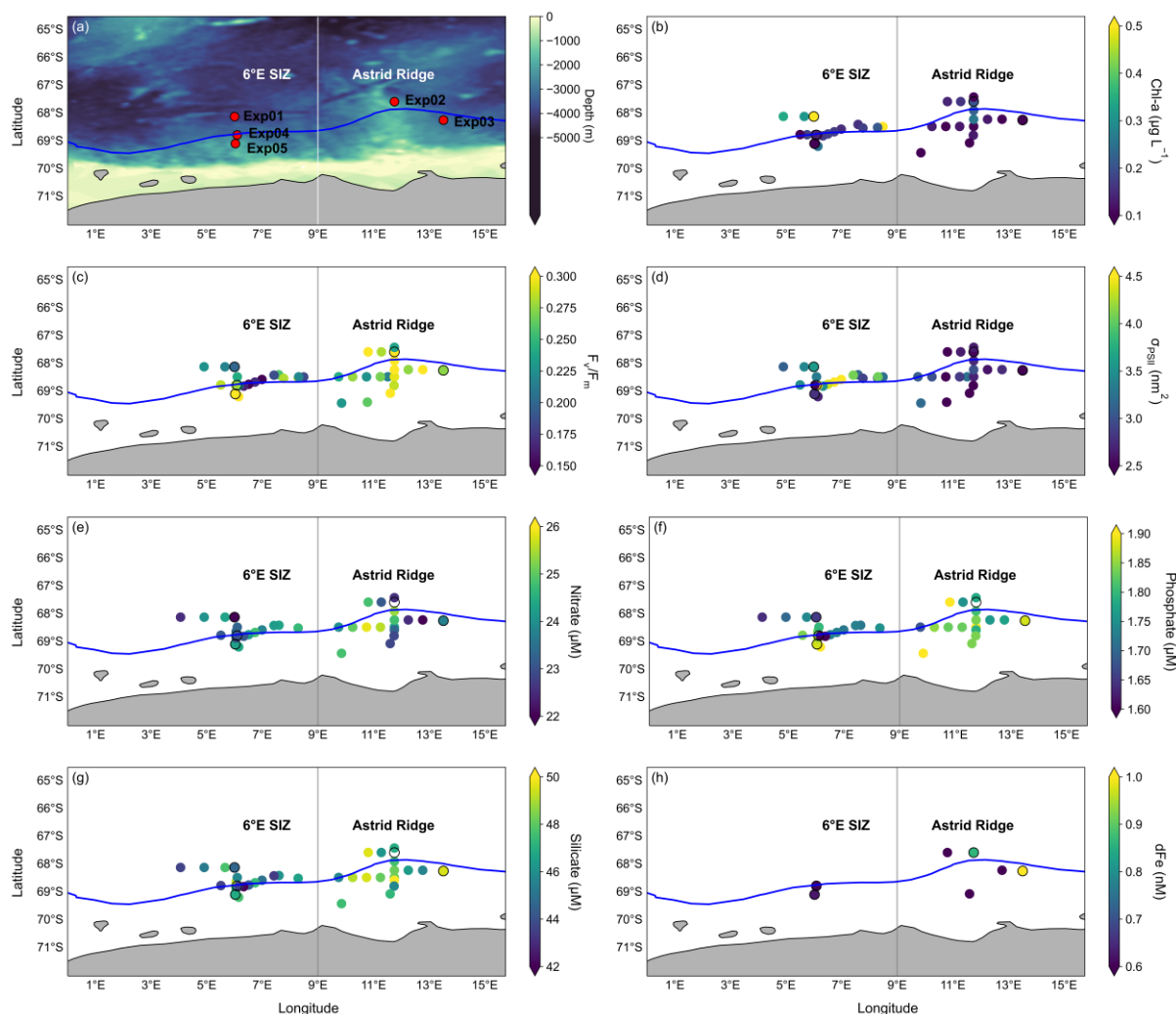
140 Figure 2. Initial conditions of the study region. Plots of (a) the overlaid bathymetry of the study region where the 6°E SIZ and Astrid Ridge region are indicated, along with the sampling locations for the incubation experiments (during March); and the associated mean initial parameters for (b) Chl-a concentrations ( \mu\text{g L}^{-1} ), (c) F_v/F_m , (d) \sigma_{PSII} ( \text{nm}^2 ), (e) Nitrate ( \mu\text{M} ), (f) Phosphate ( \mu\text{M} ), (g) Silicate ( \mu\text{M} ) and (h) dFe concentration (nM). The underway measurements, surface CTD data and the initial incubation measurements, all sampled within the study region in March, are collectively presented in (b-g) along with the average sea ice edge (concentration at 15% for March 2019 (blue line). Plot (h) shows the dFe concentrations which were sampled at all the Go-Flo stations. All data for incubation stations 145 are given in Table 1, and incubation stations are indicated by a black circle outline in (b-h).
