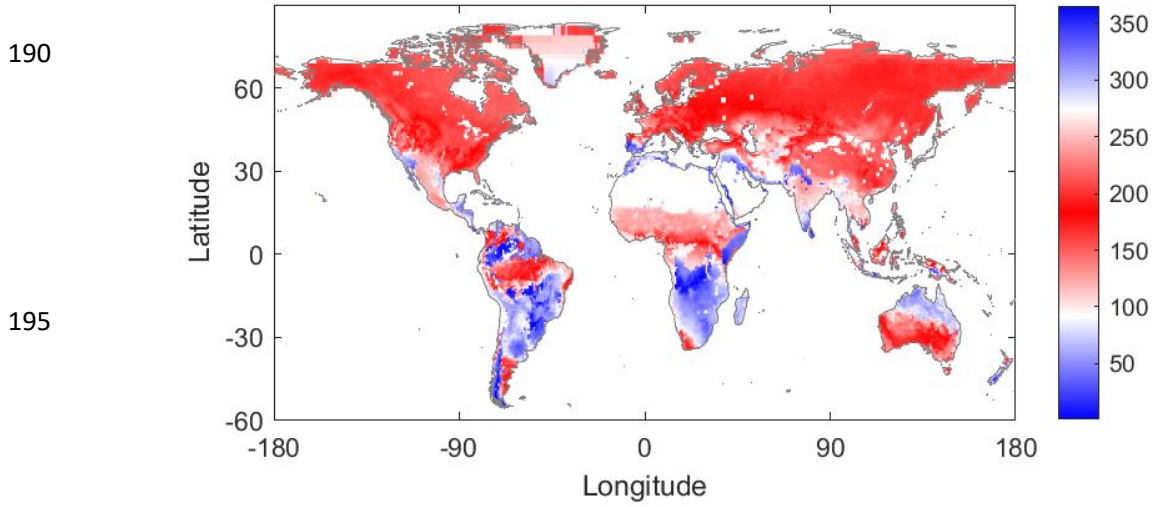
Figure 1: Growing season determination based on MODIS satellite normalized difference vegetation index (NDVI). Day of the year for the phenological peak based on MODIS NDVI climatology. White shading indicates NDVI was not available (bare-soil or water bodies).
