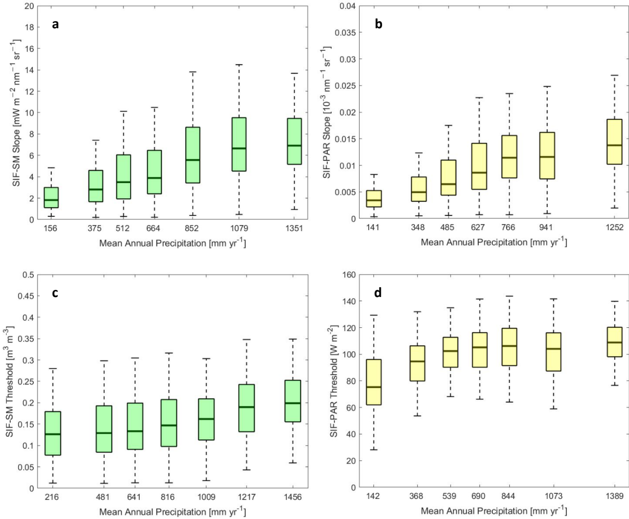
Figure 8: (a) SIF-SM slopes [\text{mW m}^{-2} \text{ nm}^{-1} \text{ sr}^{-1}] , (b) SIF-PAR slopes [10^{-3} \text{ nm}^{-1} \text{ sr}^{-1}] , (c) SIF-SM thresholds [\text{m}^3 \text{ m}^{-3}] and (d) SIF-PAR thresholds [\text{W m}^{-2}] binned as a function of mean annual precipitation [\text{mm yr}^{-1}] obtained from the GPM satellite constellation. Slope values correspond to sloped part of the two-regime model and the linear model (see Fig. 4). Each boxplot bin includes the same number of data points (915, 1548, 664 and 629 data points for boxplots (a), (b), (c), and (d), respectively). Box edges are the 25th and 75th percentiles of the distribution bounding the median (bold line), and whiskers extend to extrema (maximum and minimum). The median SIF-SM and SIF-PAR slopes and the median SIF-SM and SIF-PAR thresholds all increase with increasing mean annual precipitation.
