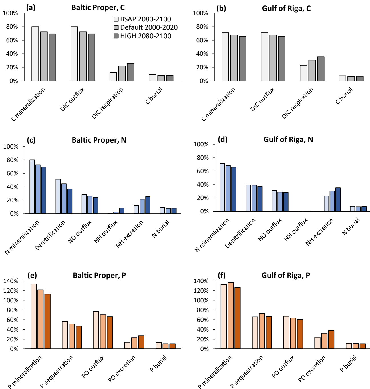
780 Figure 11. Apportionment of benthic fluxes of carbon (a, b), nitrogen (c, d) and phosphorus (e, f) in the default model run 2000-2020 and in two nutrient load scenarios 2080-2100 in the Baltic Proper (0–90 m depth, left column) and Gulf of Riga (right column). Fluxes are shown as percent of POM input to the sediment. Note that animal excretion is shown separately and not included in ‘mineralization’ or ‘outflux’.
