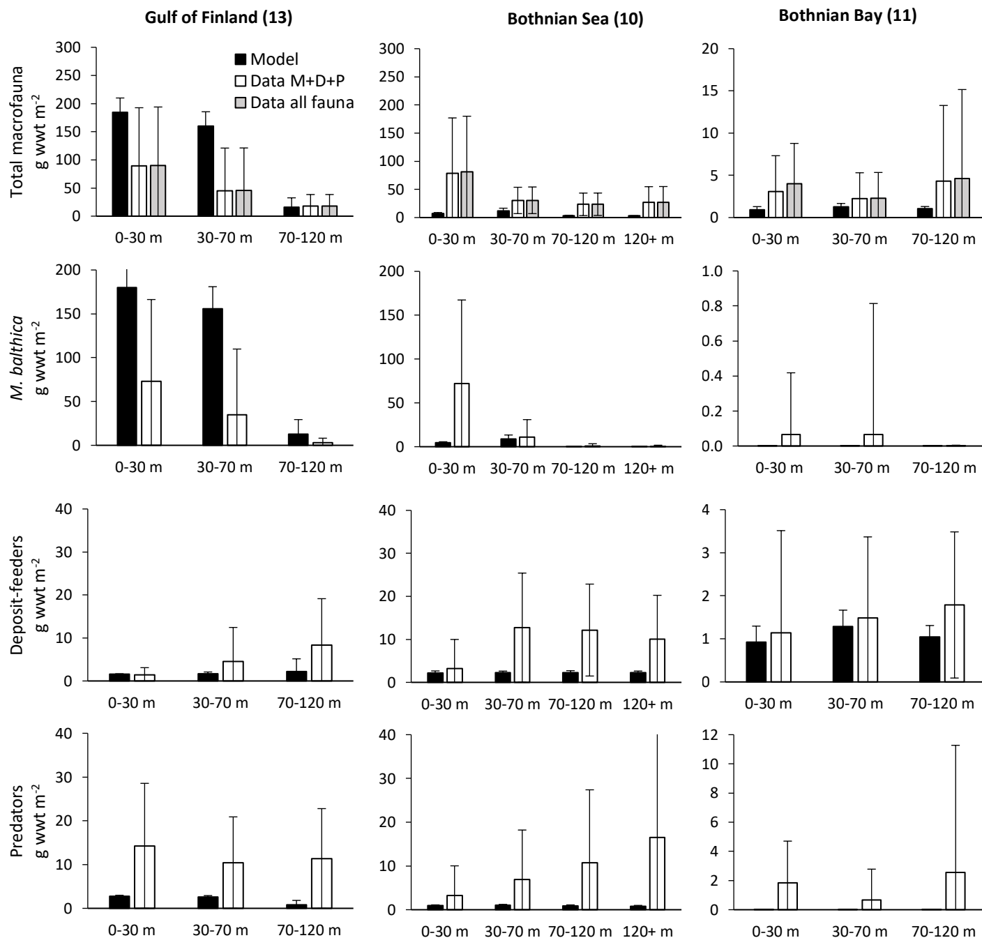
1025 Figure C2. continued. Note different scales on y-axes for the Bothnian Bay.
