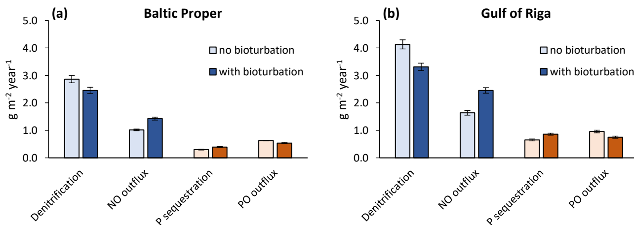
Figure 6. Immediate local effects of bioturbation on benthic fluxes. Benthic fluxes directly affected by bioturbation in the default run with bioturbation and when calculated for each time-step without bioturbation. Averages for 2000–2020 \pm standard deviations in the Baltic Proper (0–90 m depth, a) and Gulf of Riga (b). Note that ‘outflux’ refers to the flux from sediments to the water column without animal excretion.
