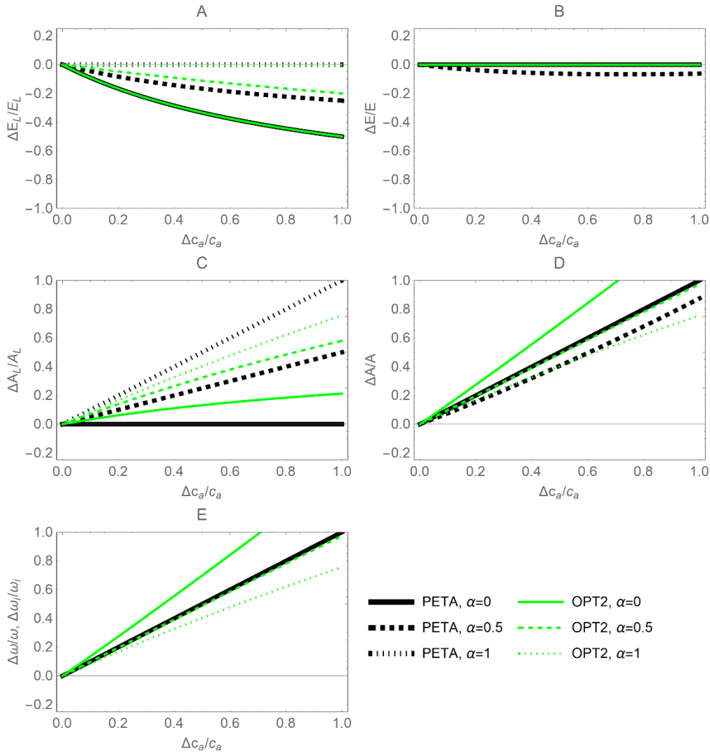
1185 Fig. 5. Relative changes in leaf-level (A, C) and canopy-level (B, D) gas exchange rates as a function of relative change in atmospheric CO 2 concentration c_a , as predicted by the PETA model (black lines) and the optimal stomatal control model OPT2 (green lines): A) leaf-level transpiration rate ( E_L ), B) canopy-level transpiration rate ( E ), C) leaf-level assimilation rate ( A_L ), D) canopy-level assimilation rate ( A ), and E) water use efficiency ( \omega , equivalent to intrinsic WUE at constant VPD). Changes in c_a have both direct and indirect effects on the CO 2 and water vapor exchange rates; the indirect effects are mediated by changes in leaf area that also depend on canopy status , indicated by \alpha (Fig. 3): lower values of \alpha refer to open-canopy conditions with largest leaf area stimulation by elevated c_a ; for \alpha = 1 leaf area is constant. Vapor pressure deficit and dry period length are equal to the baseline values (Table 2). 190
