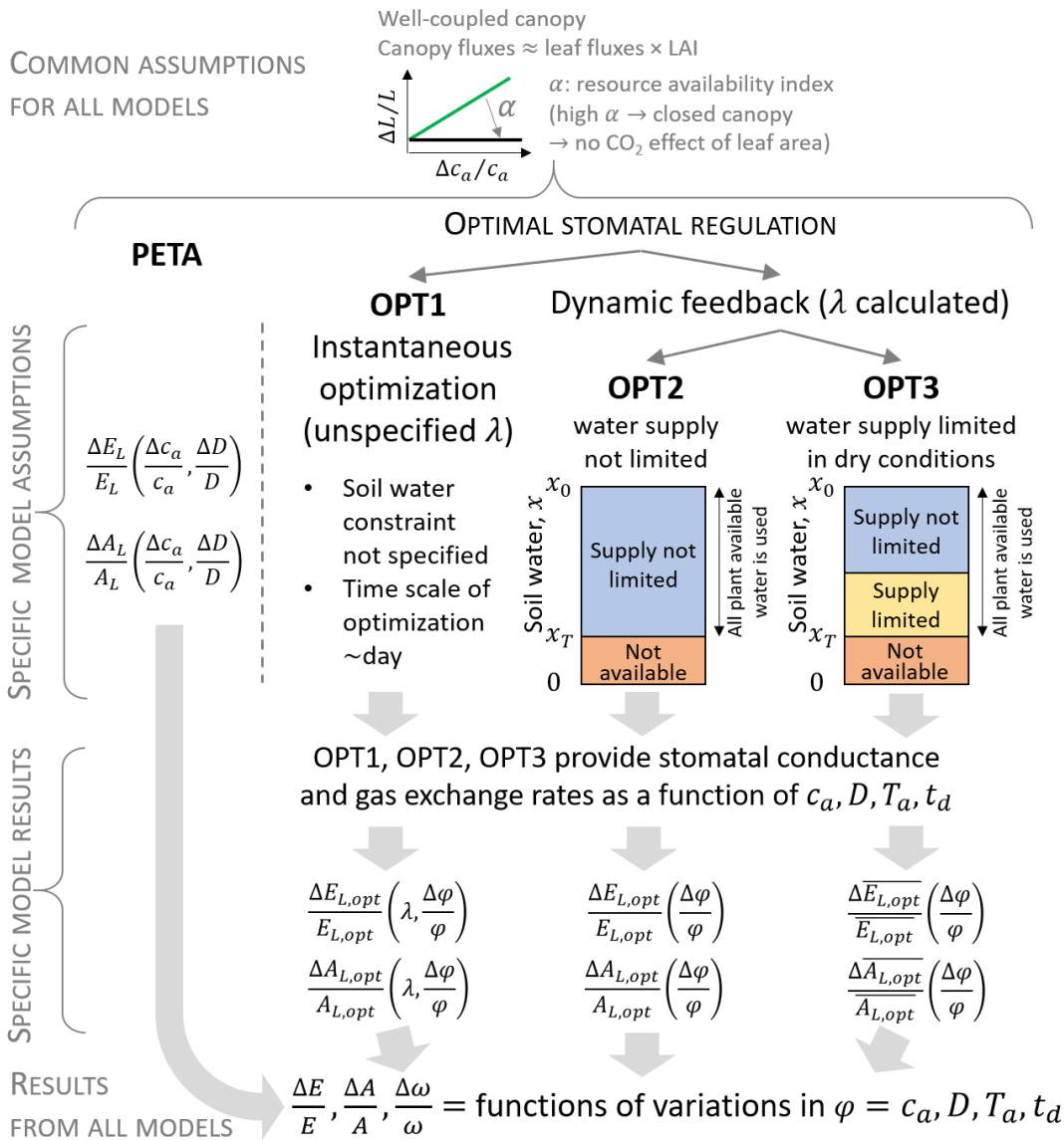
345 Fig. 1. Conceptual representation of the PETA and stomatal optimization models used to assess gas exchange responses (transpiration E and net \text{CO}_2 assimilation A ) to changes in atmospheric \text{CO}_2 concentrations c_a , vapor pressure deficit D (either independent of or caused by changes in air temperature T_a ), and length of a representative dry-down t_d (during which soil moisture x decreases from the initial value x_0 to x_T ). Three variants of the stomatal optimization model are considered: i) ‘instantaneous’ optimization (OPT1, where the marginal water use efficiency \lambda is unspecified), ii) ‘dynamic feedback’ optimization with no effect of water limitation in dry conditions (OPT2), and 350 iii) ‘dynamic feedback’ optimization including the effect of water limitation in the ‘supply limited’ regime (OPT3). In the heuristic PETA model, leaf-level gas exchange responses (subscript L ) follow from the empirical relation between water use efficiency ( \omega = A/E ) and c_a and D , whereas they are results of optimal stomatal regulation in the optimization models (subscript opt ). Overbar indicates temporal averaging during a representative dry-down period; 355 \varphi indicates a generic climatic variable ( c_a, D, T_a , or t_d ).
