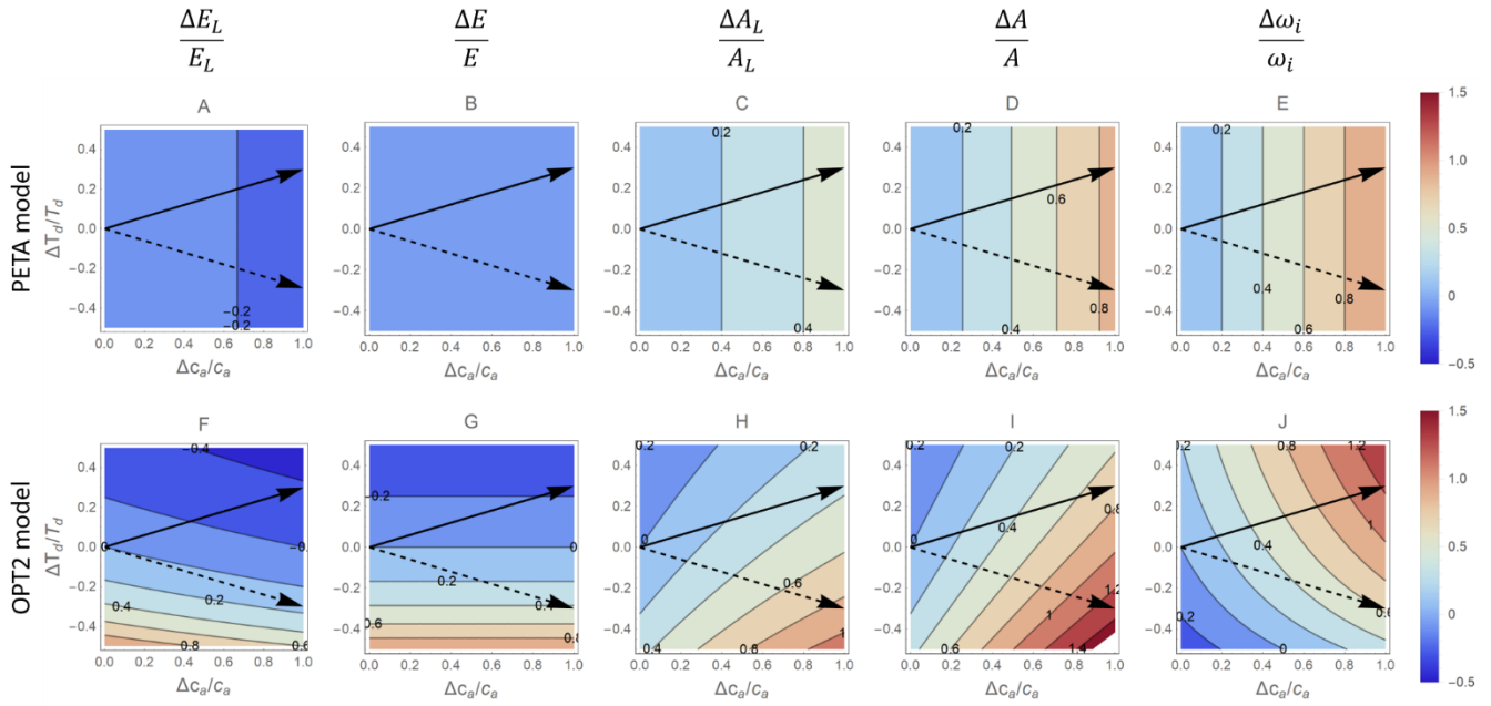
1265 Fig. 8. Contour plots of relative changes in leaf-level (A, C, F, H) and canopy-level (B, D, G, I) gas exchange rates as a | function of relative changes in atmospheric CO 2 concentration c_a (x-axis) and dry period length t_d (y-axis), as predicted by the PETA model (top panels) and the optimal stomatal control model OPT2 (bottom panels): A, F) leaf- level transpiration rate ( E_L ); B, G) canopy-level transpiration rate ( E ); C, H) leaf-level assimilation rate ( A_L ); D, I) 1270 canopy-level assimilation rate ( A ); and E, J) intrinsic water use efficiency ( \omega_i ). Leaf area index varies with c_a and D according to Eq. (7) with \alpha = 0.5 . Black arrows indicate hypothetical temporal trends in t_d and c_a in locations where t_d will lengthen (solid arrow) or shorten (dashed arrow) as c_a increases. The vapor pressure deficit is assumed to be constant and equal to the baseline value (Table 2).
