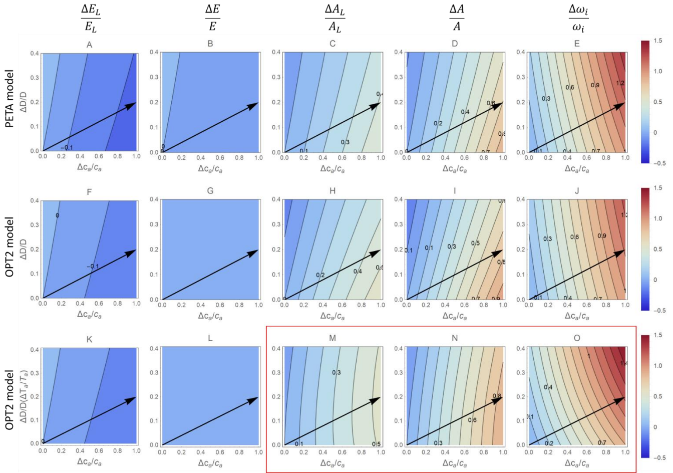
Fig. 6. Contour plots of relative changes in leaf-level (A, C, F, H, K, M) and canopy-level (B, D, G, I, L, N) gas exchange rates as a function of relative changes in atmospheric c_a (x-axis) and vapor pressure deficit D (y-axis), as predicted by the PETA model (top panels) and the optimal stomatal control model OPT2 (centre and bottom panels): A, F, K) leaf-level transpiration rate ( E_L ); B, G, L) canopy-level transpiration rate ( E ); C, H, M) leaf-level assimilation rate ( A_L ); D, I, N) canopy-level assimilation rate ( A ); and E, J, O) intrinsic water use efficiency ( \omega_i ). In F-J, D is varied by letting the relative humidity change at constant temperature T_a (i.e., the assimilation rate constants do not co-vary with D ); in K-O, D is varied by letting the T_a change at constant relative humidity, set at 50% (i.e., the assimilation rate constants co-vary with D due to the effect of T_a ). Leaf area index varies with c_a and D according to Eq. (7) with \alpha = 0.5 . Black arrows indicate hypothetical temporal trends in D and c_a assuming a \text{CO}_2 concentration doubling and associated D and T_a increase. The dry period length is assumed to be constant and equal to the baseline value (Table 2).
