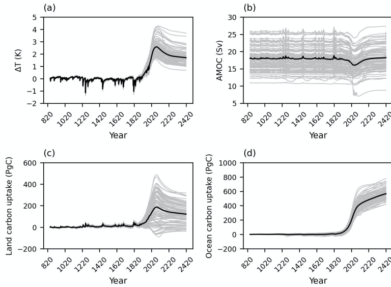
Figure 2: Inter-model spread of 86-member ensemble for change in (a) the surface air temperature, (b) Atlantic meridional overturning circulation (AMOC), (c) land carbon pool and (d) ocean carbon pool from year 850 CE until year 2420 following the SSP1-2.6 scenario. Black lines show the mean values.
