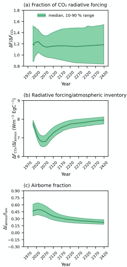
395 Figure 8: Radiative forcing dependence for the effective TCRE and its components in SSP1-2.6 scenario from year 2000. (a) Fractional radiative forcing contribution from atmospheric CO 2 , (b) dependence of the radiative forcing on atmospheric CO 2 and (c) airborne fraction. Solid lines show the median values, and shaded areas indicate the values between the 10 th and 90 th percentiles.
