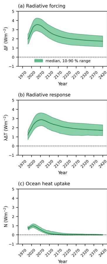
Figure 4: The evolution of (a) radiative forcing, (b) radiative response and (c) ocean heat uptake in SSP1-2.6 scenario from year 2000. Solid lines show the median values and shaded areas indicate the values between the 10 th and 90 th percentiles.
