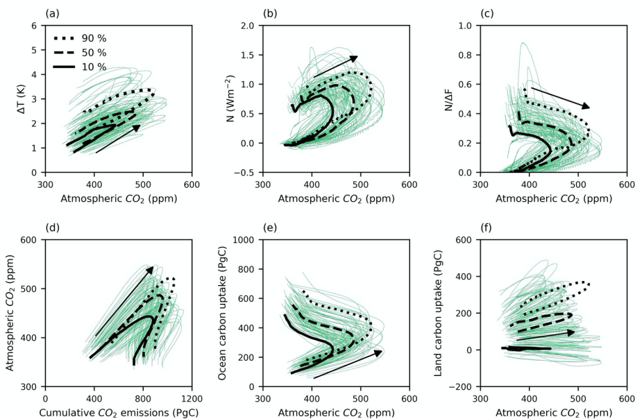
Figure 10: The thermal (upper row) and carbon (lower row) variables versus atmospheric CO 2 in SSP1-2.6 scenario from year 2000. (a) Change in surface air temperature; (b) ocean heat uptake; and (c) fraction of the radiative forcing warming the ocean interior; (d) cumulative CO 2 emissions; (e) change in the ocean carbon pool; and (f) change in the land carbon pool. In each panel the black lines show the median, 10 th and 90 th percentile values of the atmospheric CO 2 versus the median, 10 th and 90 th percentile values of the thermal and carbon variables.
