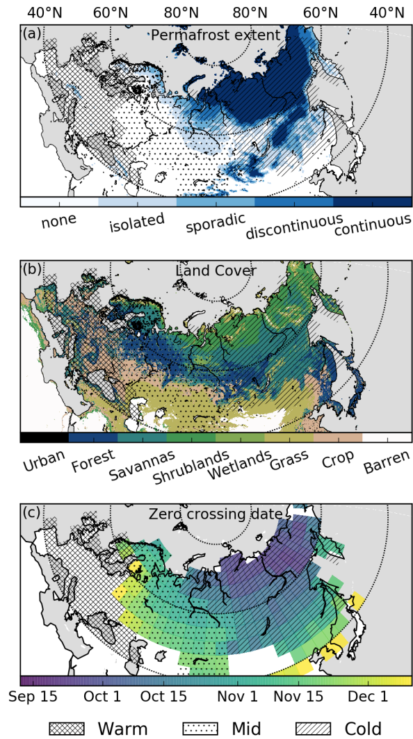
Figure 1. (a) Permafrost extent over 2000-2016 (Obu et al., 2019; Obu et al., 2018) (b) MODIS IGBP (MOD12C1 v6) land cover for urban areas, forest (tree cover >60% and height>2 m), savanna (tree cover 10–60% and height>2 m), shrublands (woody perennials cover >10% and height<2m), grasslands, croplands, and barren land. (c) zero-crossing date (date when the mean soil temperature drops below 0 °C) for the top 0.5 m of soil from the MERRA-2 Land dataset at 4° × 5° spatial resolution. Gridcells with no shading do not have a zero-crossing date. Three regions are shown by different hatching patterns. The “Warm” (cross hatching) region does not have a zero-crossing date, the “Mid” (dots) region has a zero-crossing date after Oct 27, and the “Cold” (diagonal hatching) region has a zero-crossing date before Oct 27. Note that some adjustments from these definition are made so that the regions are contiguous. The Warm, Mid, and Cold regions have land areas of 5.66 \times 10^6 km, 8.66 \times 10^6 km, and 12.65 \times 10^6 km, respectively.
