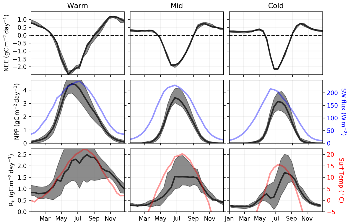
Figure 4. Data-driven four-year-mean (2015, 2016, 2018, and 2019) 14-day NEE, NPP, and R_h . (a-c) Median-mean and ensemble spread of NEE for the CMS-Flux 14day , TM4-4DVar 14day , and CAMS 14day flux inversions. (d-f) Median-mean and ensemble spread for the data-driven NPP. MERRA-2 Land net downward shortwave flux over land is shown in blue. (g-i) Ensemble estimate of R_h = NEE + NPP estimated from the three NEE and GPP estimates. MERRA-2 Land surface temperature is shown in red.
