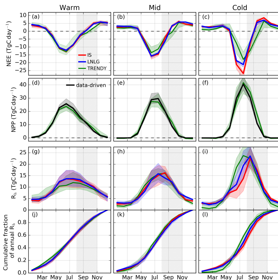
Figure 2. Monthly carbon cycle fluxes (average of 2015, 2016 and 2018; 2017 is excluded due to an OCO-2 data gap). (a-c) Median (solid line) and interquartile range (shaded area) of NEE for the ensemble of IS (red) and LNLG (blue) OCO-2 MIPv9 and for the TRENDY ensemble (green). (d-f) NPP for the TRENDY ensemble (green) and estimated from data-driven GPP (black). (g-i) R_h simulated by the TRENDY ensemble (green) and calculated from combining the data-driven GPP with the IS (red) and LNLG (blue) OCO-2 MIPv9 NEE constraints. (j-l) Cumulative fraction of R_h over the growing season. Figure S7 shows these fluxes per unit area.
