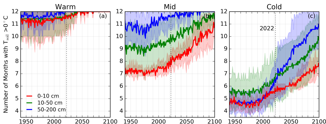
Figure 5. Number of months per year with monthly mean soil temperatures above 0^{\circ}\text{C} at depths of 0–10 cm (red), 10–50 cm (green), and 50–200 cm (blue) simulated by seven CMIP6 models under ssp585 for the (a) Warm, (b) Mid, and (c) Cold regions. The solid lines show the model mean and shading shows \pm 1 standard deviation.
