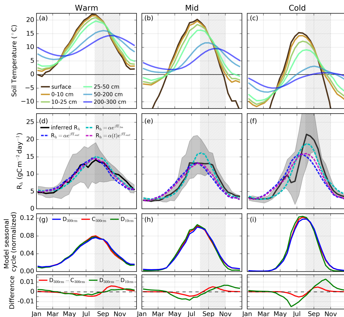
Figure 4. Impact of temporal and vertical variations in carbon pools on R_h . (a-c) MERRA-2 Land soil temperature over five intervals for the (a) Warm, (b) Mid, and (c) Cold regions. (d-e) Median and range in inferred 14-day R_h with fits for single-layer R_h models that employ (navy dash) T_{\text{surf}} dependence and no seasonal variations in the carbon pool, (cyan dash) T_{1m} dependence and no seasonal variations in the carbon pool and (magenta dash) T_{\text{surf}} dependence and seasonal variations in the carbon pool. (g-i, top) Normalized seasonal cycle of R_h simulated for D_{300\text{cm}} (dynamic carbon pool over 0-300 cm depth), C_{300\text{cm}} (constant carbon pool over 0-300 cm depth), D_{10\text{cm}} (dynamic carbon pool over 0-10 cm depth) and (g-i, bottom) the difference in simulated R_h .
