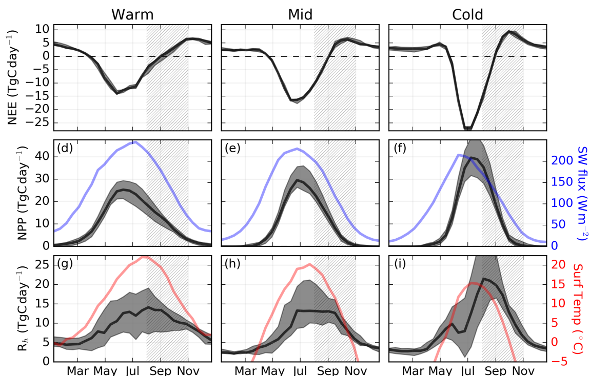
Figure 3. Data-driven four-year-mean (2015, 2016, 2018, and 2019) 14-day NEE, NPP, and Rh. (a-c) Median and ensemble spread of NEE for the CMS-Flux 14day , TM4-4DVar 14day , and CAMS 14day flux inversions. (d-f) Median and ensemble spread for the data-driven NPP. MERRA-2 Land net downward shortwave flux over land is shown in blue. (g-i) Ensemble estimate of R_h = NEE + NPP estimated from the three NEE and GPP estimates. MERRA-2 Land surface temperature is shown in red.
