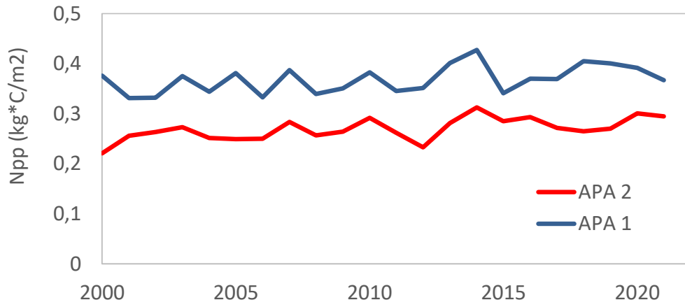
Figure RC3.1: Primary production from MODIS satellite data (2000-2021) for the study area.
