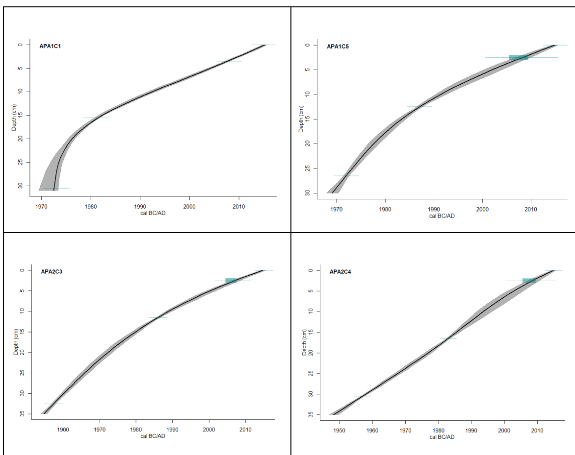
Figure RC4.3: New age models.
