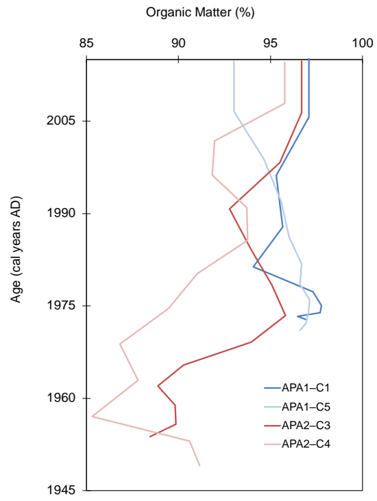
Figure RC4.4: Organic matter content (%) for the 4 cores.
