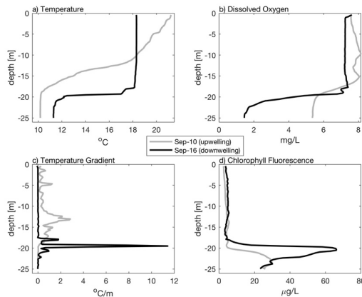
Figure 4: Vertical profiles from the mid-shelf ( \sim 41.82^\circ \text{N} ) collected during late summer 2020 including a) temperature, b) dissolved oxygen, c) vertical temperature gradient, and d) chlorophyll fluorescence highlighting the difference following upwelling (Sept-10 grey line) and downwelling (Sept-16 black line) conditions. Note that even though the top-to-bottom temperature difference is greater following upwelling, downwelling results in a stronger temperature gradient, thinner bottom boundary layer, lower dissolved oxygen and higher sub-surface chlorophyll fluorescence.
