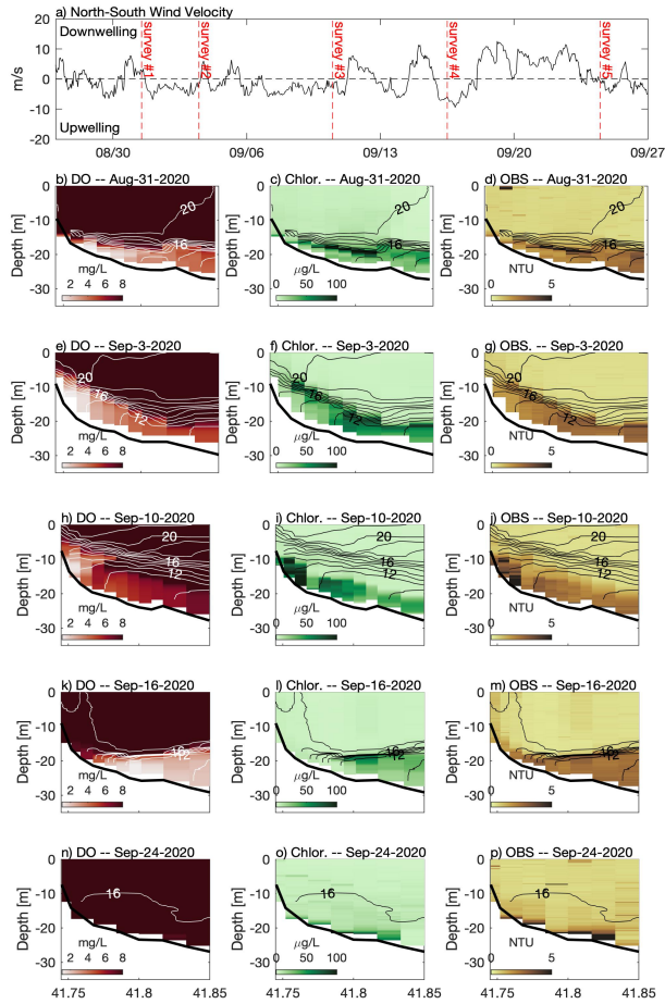
Figure 3: a) North-South component of wind measured at NDBC buoy 44013 . Panels on the left (b,e,h,k,n) show across-shelf transects of dissolved oxygen, panels in the centre (c,f,i,l,o) show chlorophyll fluorescence and panels on the right (d,g,j,m,p) show optical backscatter measured during a series of cruises in late summer 2020. For each transect, temperature contours (1°C interval) are shown. In the top panel the vertical red dashed lines indicate the approximate timing of each cruise. Note that Aug. 31 and Sept. 16 followed downwelling winds (positive) and Sept. 3 and 10 were during a period of prolonged upwelling-favourable winds (negative). See figure 1 for location of transect and wind measurements.
