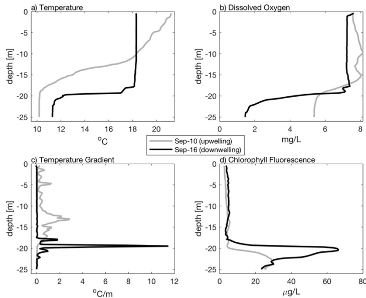
Figure 4: Vertical profiles from the mid-shelf ( \sim 41.82^{\circ}\text{N} ) collected during late summer 2020 including a) temperature, b) dissolved oxygen, c) vertical temperature gradient, and d) chlorophyll fluorescence highlighting the difference following upwelling (Sept-10 grey line) and downwelling (Sept-16 black line) conditions. Note that even though the top-to-bottom temperature difference is greater following upwelling, downwelling results in a stronger temperature gradient, thinner bottom boundary layer, lower dissolved oxygen and higher sub-surface chlorophyll fluorescence.
