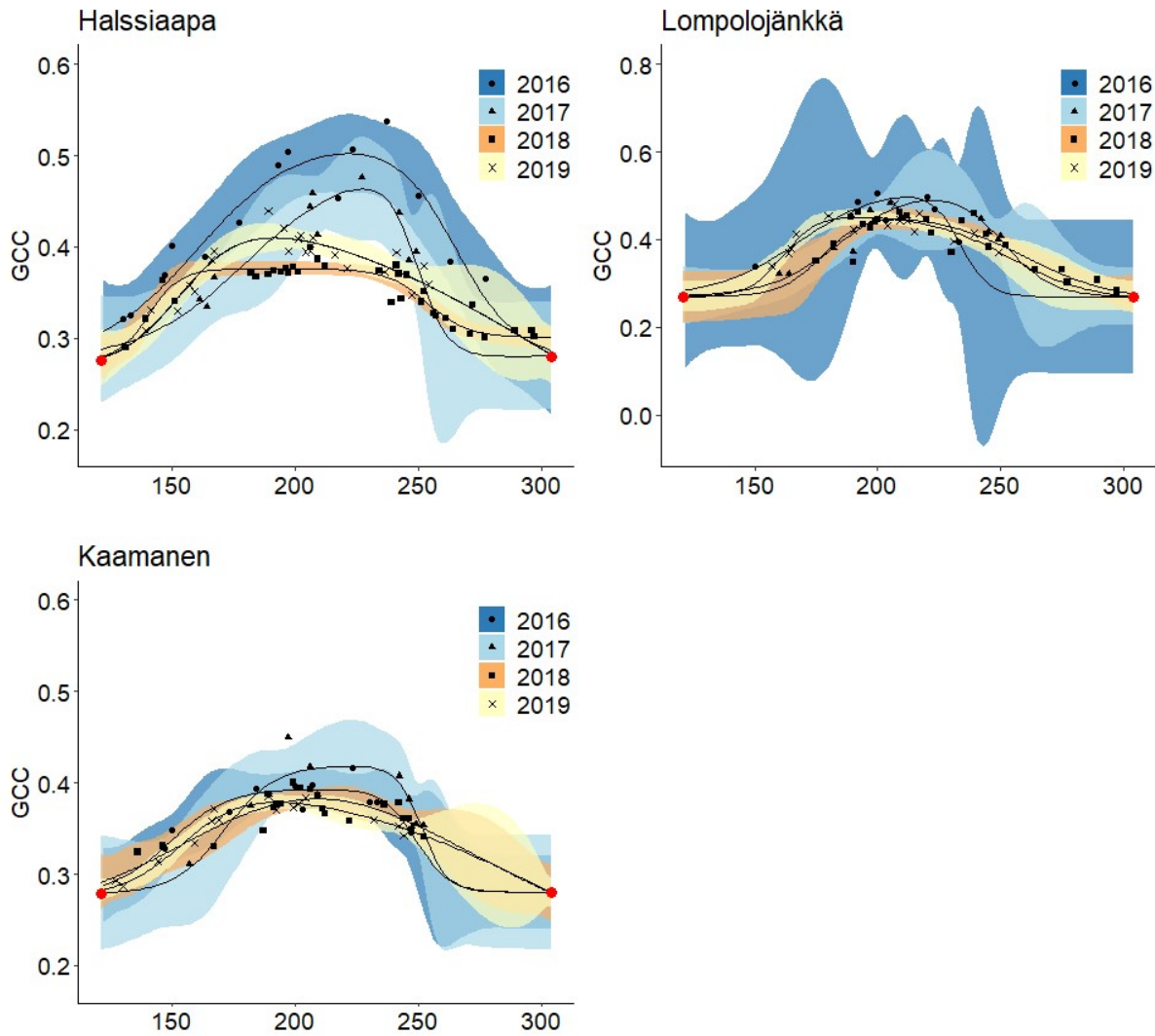
370 Figure 98: Mean GCC derived from the Sentinel-2 data from 1 May to 30 September in 2016–2019 at Halssiaapa, Lompolojänkkä and Kaamanen. Different symbols and colours denote different years, and the bands show the 95% confidence intervals of the fitted double hyperbolic tangent function. The red dots indicate the fixed start and end days defined for the fitting. Note the different y-axis scaling for Lompolojänkkä.
