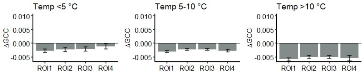
Figure S8: Mean three-day difference in GCC divided to temperature classes (<5 °C, 5-10 °C, >10 °C) at Lompolojännkä from May to September. No temperature data in the <5 °C class in August. The error bars denote the standard error.
