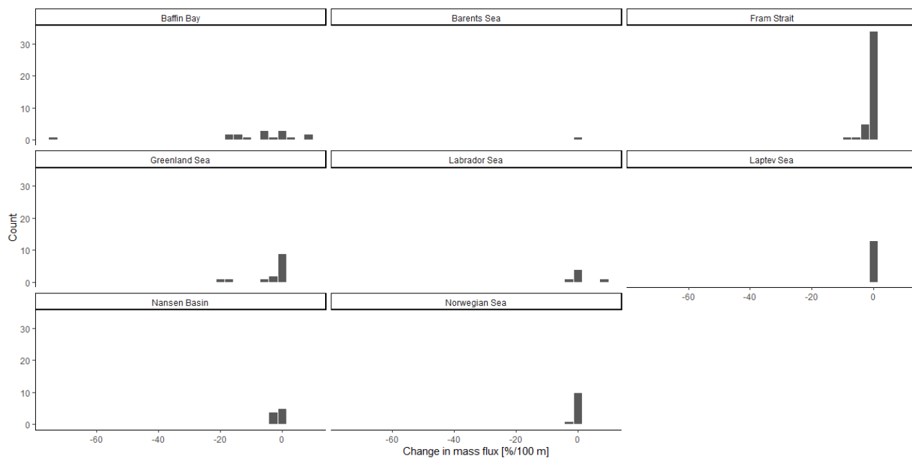
Figure A3: Loss in shell flux between the net directly below the calculated base of the productive zone and the deepest net of sampling of each station, divided by the different regions of sampling.
