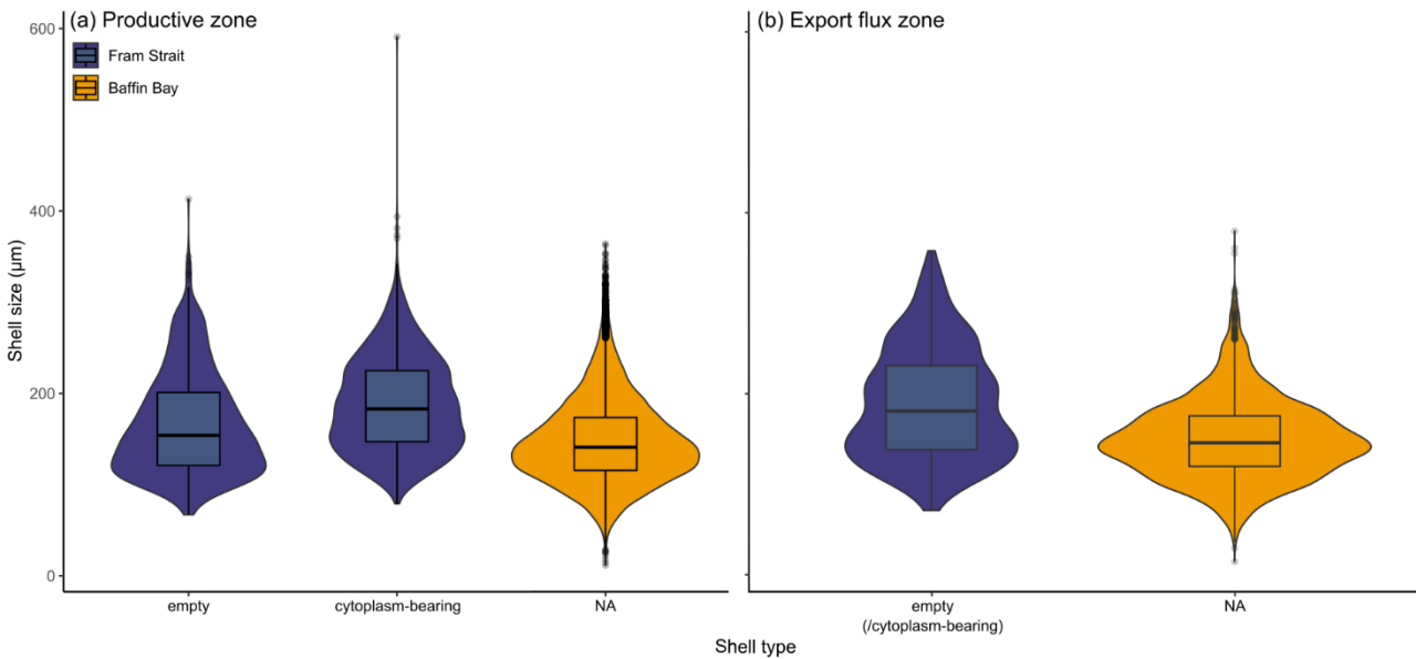
Figure 4: Overview on shell sizes of N. pachyderma from the Fram Strait (blue) and the Baffin Bay (orange), contrasting empty, cytoplasm-bearing and non-determined shells (NA) (a) within the productive zone, and (b) in the export flux zone. Shell types are not distinguished in (b) as we assume all shells collected below the productive zone to represent specimens that were dead during retrieval (denoted as empty (/cytoplasm-bearing)).
