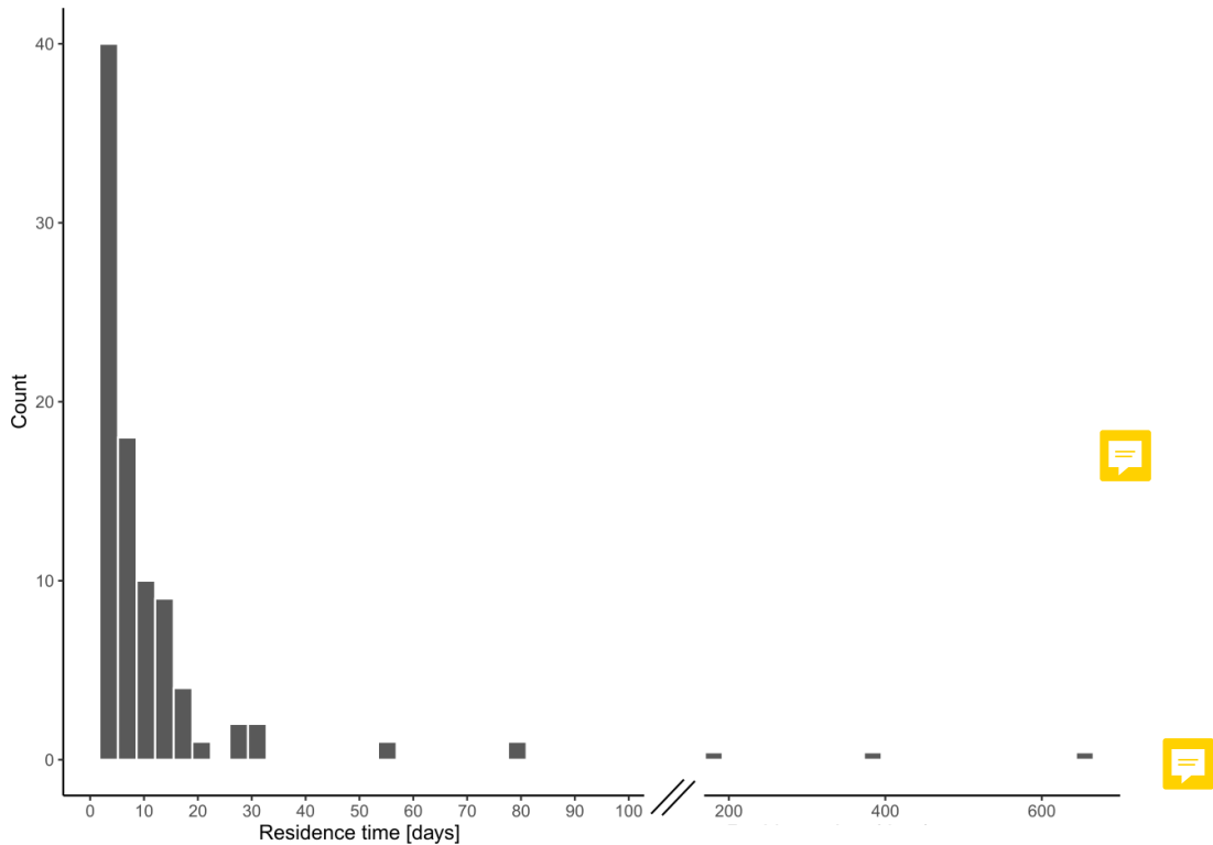
370 Figure 12: Residence Time of N. pachyderma within the productive zone in days, calculated based on the standing stock within the productive zone and the shell flux below the base of the productive zone, calculated with average shall masses below the productive zone. Consider the break in the x-axis between 100 and 200 days.
