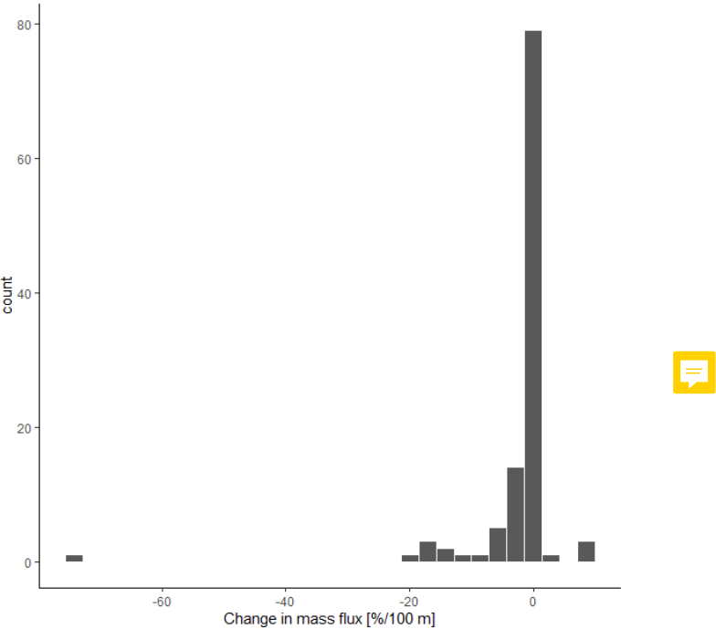
Figure 8: Loss in shell flux between the net directly below the calculated base of the productive zone and the deepest net of sampling of each station.
