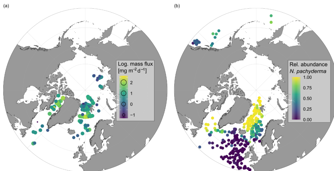
Figure 11: Regional overview on (a) logarithmic shell flux of planktonic foraminifera N. pachyderma during summer (sampling period from June to September, varies among stations) below the estimated productive zone. Fluxes were calculated based on shell abundances determined in plankton net samples. Shell weights are either from direct measurements or based on average weights from the region of sampling. (b) shows the relative abundance of the species N. pachyderma found in sediment cores (data from ForCenS data set, Siccha and Kucera, 2017).
