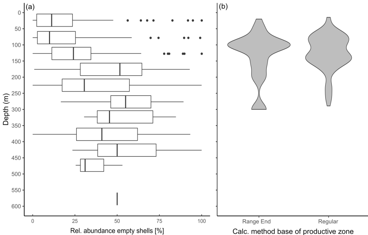
Figure 3: (a) Vertical Profile of relative abundance of empty shells at all stations of the study in which empty and filled shells were distinguished. (b) Range of the base of the productive zone (BPZ), divided by the way they were determined: “Range end” shows all samples in which the maximum depth of the net of the transition zone was defined as the BPZ, while “Regular” shows all samples in which the equation from Lončarić et al. (2006) to estimate BPZ could be applied, as described in Sect. 2.2.
