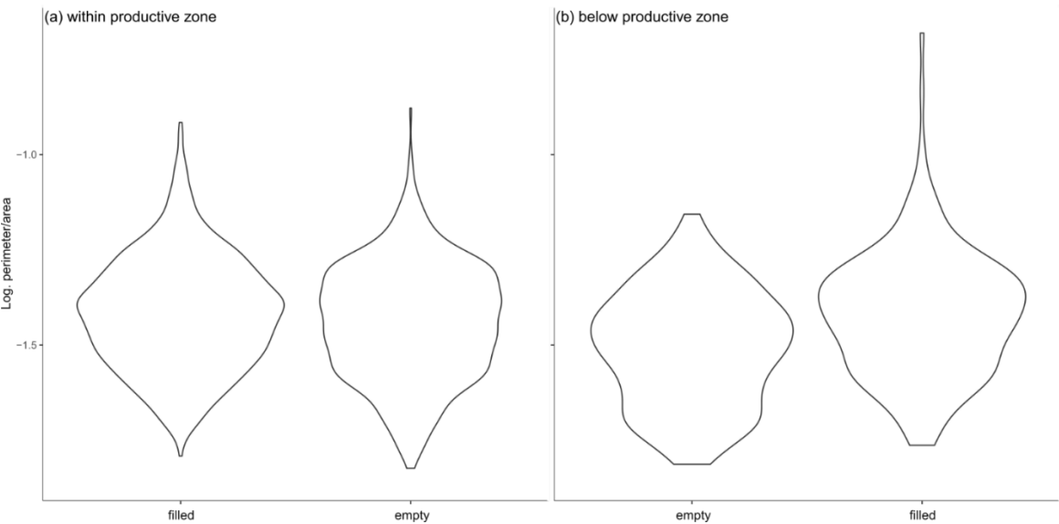
845 Figure A2: Logarithmic value of the ratio of perimeter to area in individual shells of N. pachyderma in samples from PS 93.1, divided by the status (cytoplasm-bearing and empty). (a) represents the shells from within the calculated productive zone of the individual stations, (b) those from below the productive zone.
