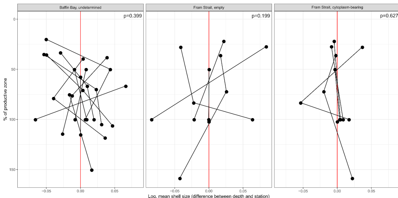
Figure 5: Logarithmic mean of shell sizes at individual stations and depths against the overall mean of each station, plotted against the percentage of the depth interval on the overall depth of the productive zone, divided into different types of shells (undetermined, empty, cytoplasm-bearing) and the two regions from which size measurements are present (Baffin Bay, Fram Strait). Consider that the samples do not represent all samples from the region shown in Fig. 1, but only those from PS93.1 (Fram Strait), MSM44 and MSM66 (Baffin Bay). The red line indicates the position at which no difference between the mean of the depth and the overall station exists. Only the depth interval within the estimated productive zone of each station is shown. p-values show the effect of increasing proportion of productive zone on shell size.
