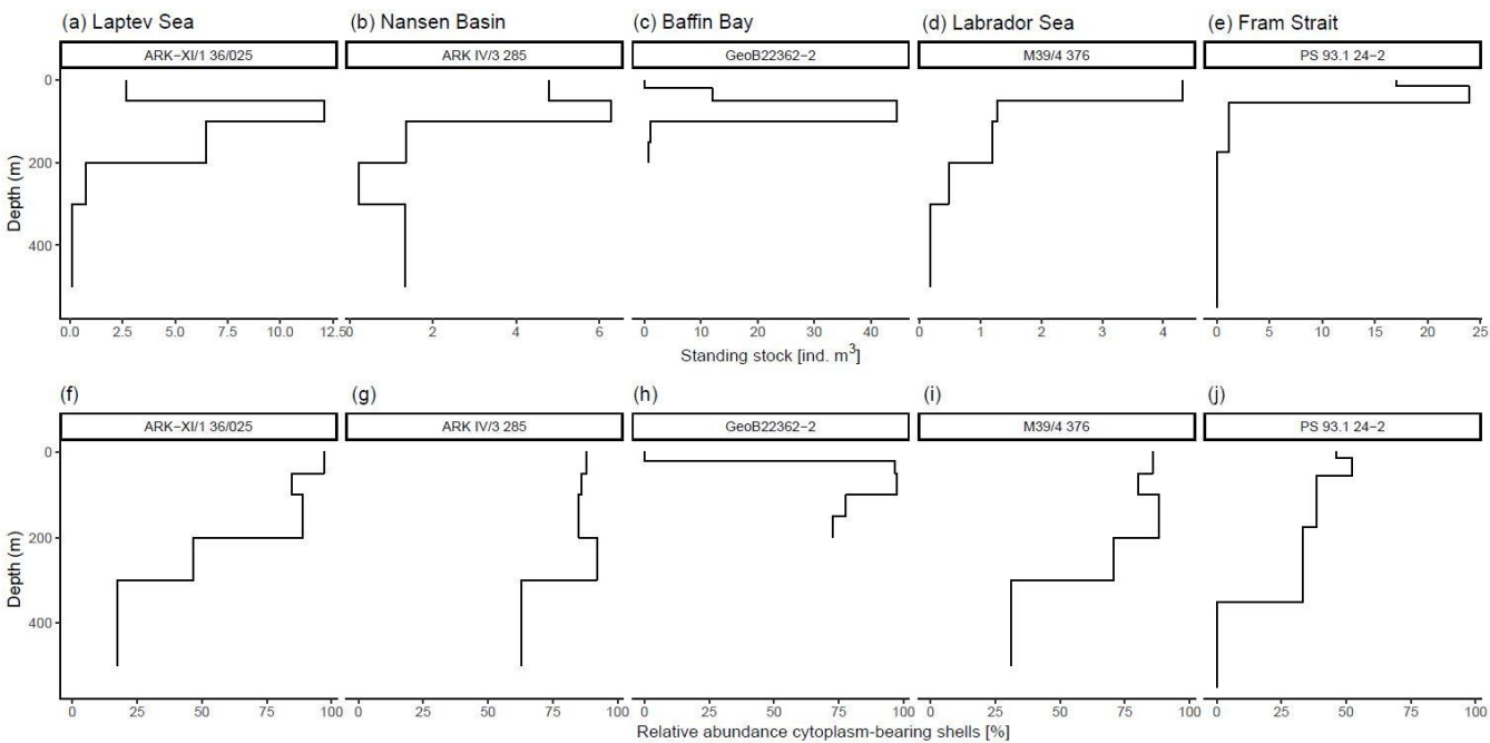
840 Figure A1: Example of vertical profiles of abundances of N. pachyderma at five different sampling locations from different parts of the Arctic Ocean. (a-e) show absolute shell concentration (ind. m -3 ) of N. pachyderma , (f-j) relative abundance of cytoplasm-bearing shells of N. pachyderma .
