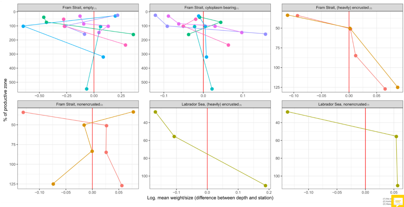
Figure 7: Logarithmic mean of the average ratio of shell weight and shell size (= calcification intensity) at individual stations and depths against the overall weighted mean of each station within the productive zone, plotted against the percentage of the depth interval on the overall depth of the productive zone. Differentiation of shell types is done between cytoplasm-bearing and empty shells from Fram Strait samples of this study (1), while Kohfeld et al. (1998) (2) and Stangeew (2001) (3) distinguished between (heavily) encrusted and non-encrusted shells in samples from the Fram Strait and the Labrador Sea. The red line indicates the position at which no difference between the mean of the depth and the overall station exists, different colours are used to make the shape of change in individual profiles visible.
